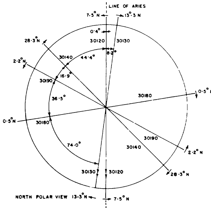
Fig. 2 : Orbits of the five operational satellites.
