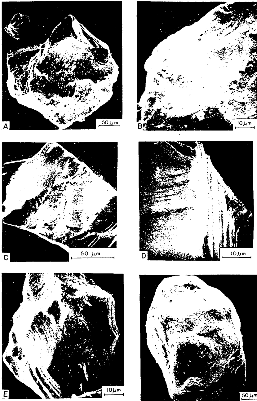
Fig. 4 : Scanning Electron Photomicrographs of quartz grains from the sediment: A – Fresh angular quartz grains with sharp edges and conchoidal fracture. B, C – Grains with irregular and varied conchoidal fracture. D, E – Sharp edge grains with thin plates. F – Conchoidal breakage pattern scattered over the surface, the edges are probably rounded by solution precipitation.
