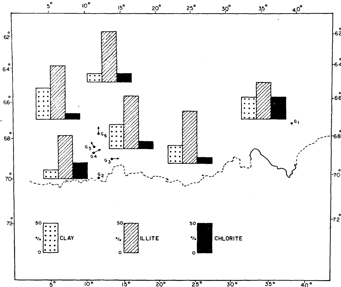
Fig. 5 : Distribution of Illite and Chlorite in clay.
