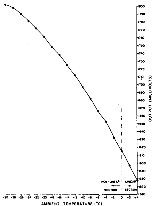
Fig. 1 : Thermistor calibration curve.
