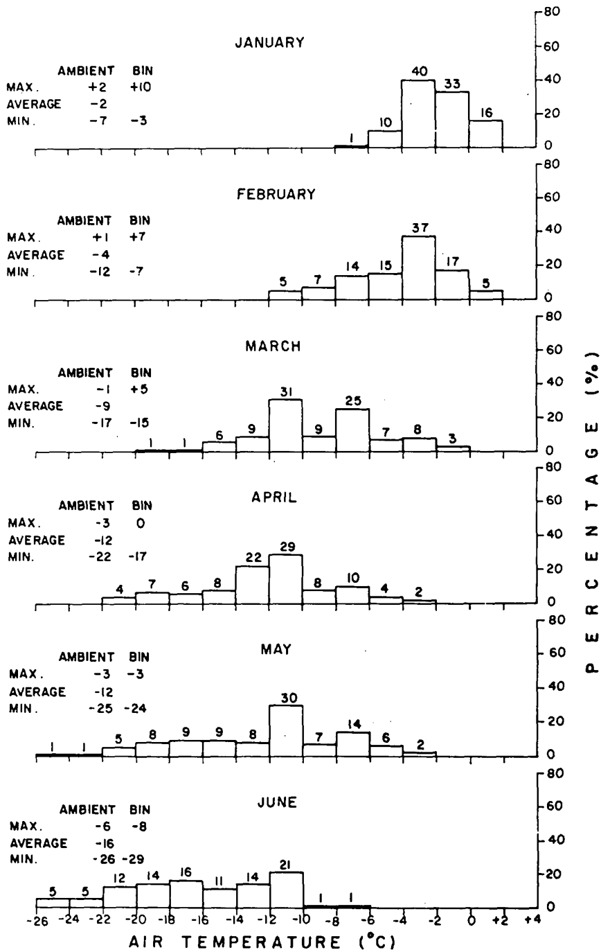
Fig. 4 : Percentage distribution of air temperature.
