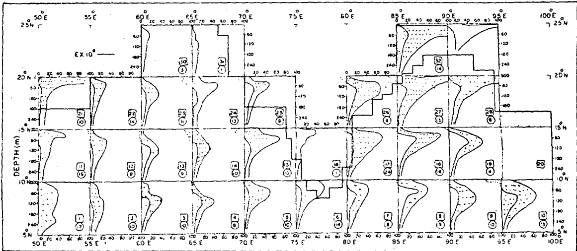
Fig. 2. Distribution of stability to the upper 300 m (June, July and August)
