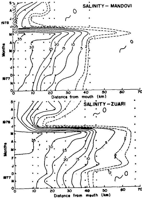
Fig. 2—Diagrammatic representation showing extent of salt water penetration from the mouth of Mandovi and Zuari rivers upstream in different months [—, salinity at 5‰ intervals; ---, salinities of 2 and 1‰]
