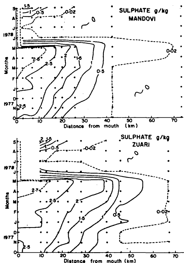
Fig. 5—Diagrammatic representation showing isolines of sulphate concentration from the mouth of Mandovi and Zuari upstream in different months [—, concentrations at 0.5 g/litre intervals; ---, at the top of the figure for Mandovi gives concentration of 2.6 g/litre and the same for Zuari gives 2.7 g/litre; ---, at the bottom in both the figures indicate concentration of 0.02 g/litre]
