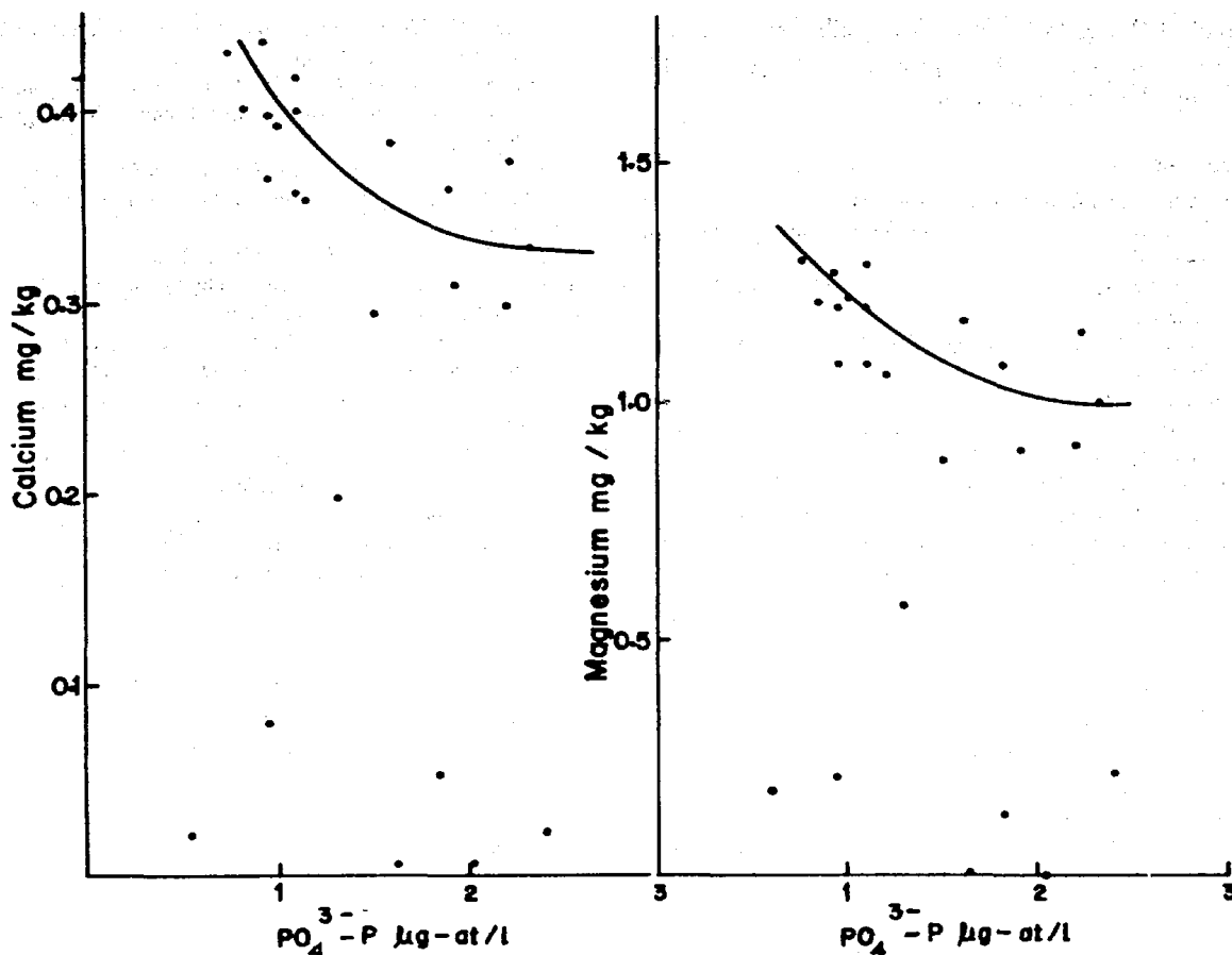
Fig. 6—Cumulative relations of calcium and magnesium with phosphate-phosphorus in both the rivers through the year [Curves have been extrapolated at higher concentrations]
