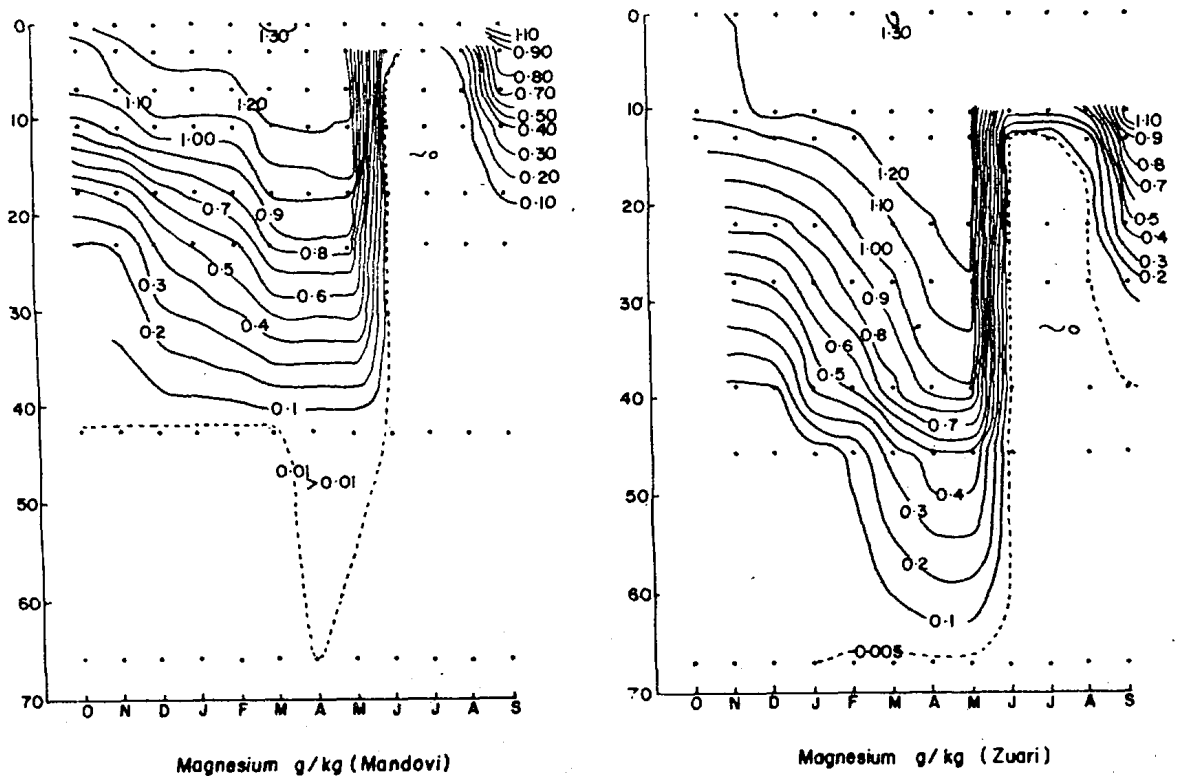
Fig. 4—Diagrammatic representation showing isolines of magnesium concentration from the mouth of Mandovi and Zuari upstream in different months [—, concentrations at 0.1 g/litre intervals, ---, concentration of 0.01 g/litre]
