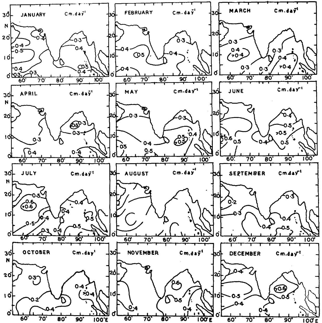
Fig. 1—Distribution of evaporation from the sea surface during different months
