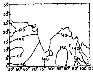
Fig. 2—Distribution of annual evaporation
