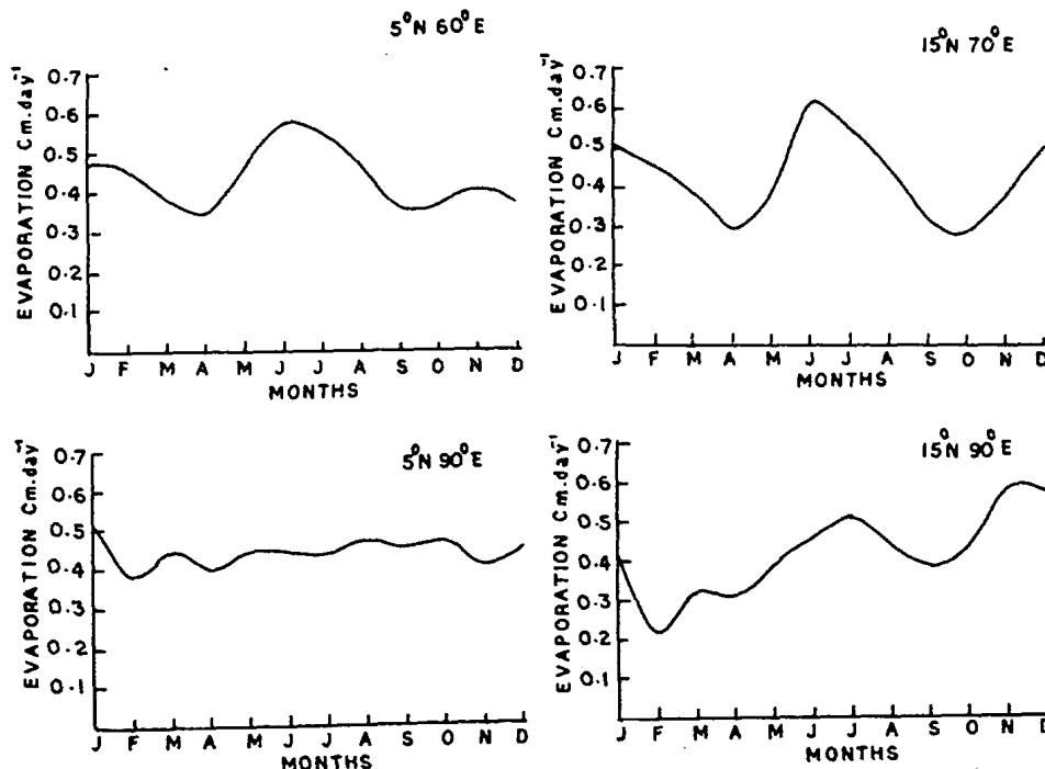
Fig. 3—Annual distribution of evaporation at 4 different stations
