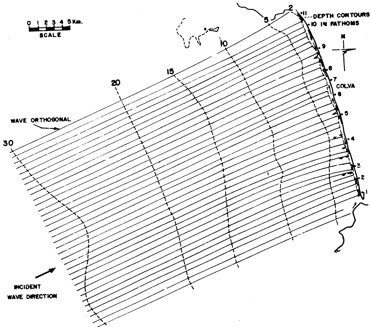
Fig. 2—Wave refraction diagram (WSW, 8 sec) for Colva area [→ Probable direction of littoral flow]
