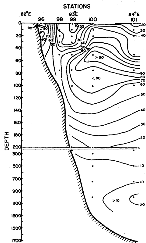
Fig. 7—Vertical per cent calcium phosphate saturation in sea water between 82-84°E long in Bay of Bengal
