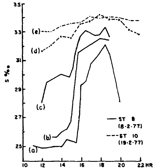
Fig. 5—Variation of salinity at sts 8 and 10 [(a) and (d) surface; (b) middle; (c) and (e) bottom]
