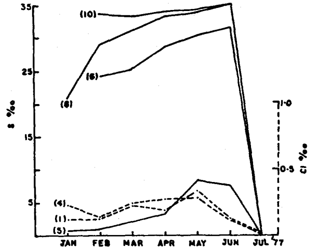
Fig. 4—Monthly salinity/chlorinity variation during flood tide at sts 1, 4, 5, 6, 8 and 10
