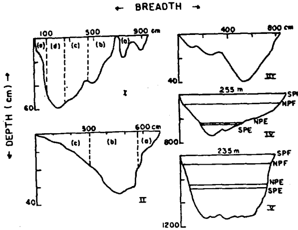
Fig. 3—Cross-sectional profiles [(I) st 1, (II) st 3, (III) st 5, (IV) st 8, (V) st 10; NP - neap, SP - spring, F - Flood, E - ebb]
