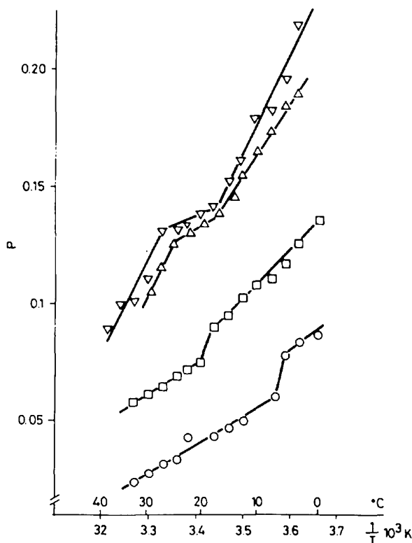
FIG. 1. Temperature dependency ( 1/T ) of DPH fluorescence polarization ( P ) in phospholipids of marine calanoid copepods. Calanus spp. were collected at Dona Paula, Goa ( \nabla ) and Bombay ( \Delta ) at the Southwest coast of India, while C. finmarchicus were collected at the West coast of Norway in the fall ( \square ) and in the spring ( \circ ), respectively.
