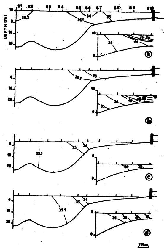
Fig.3 : Salinity distribution in the synoptic survey in October-November, 1978. a) STHW; b) NTHW; c) STLW and d) NTLW. Stations S7-S10 with different depth scale.
