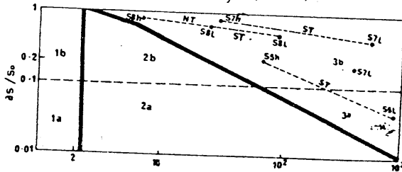
Fig.6: Stratification-circulation diagram for 3 stns. in the Morlaix estuary. H-high river discharge, L - low river discharge.
