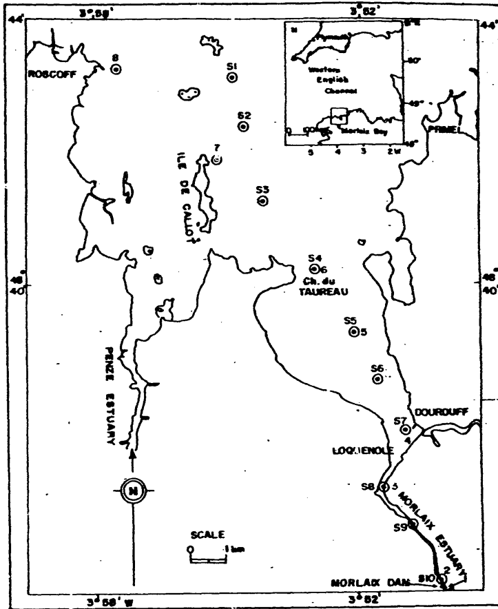
Fig.1 : Morlaix estuary showing the position of the stations in transect and synoptic surveys.
