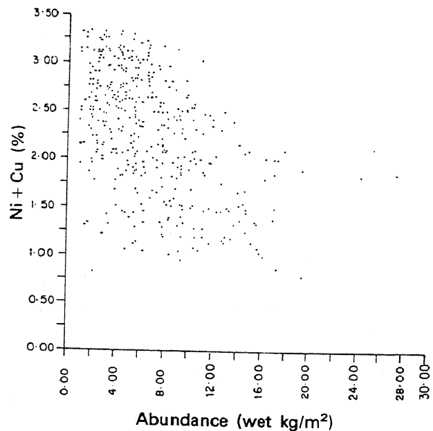
Figure 1. Scatter diagram showing the relation between abundance (wet kg/m 2 ) and grade (% Ni + %Cu) in nodules.
