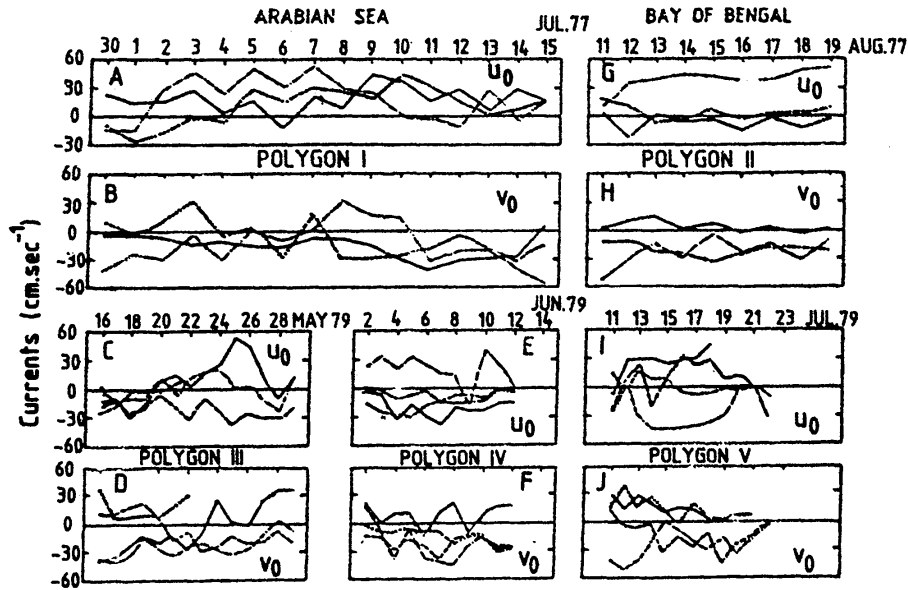
Fig. 5—Daily variation of zonal ( U_0 ) and meridional ( V_0 ) components of currents observed at 25 m in the Arabian Sea (A-F) and Bay of Bengal (G-J) [Western, —; eastern, ---; northern, ....; southern, -.-.-]
