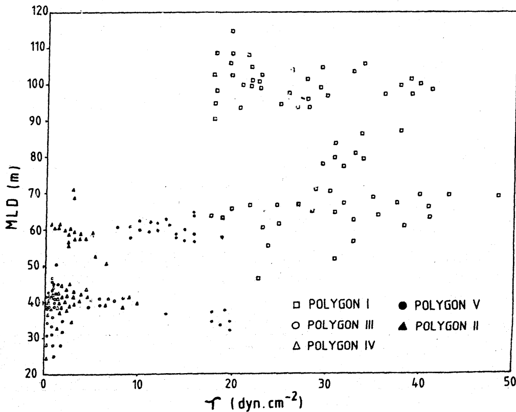
Fig. 3—Scatter diagram between MLD and \tau
