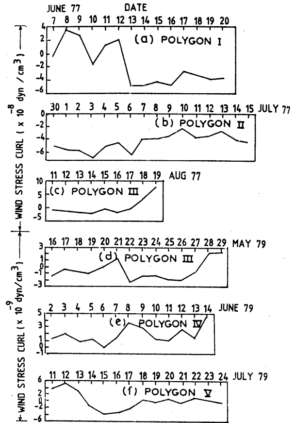
Fig. 3. Mean daily variation of wind stress curl (WSC) in all the polygon areas
