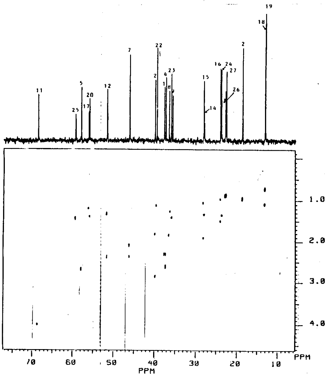
FIGURE 3. A section of the contour plot of the 2D ^1\text{H} - ^{13}\text{C} COSY spectrum of 1. The 1D ^{13}\text{C} -nmr spectrum of this section is shown above the 2D spectrum, giving their respective carbon assignments.
