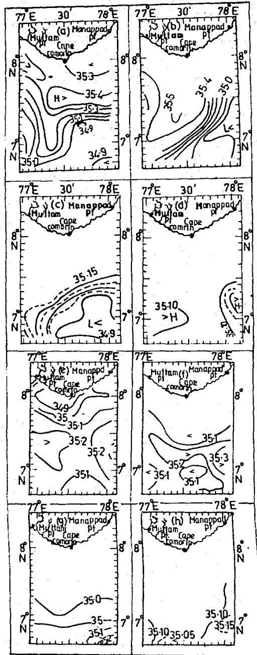
Fig. 2. Salinity ( \times 10^{-3} ) distribution at (a) surface, (b) 50, (c) 100 and (d) 500 m depths during May and at (e) surface, (f) 50, (g) 100 and (h) 500 m depths during September.
