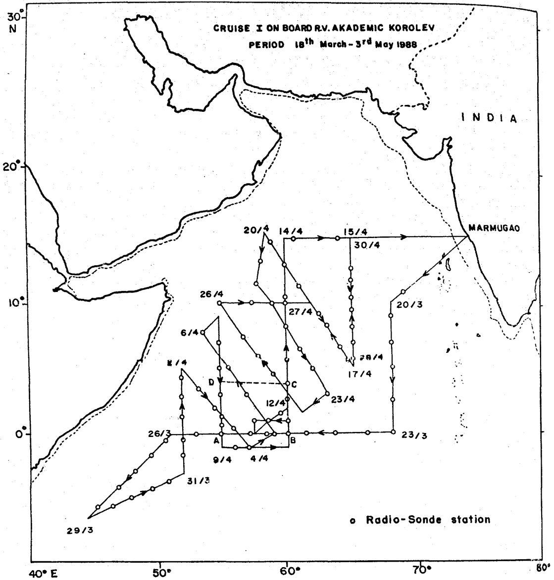
Fig. 1. Cruise track together with the radiosonde stations during the pre-monsoon period (MONSOON-88 Expedition). The data in the area ABCD which was covered repeatedly was used for the computations of heat and moisture budgets.
