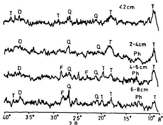
Fig. 2—X-ray diffractograms of different size nodules. (T = todorokite, D = \delta -MnO 2 , Q = quartz, Ph = phillipsite and F = feldspar)
