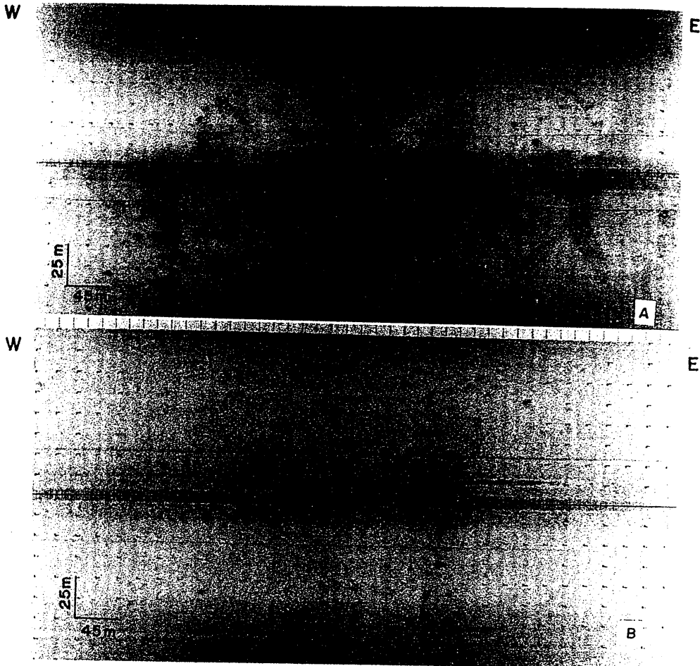
Figure 7. Sonographs showing spot phenomenon produced by algal knolls. (A) Algal knolls are densely distributed in the north; and (B) less towards the south.
