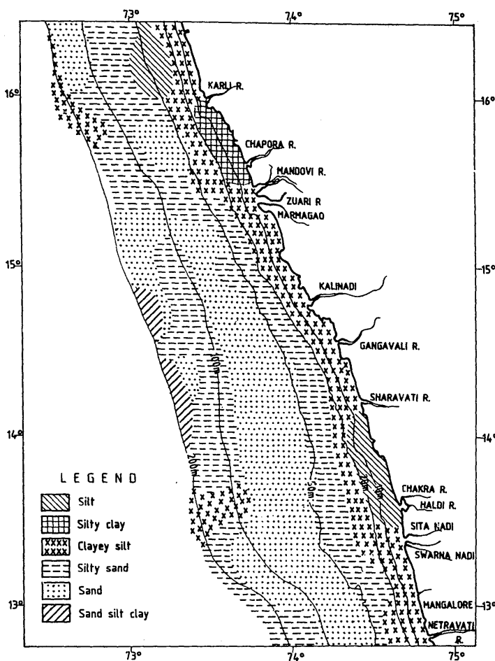
Figure 2. Map showing surface sediment distribution on the central western continental shelf of India (after Nair et al. , 1978).
