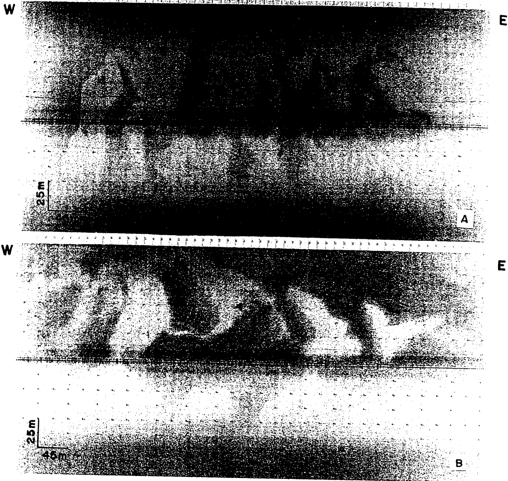
Figure 5. Sonographs showing tonal patches produced by textural differences in the sediments. Dark patches are the reflections from coarse grained sediments. (A) Abundance of the patches is less towards the inner shelf, and (B) more towards the outer shelf.
