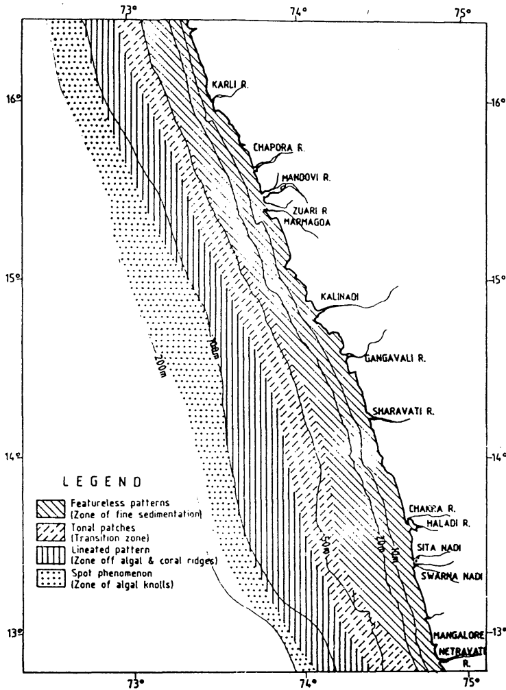
Figure 9. Schematic diagram showing sonograph facies distribution on the central part of the western continental shelf of India.
