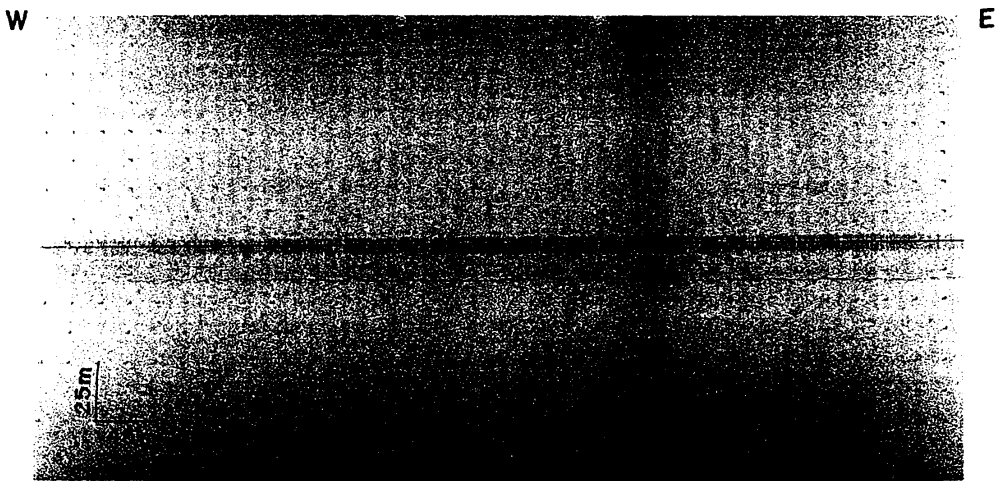
Figure 3. Sonograph showing featureless pattern due to the smooth topography on the inner shelf which is covered with fine grained sediments.
