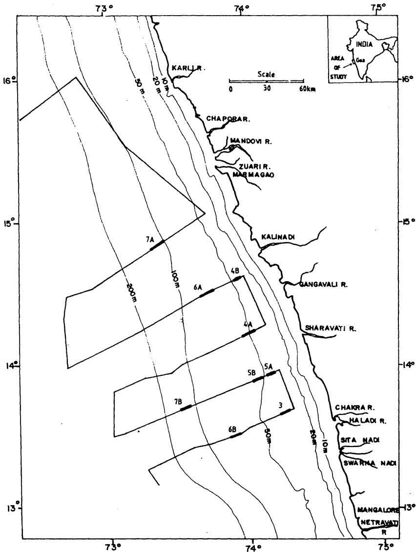
Figure 1. Map of the central western continental shelf of India showing side scan sonar tracks. Numbers on the track lines indicate the locations of sonographs shown in Figures 3-7.
