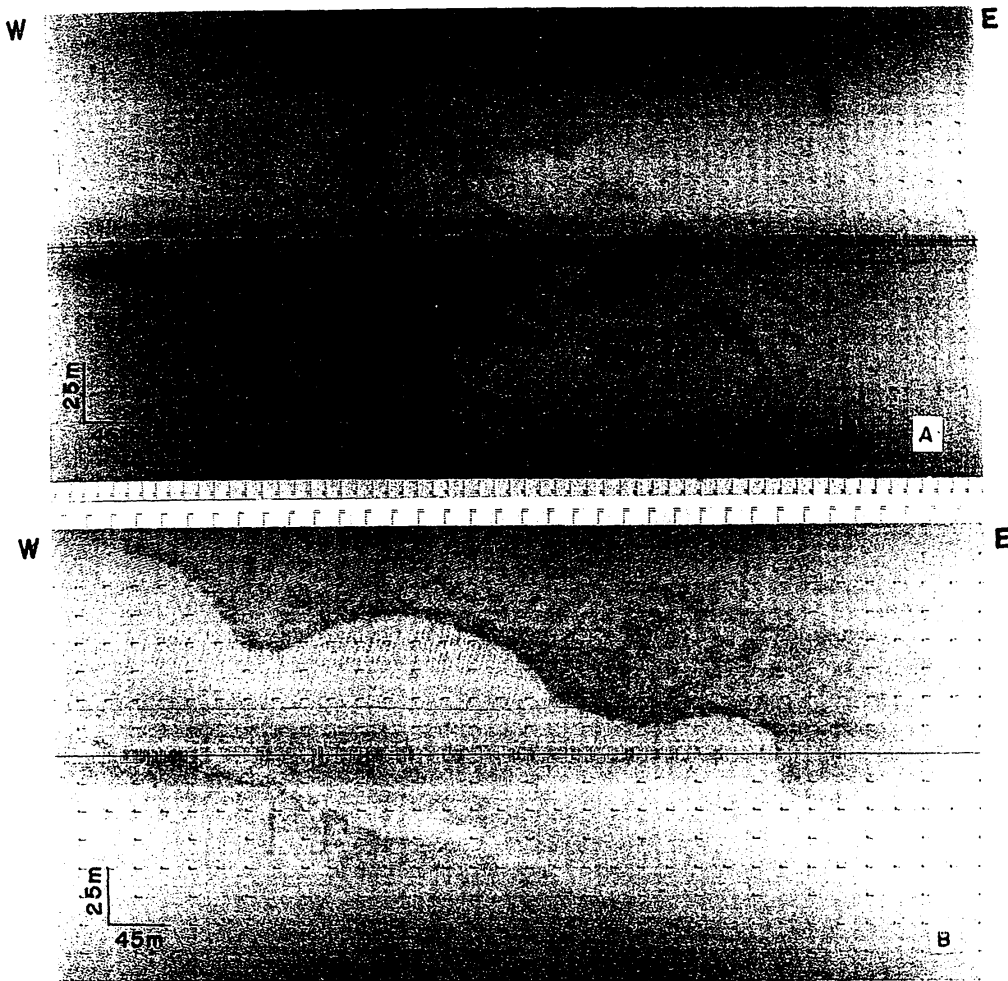
Figure 4. Sonographs showing (A) light tone towards the inner shelf and moderate tone towards the outer shelf; and (B) distinct tonal difference reflecting variations in the surface sediments ( i.e. coarse—dark tone, finer—light tone).
