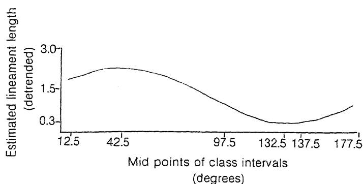
Figure 3. Cosine wave curve obtained from data for lineaments of Goa.
