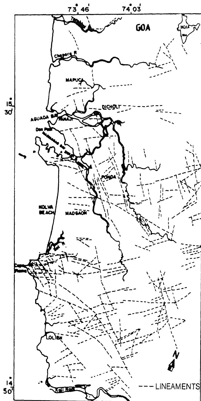
Figure 1. Lineament map of Goa.
