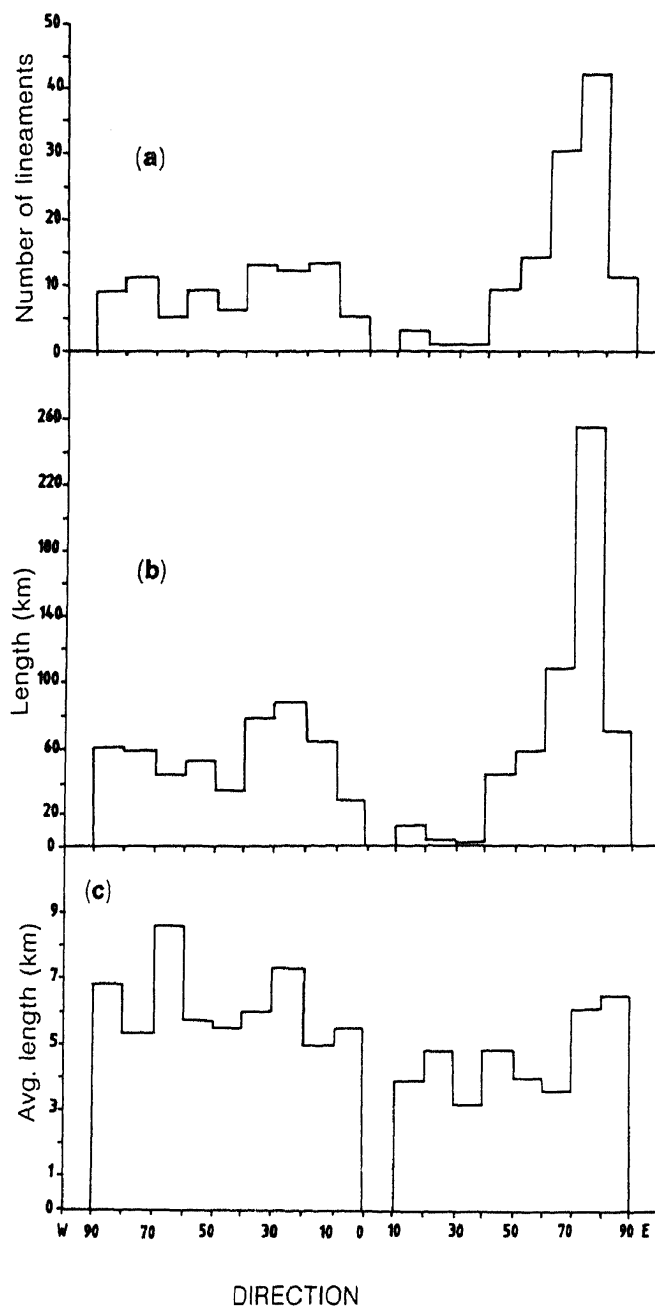
Figure 2. Histograms: (a) number of lineaments in 10° direction intervals, (b) total length of lineaments, and (c) average length of lineaments.
