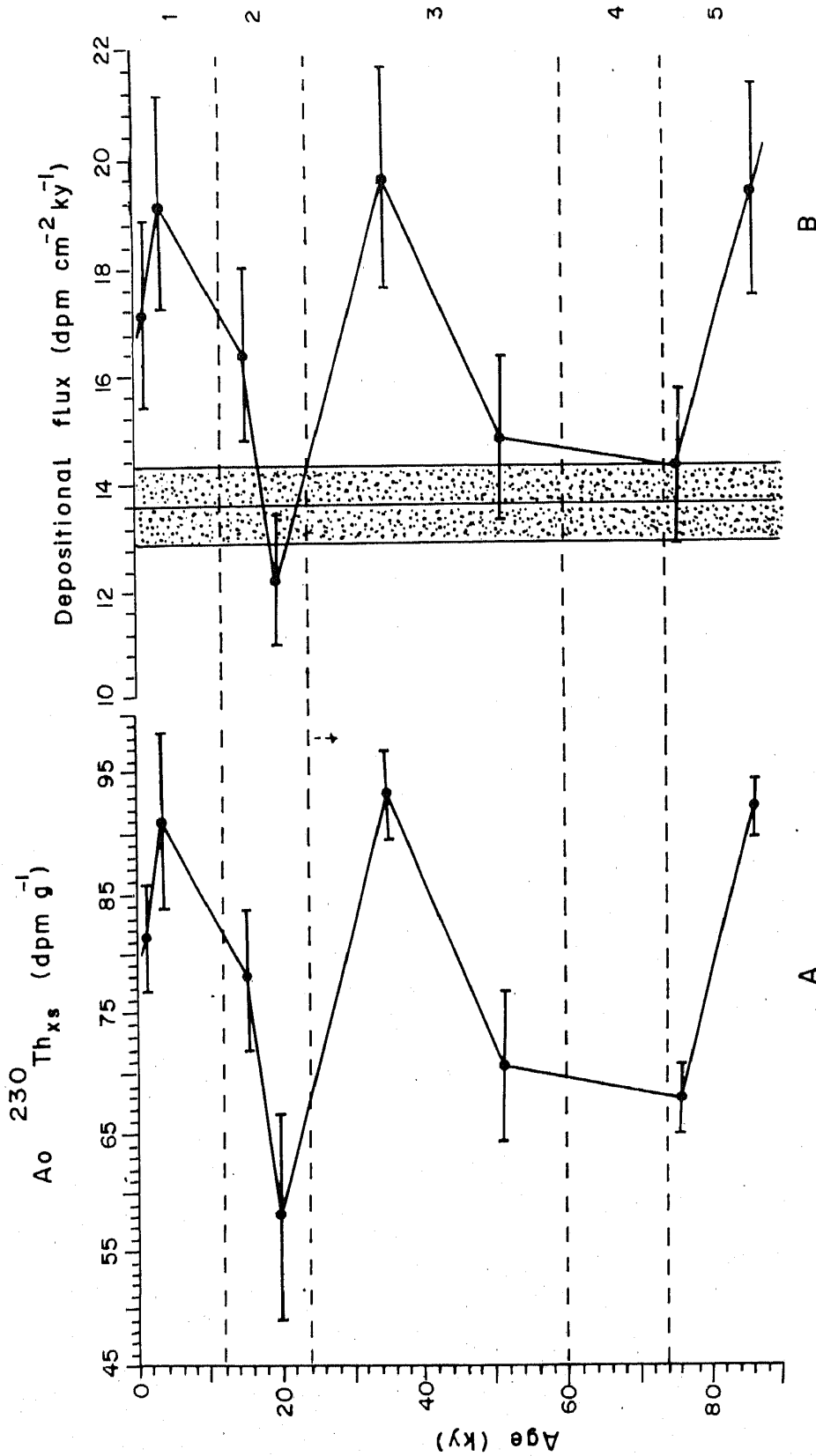
Figure 1(A). Distribution of A_0^{230}\text{Th}_{xs} with time in \text{dpm g}^{-1} . The numbers 1, 2, 3, 4 and 5 are the tentative oxygen isotope stages identified by comparing the U/Th ages with the oxygen isotope stratigraphy of Martinson et al (1987)(B). Depositional flux of ^{230}\text{Th}_{xs} with time. The dotted area represents the present day expected flux of 13.6 \pm 0.7 \text{ dpm cm}^{-2} \text{ky}^{-1} .
