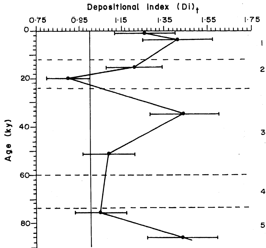
Figure 2. Age profiles of depositional index (Di). The solid line ( Di = 1 ) shows the flux expected under steady state condition. Values < 1 indicate removal of Th while > 1 reflect supply of Th by lateral transport.
