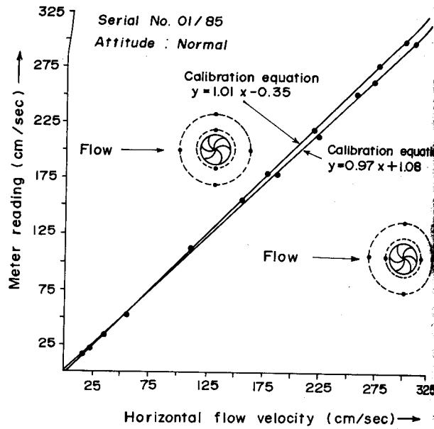
FIG. 7. Calibration limits in orthogonal flow orientations of the meter shown in Fig. 1a.
