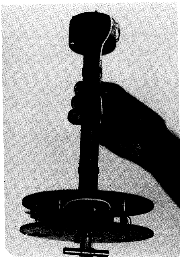
FIG. 2. (a) Open wedge-shaped miniature free vane used in the flowmeter of Fig. 1a. (b) Magnetic compass (top) and cylindrical bar magnet (bottom) rigidly mounted on the stud of a precision circular potentiometer (located between two circular plates), which magnetically couples to the free vane in panel (a).
