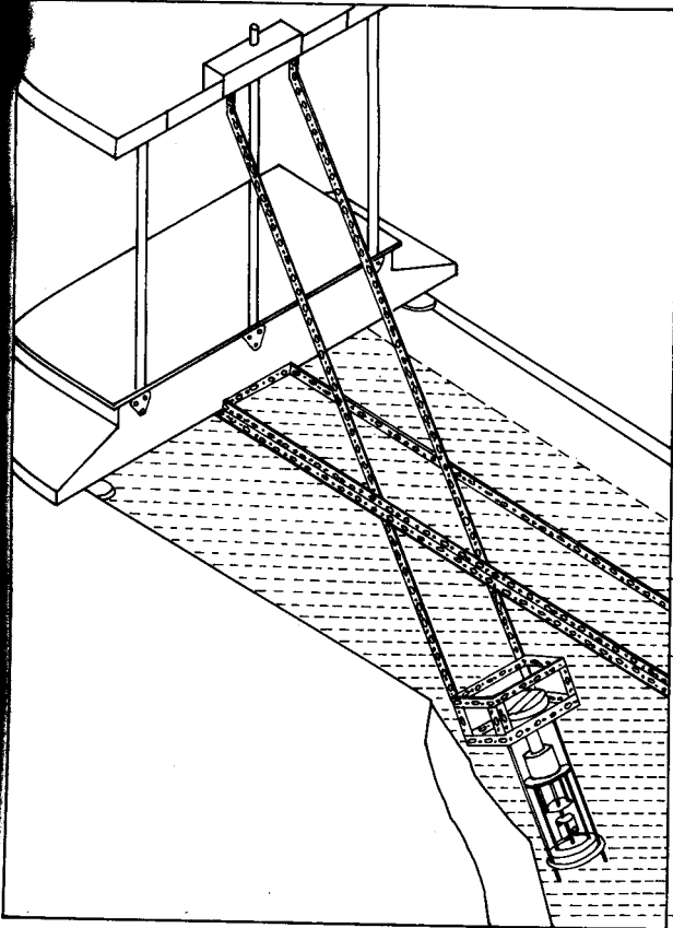
FIG. 8. Experimental setup for investigation of tilt response. In this figure, a meter shown in Fig. 1a is seen attached to the tilting mechanism.
