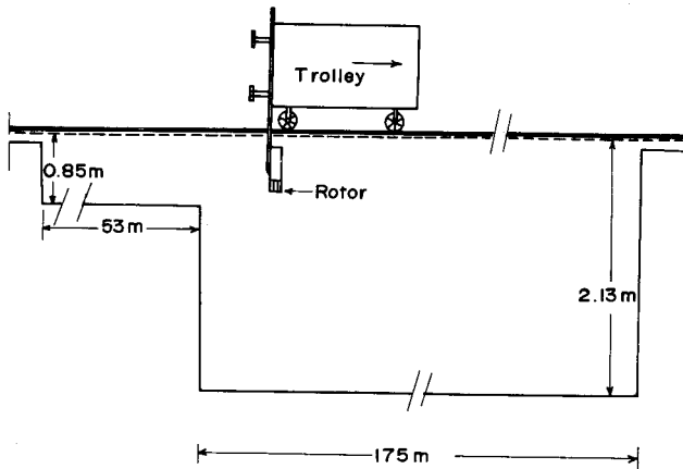
FIG. 3. Tow tank and trolley facility used for conducting flow evaluation experiments on flowmeters.
