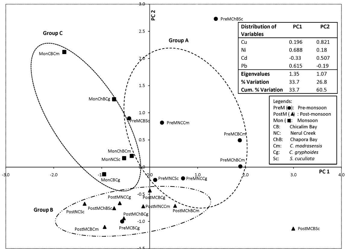
Fig. 2 The scatterplot of PCA scores (PC1 vs. PC2) of samples analyzed for metal concentrations in oyster species in three different seasons from selected sites
