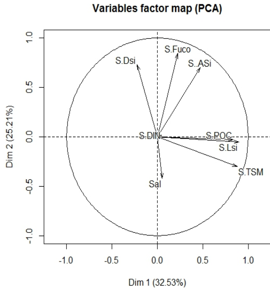
Fig. B1: PCA analysis on upper estuaries during dry period.
