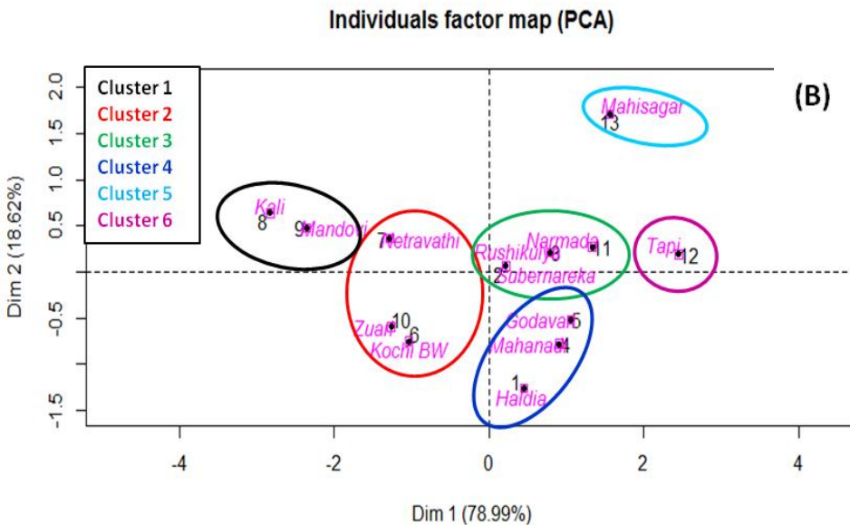
Fig. 6a and b , PCA analysis on the impact of land use in the Indian estuaries during the wet period. A) Relationship among the variables and b) Individual factor map and clustering with Indian estuaries based on PCA results.
