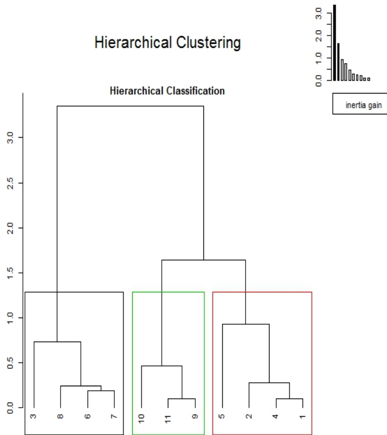
Fig.B7: Hierarchical clustering of PCA results on lower estuaries during wet period.
