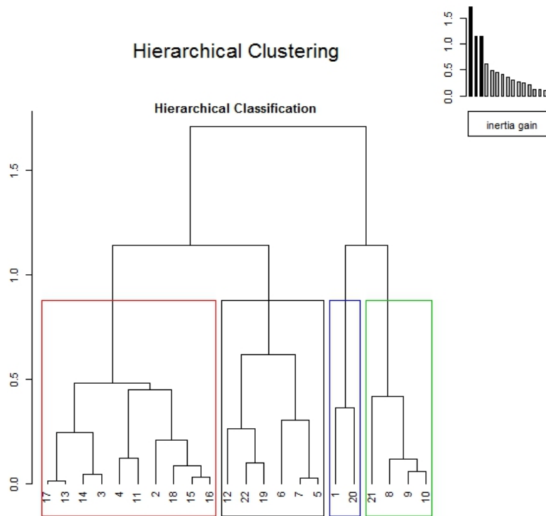
Fig. B2 Hierarchical clustering of PCA results on upper estuaries during dry period.
