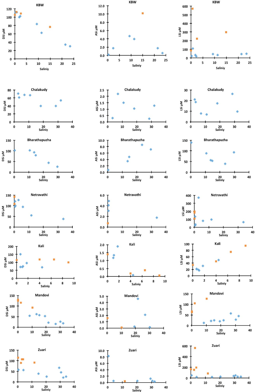
Fig. A3 DSi, ASi and LSi vs. salinity for southwest estuaries (wet season: orange squares, dry season: blue diamonds).
