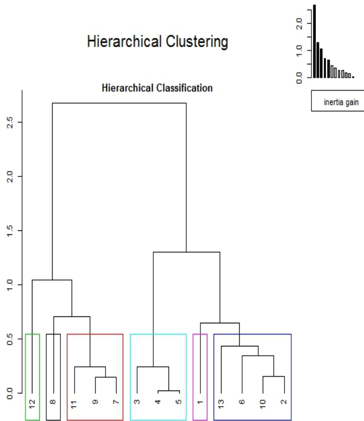
Fig. B5: Hierarchical clustering of PCA results on upper estuaries during wet period.
