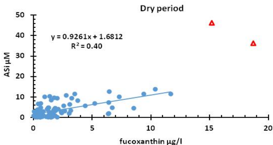
Fig. 2 Best linear fit of ASi vs. fucoxanthin, to calculate the missing ASi. Two outliers (red triangles) from the small estuary Ponnaiyar (SE estuary) are excluded from the regression due to their very high ASi concentrations. Note that the regression line equation is used to recalculate the missing and negative ASi concentrations of the dry season for the PCA (see text).
