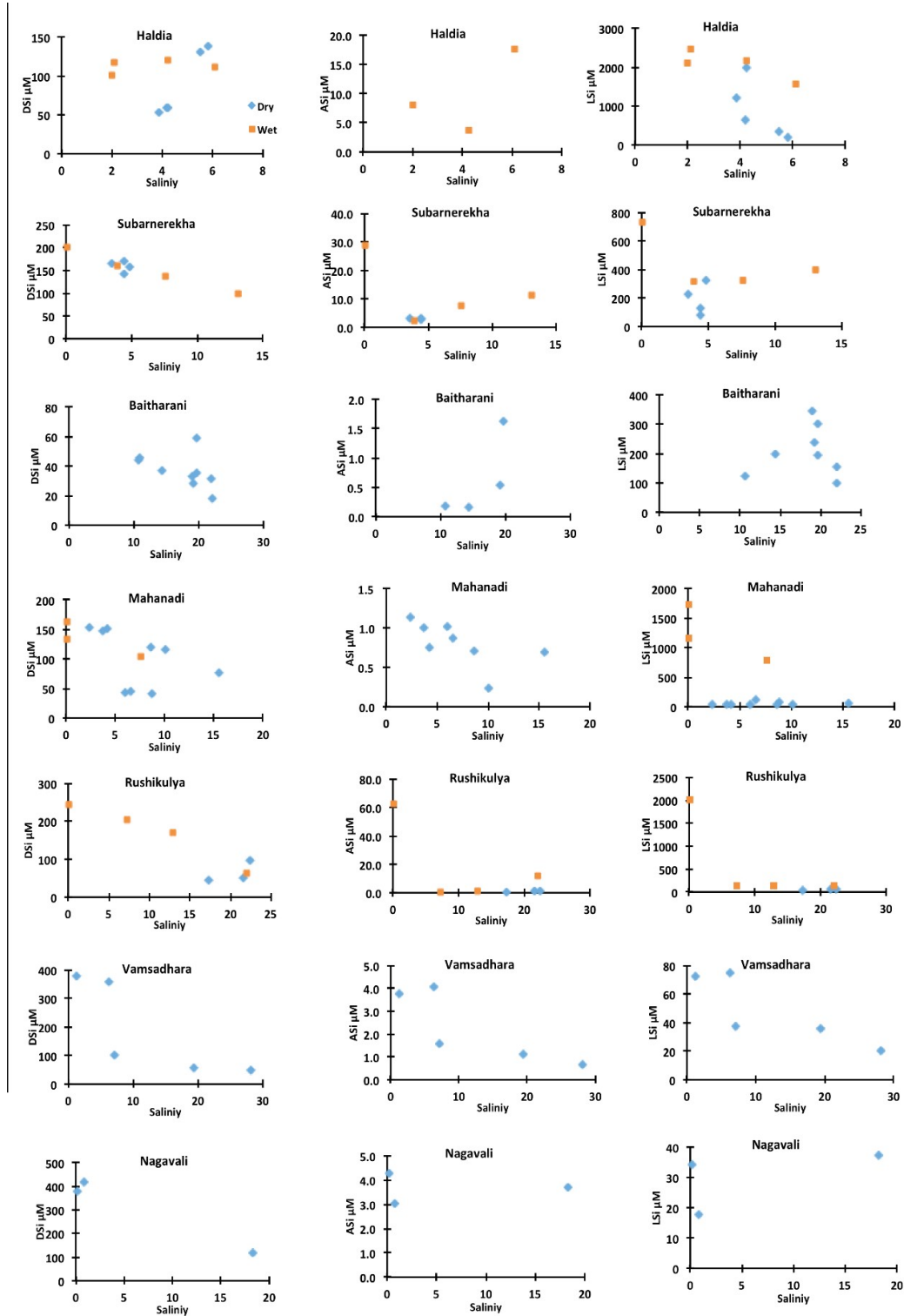
Fig. A1 DSI, ASI and LSI vs. salinity for northeast estuaries (wet season: orange squares, dry season: blue diamonds).
