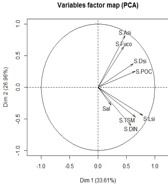
Fig. B3: PCA analysis on lower estuaries during dry period.
