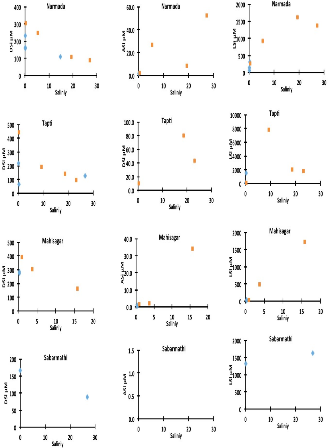
Fig. A4 DSi, ASi and LSi vs. salinity for northwest estuaries (wet season: orange squares, dry season: blue diamonds).
