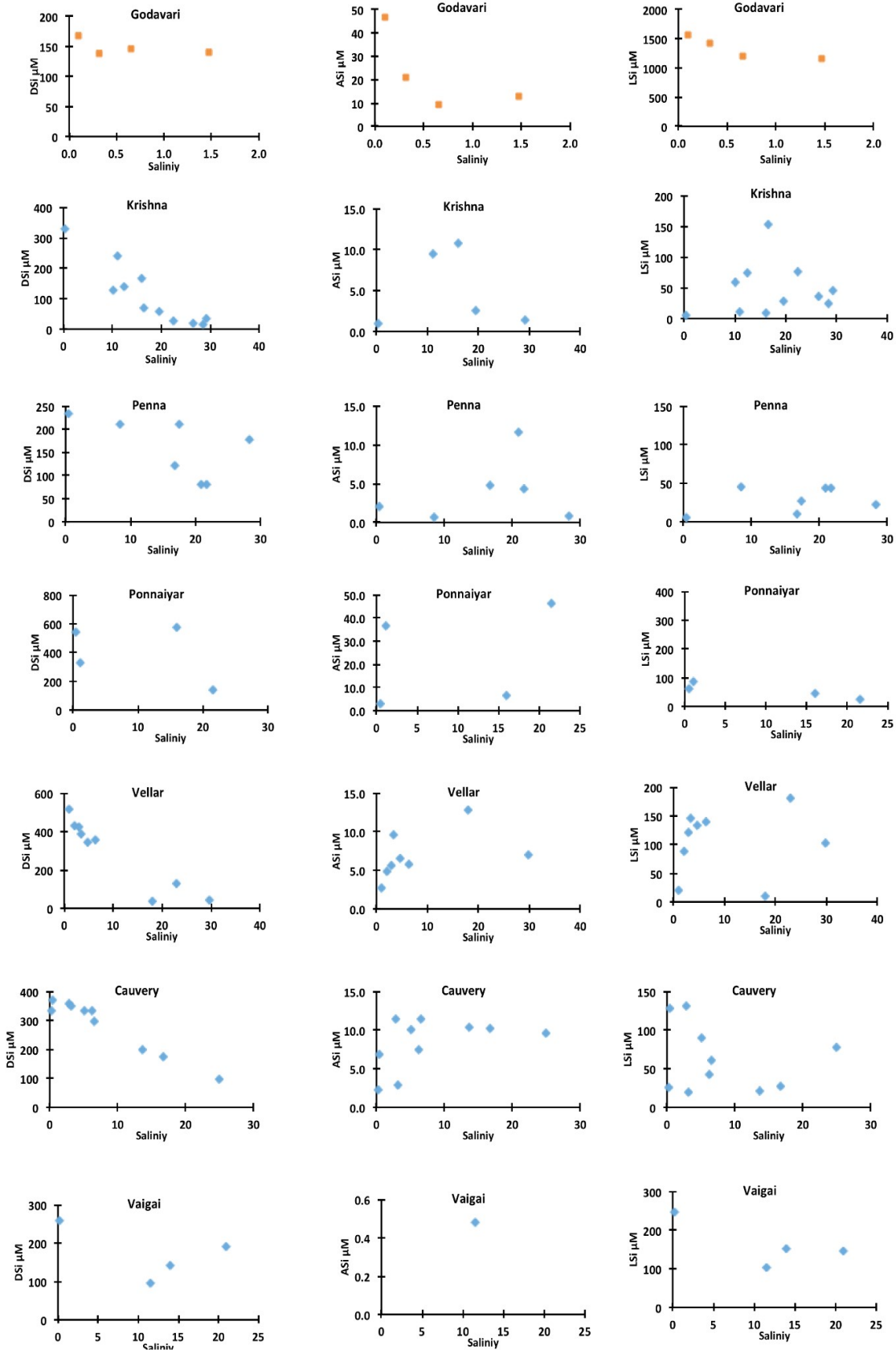
Fig. A2 DSi, ASi and LSi vs. salinity for southeast estuaries (wet season: orange squares, dry season: blue diamonds).
