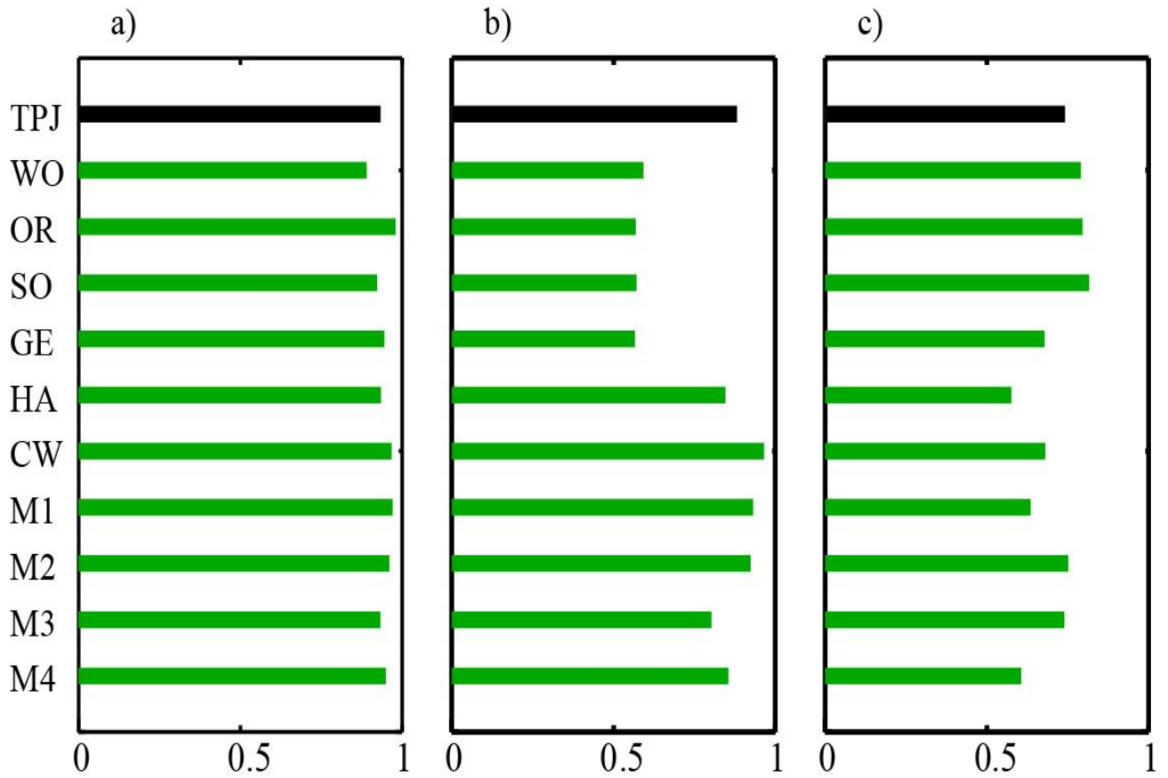
Figure S8: Complement to fig. 4: pattern correlation between SLA pattern from individual products and pattern shown in panels a, b, c of figure 4.
