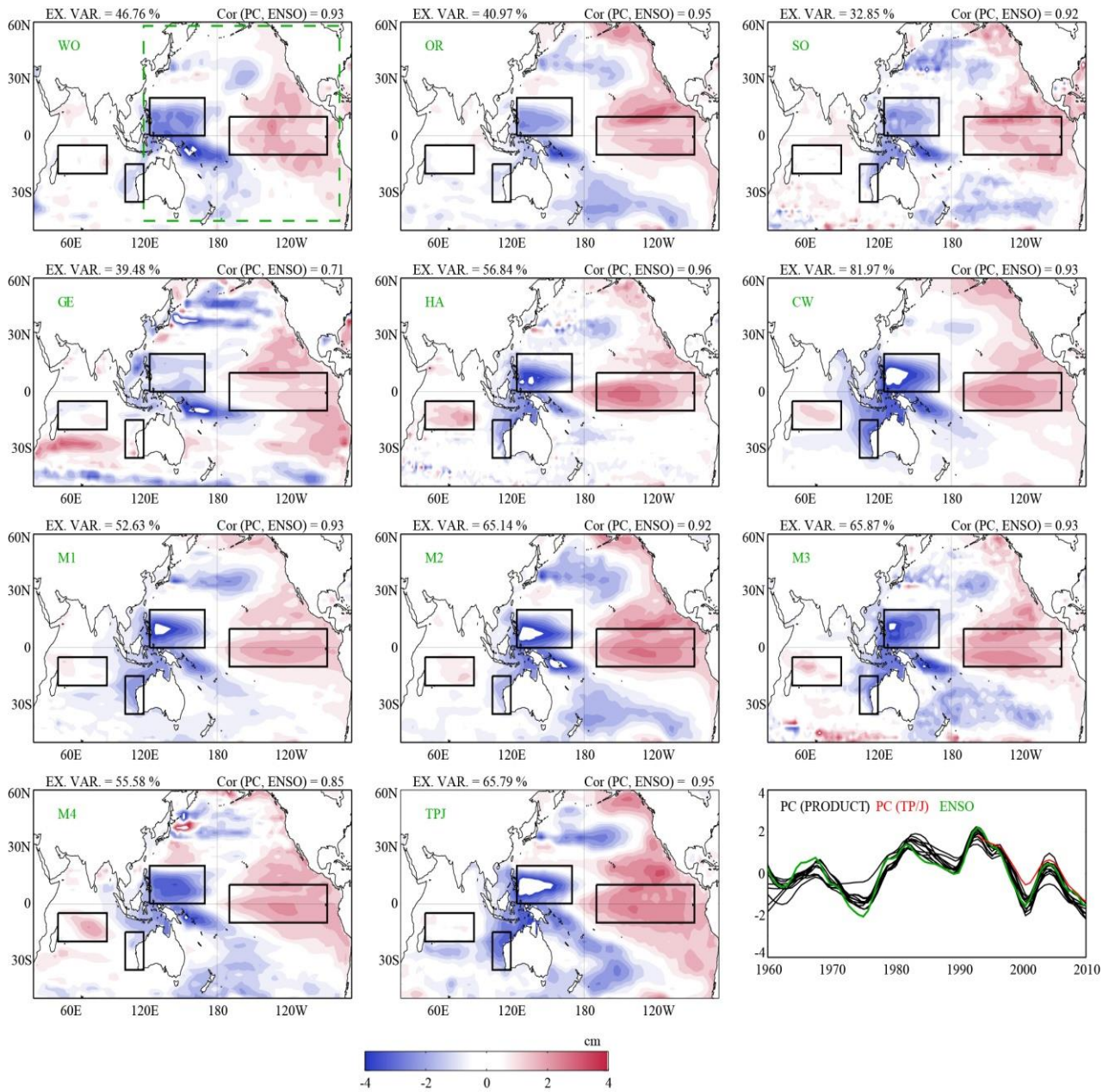
Figure S4: Indo-Pacific SLA signature of Pacific decadal SLA EOF1 (spatial maps) from 10 sea-level data used in this study and for the shorter merged altimetric dataset.. PC1 from 10 products (black) and TPJ (red) are shown in the last panel with decadal ENSO time series (green).
