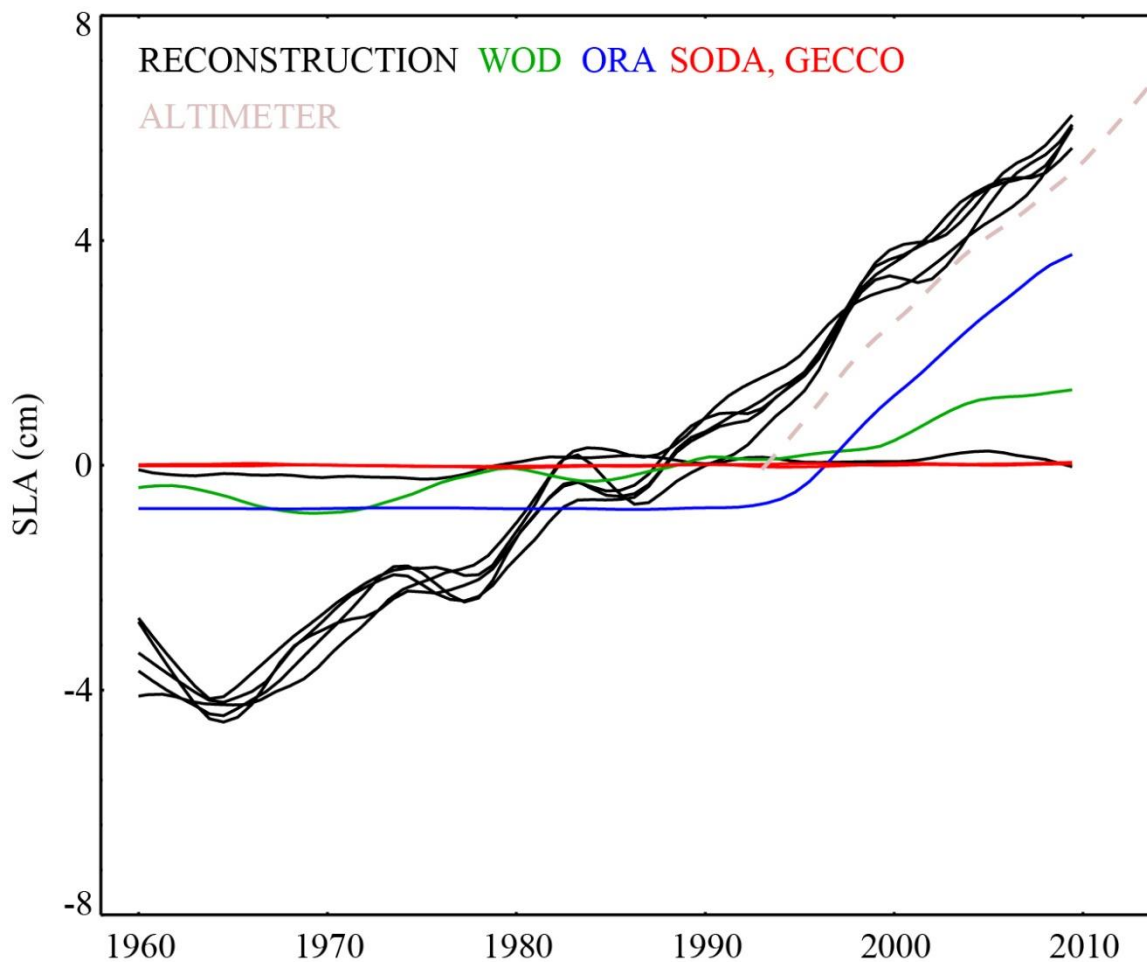
Figure S1: Global mean sea level (GMSL) time series from 11 gridded products (including Altimetry - TPJ) analysed in this study: WO (green), OR (blue), SO & GE (red), HA, CW, M1, M2, M3, M4 (black) and TP/J (light red). This GMSL is obtained as the spatial average over the 65°N-65°S latitudinal band of the decadal sea-level component of each gridded product
