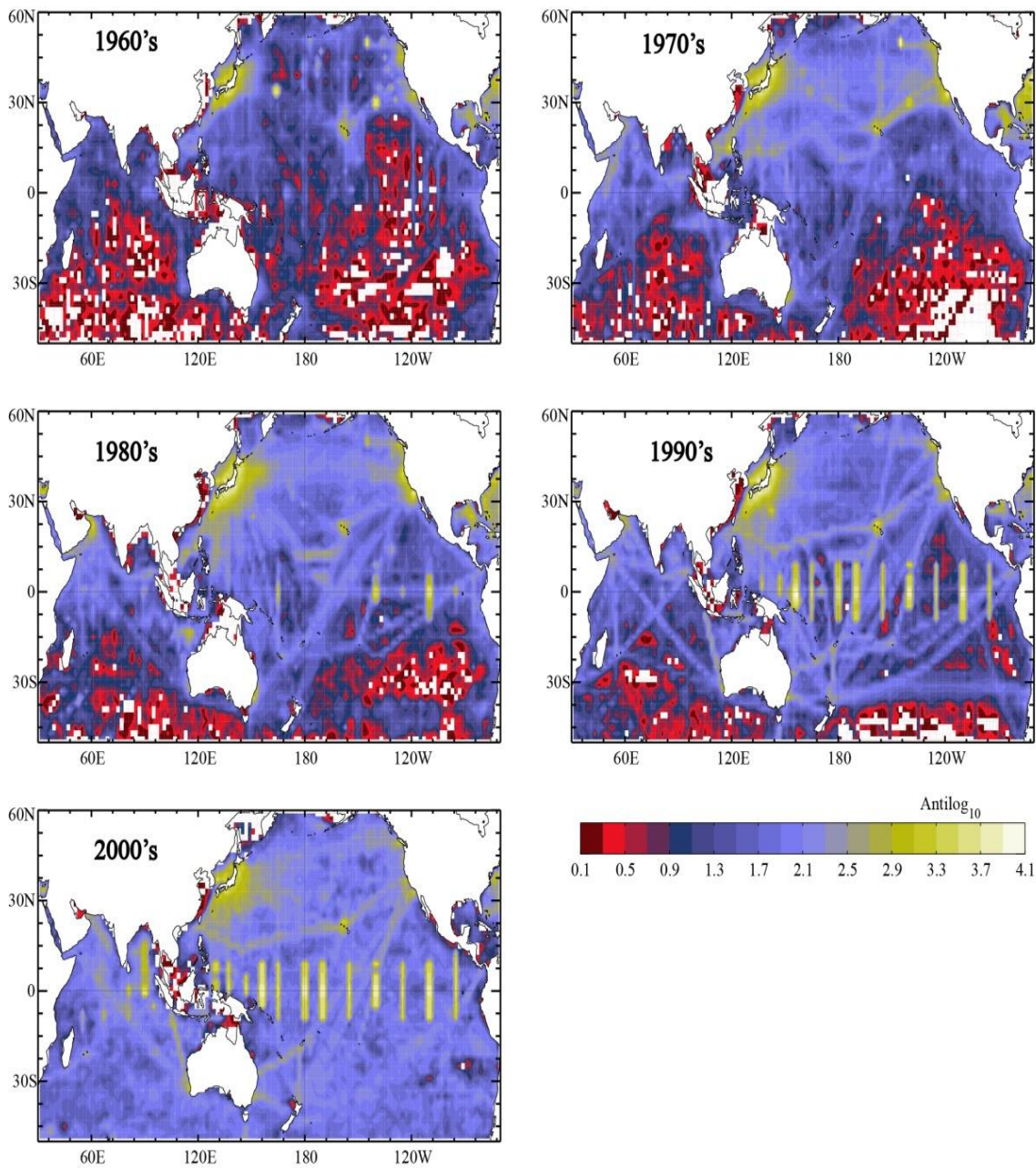
Figure S9: Decimal logarithm of the number of profiles per 2^\circ \times 2^\circ box and per decade, with enough levels to estimate the heat content of the top 300 meters of the Indo-Pacific Ocean (i.e. that resolve vertical movements of the thermocline associated with natural decadal climate variability), during 1960-2010.
