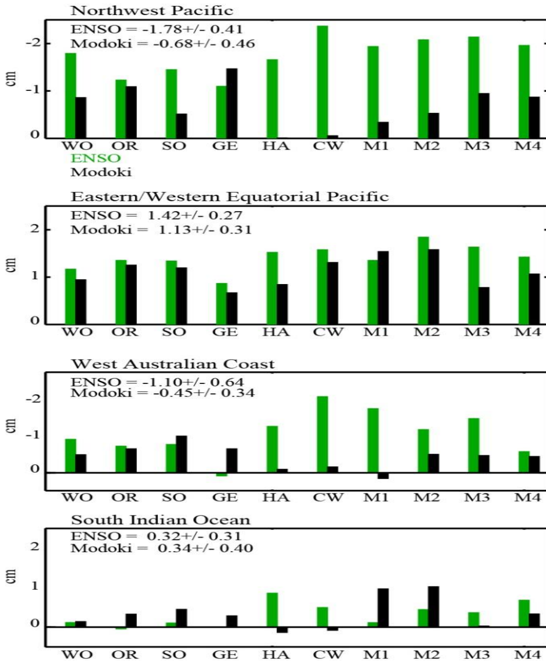
Figure S6: Decadal ENSO- (green) and Modoki- (black) related SLA amplitude at four regions shown in SI4 and SI5 (four boxes), computed as the box-averaged value of EOF from each product. The mean amplitude and its inter-product standard deviation are also given on each panel for both ENSO and Modoki. Note that in S4 and S5, the regions selected to highlight equatorial Pacific variability for ENSO and Modoki are different (eastern equatorial Pacific for ENSO and western equatorial Pacific for Modoki) based on their maximum centers of action.
