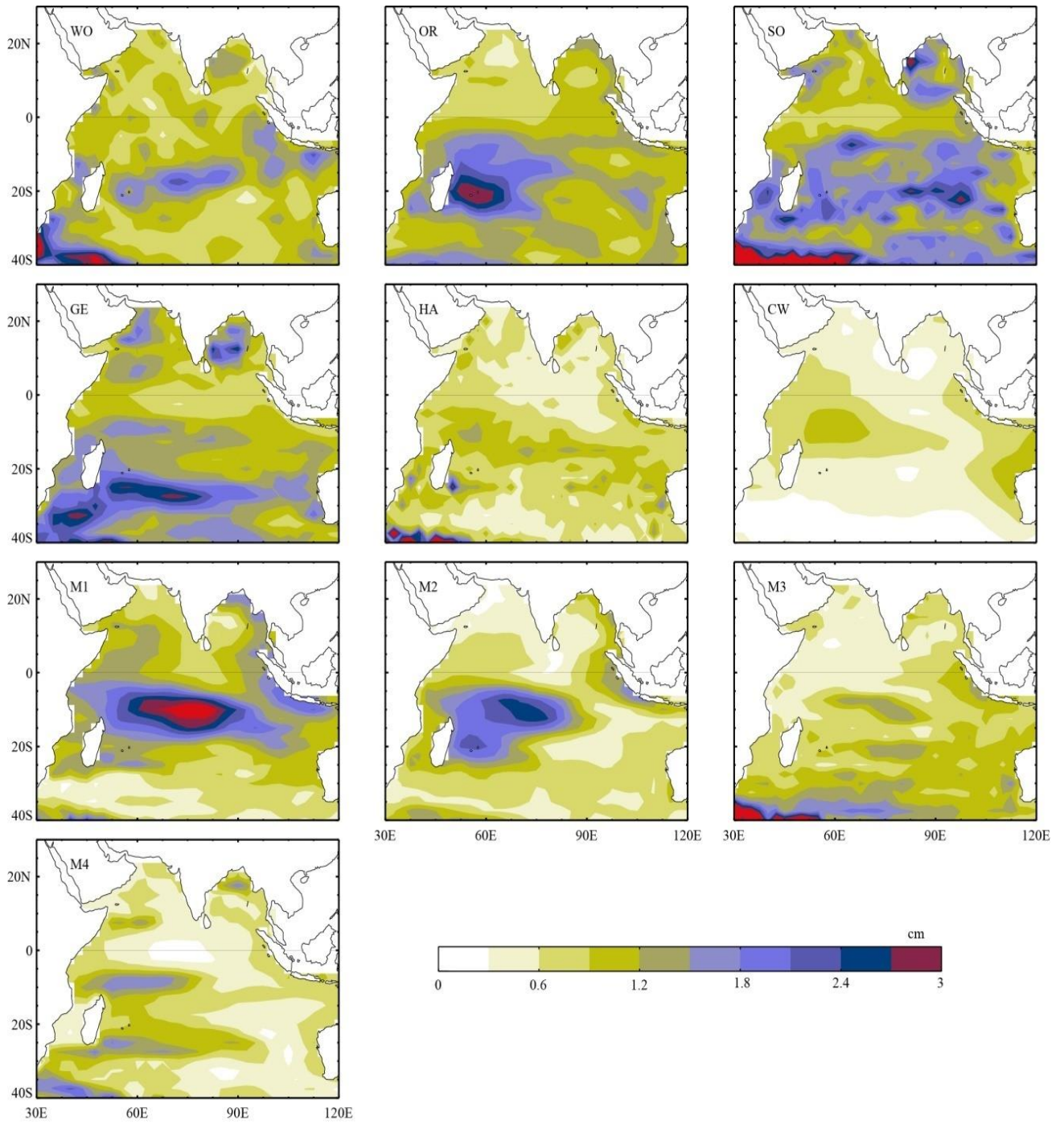
Figure S7: Standard deviation of Pacific-independent decadal SLA in the IO from individual products.
