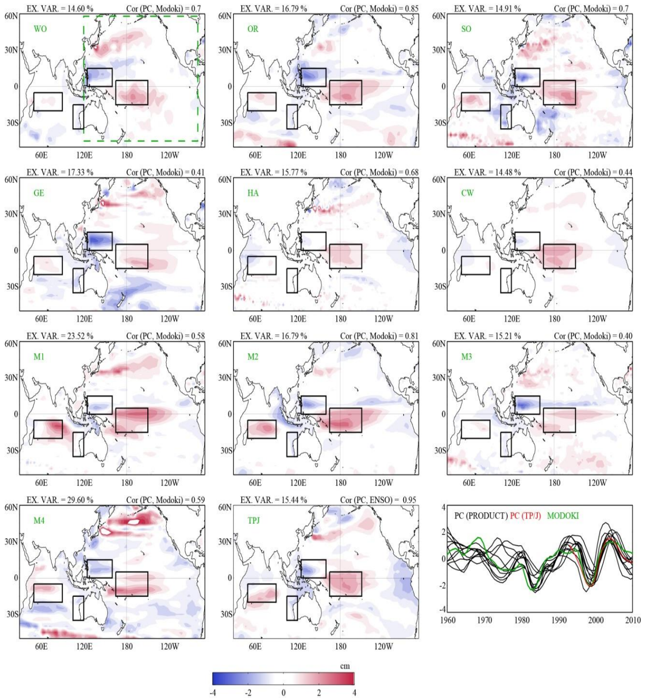
Figure S5: As Figure S4, but for Indo-Pacific SLA signature of Pacific decadal SLA EOF2. In the last panel, decadal MODOKI time series (green) is shown with sea-level PCs.
