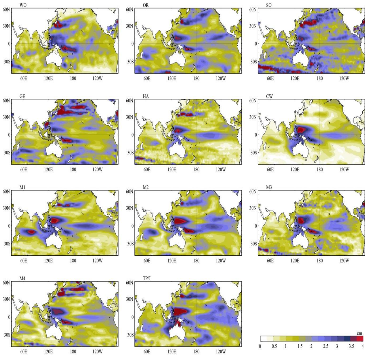
Figure S3: Standard deviation of decadal SLA from the 10 gridded products analyzed in this study and for the shorter merged altimetric dataset.
