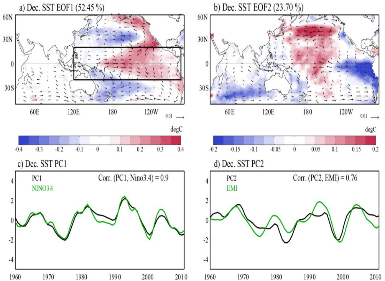
Figure S2: First two EOFs of decadal SST variability in the tropical Pacific (120°E-70°W, 20°S-20°N; black rectangle on panel a) over the 1960-2010 period. (a, b) SST (color) and wind-stress (arrow) patterns associated with EOF1 and EOF2. (c, d) Corresponding principal components (PCs). Decadal components of Niño3.4 SST index and EMI (El Niño Modoki Index; Ashok et al. 2007) are overlaid on panels c and d respectively with corresponding correlation coefficient. Even though the EOFs are computed for the tropical Pacific, the SST and wind are regressed onto the corresponding normalized PCs over the entire Indo-Pacific region to assess their Indo-Pacific signature. PCs shown in panels c and d are used in this study as indices for decadal ENSO and Modoki variability respectively.
