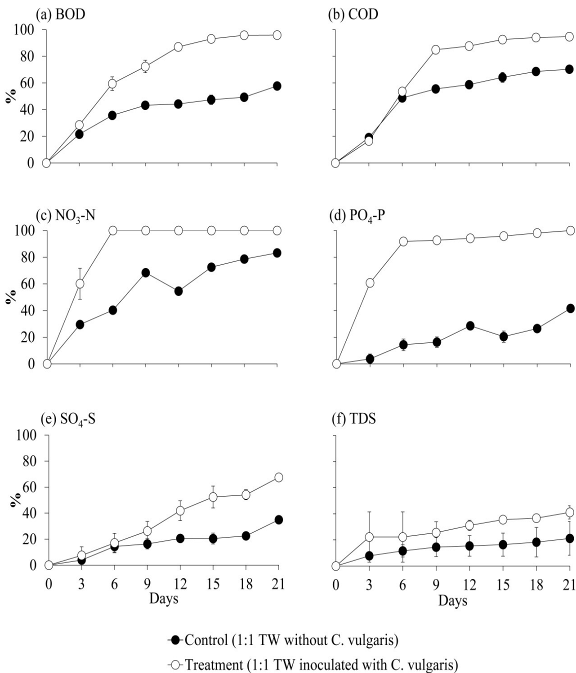
Figure 2 Reduction efficiencies for pollutants of tannery effluent after treatment with C. vulgaris
