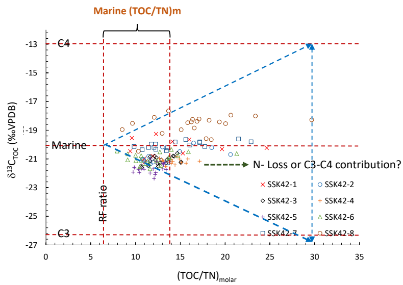
Supplementary Figure 1: Scatter plot of (\text{TOC}/\text{TN})_{\text{molar}} vs \delta^{13}\text{C}_{\text{TOC}} of sediment cores (SSK42/1-8). Dotted lines show approximate end member \delta^{13}\text{C} and (\text{TOC}/\text{TN})_{\text{molar}} ratios values of terrestrial C3, C4 and marine phytoplankton. RF = Redfield Ratio.
