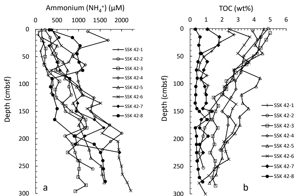
Supplementary Figure 2. Pore-water ammonium concentrations (a) and sediment TOC contents (b) down the sediment-depths of SSK42/1-8.
