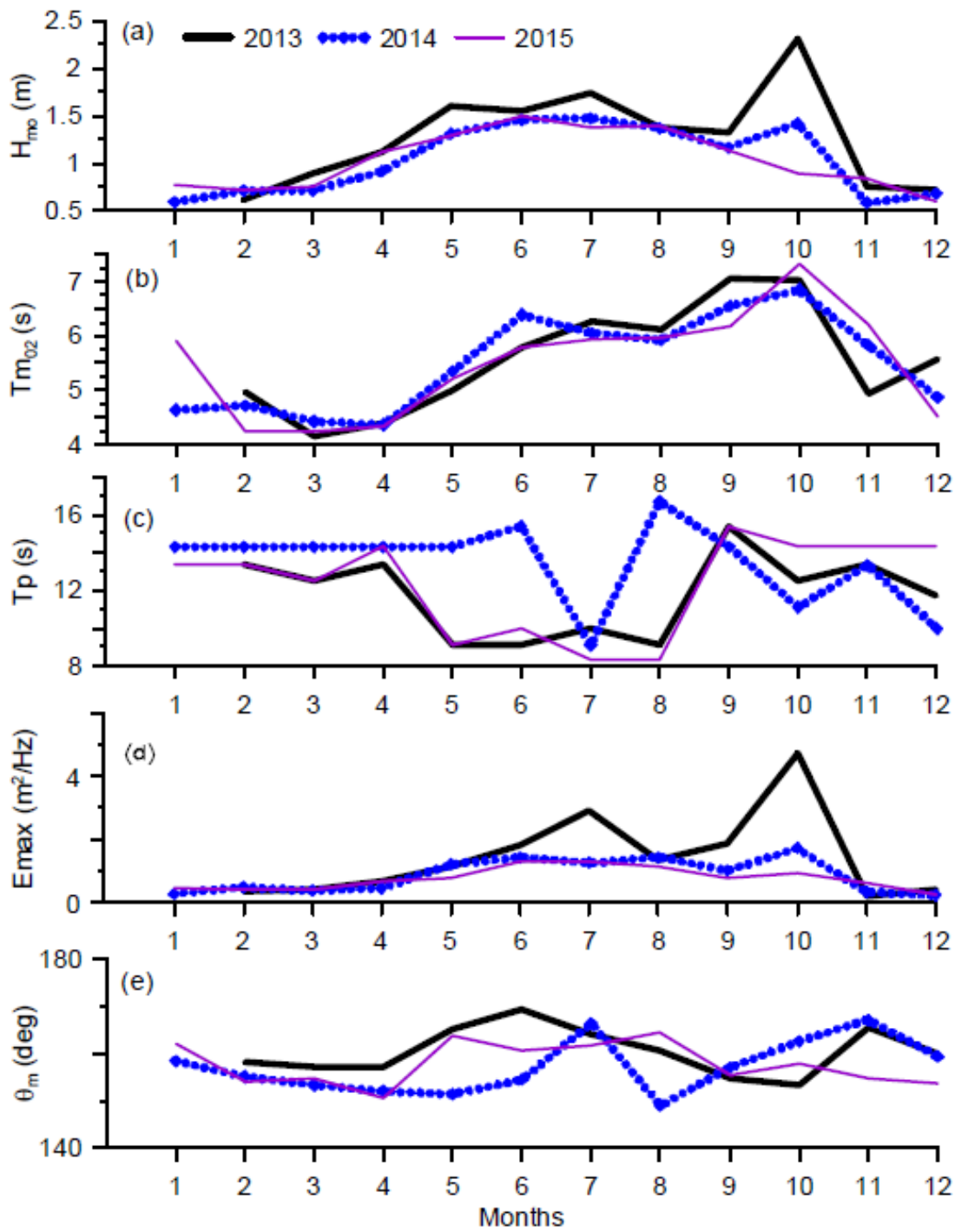
Figure 5. Wave parameters (a) significant wave height, b) mean wave period, c) peak wave period, d) maximum spectral energy density and e) mean wave direction from monthly average wave spectrum of measured data
