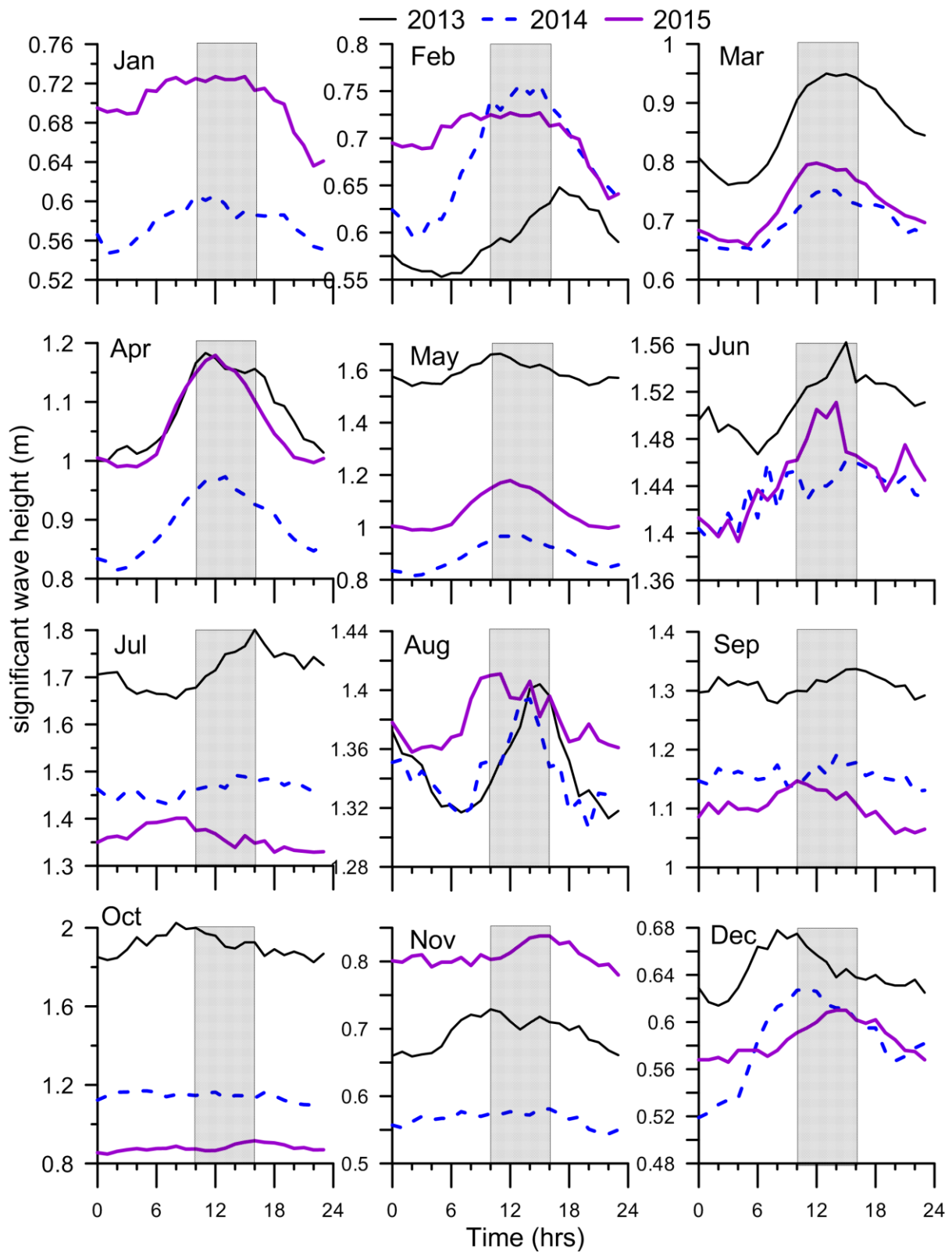
Figure 7. Diurnal variation of significant wave height in different months in 2013,2014 and 2015. The shaded area is the time during which the wave height is maximum in most of the months.
