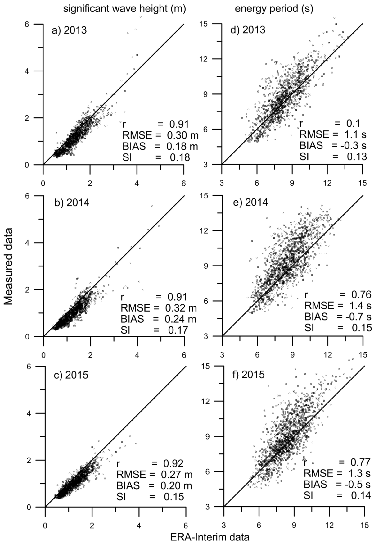
Figure 4. Scatter plot of measured significant wave height with that from ERA-I (left panel) and energy period (right panel) in different years
