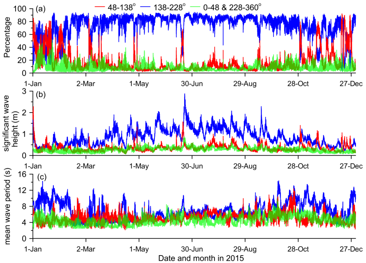
Figure 18. a) Percentage of surface height variance from different directions (0-48° & 228-360°, 48-138° and 138-228°), b) corresponding significant wave height and c) the mean wave period
