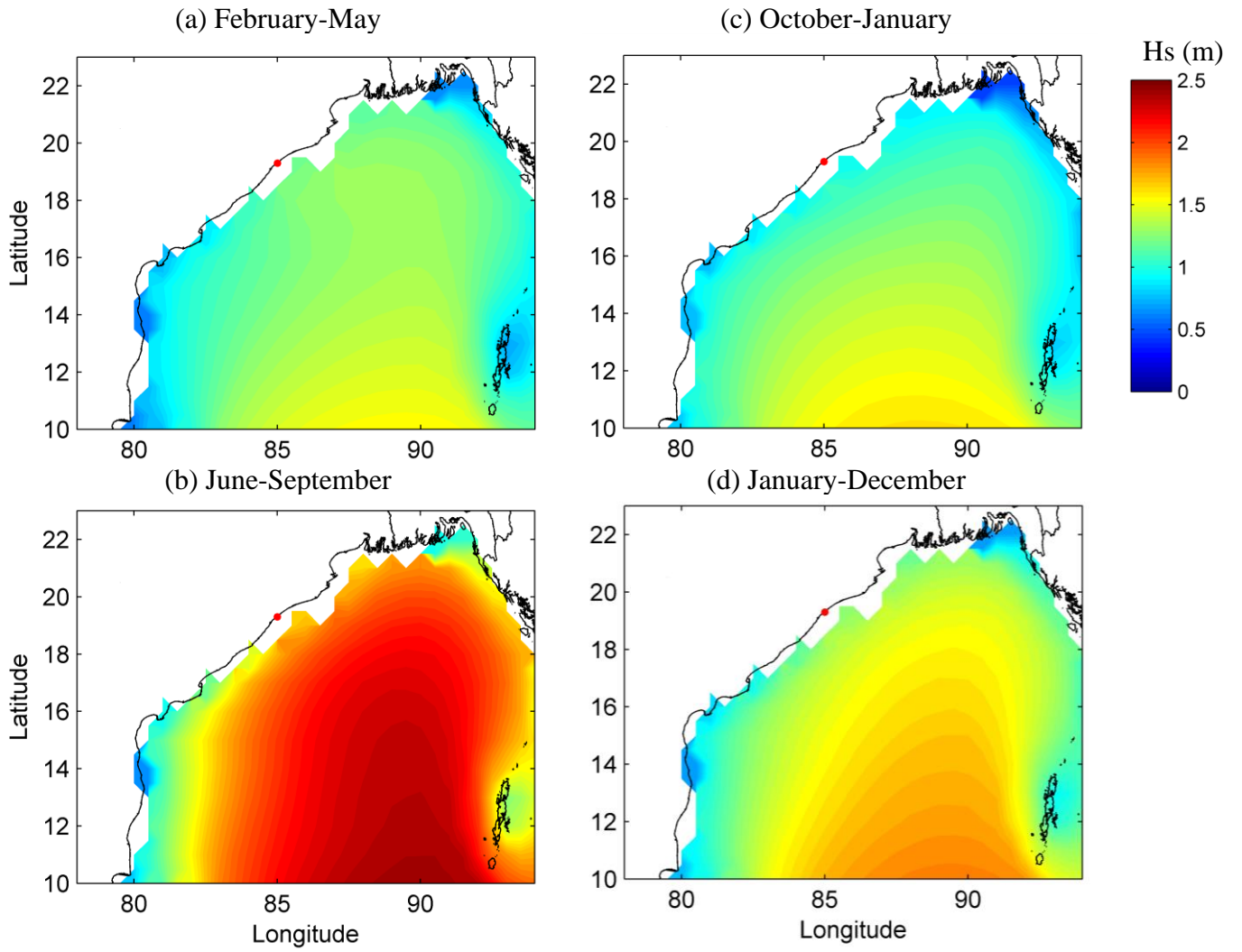
Figure 2. Mean significant wave height in Bay of Bengal during (a) February-May, (b) June-September, (c) October-January and (d) January-December. ERA-I data during 1979 to 2015 is used. The red dot near the coast indicates the waverider buoy location
