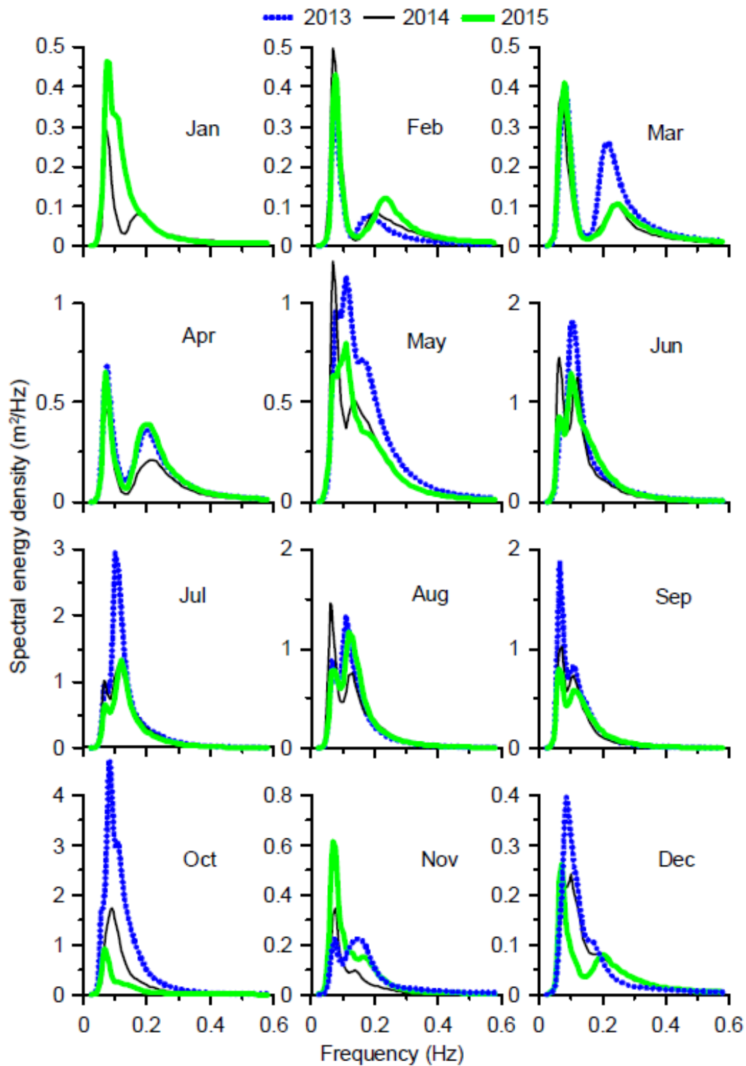
Figure 12. Monthly average wave spectrum during January to December in 2013, 2014 and 2015
