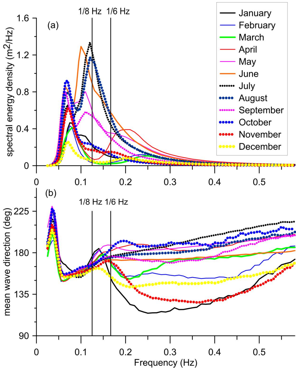
Figure 9. Monthly average wave spectrum (a) and mean wave direction (b) during January to December 2015 based on measured data
