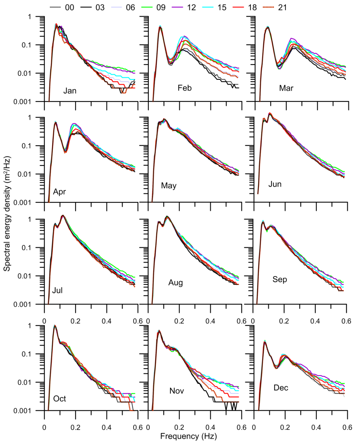
Figure 15. Monthly averaged wave spectra at different time in a day during January to December 2015 based on measured data
