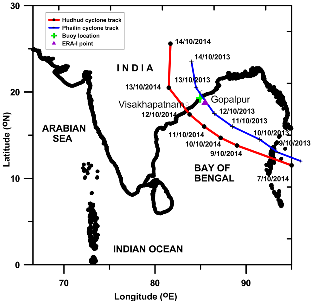
Figure 1. Location of waverider buoy in northern Bay of Bengal. The track of the tropical cyclones Phailin and Hudhud are also shown in the figure.
