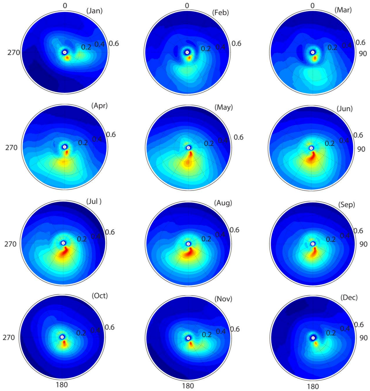
Figure 10. Monthly average wave directional spectrum in different months in 2015 based on measured data
