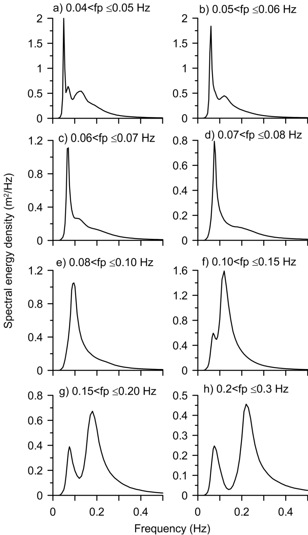
Figure 16. Average wave spectra for different peak frequency ranges
