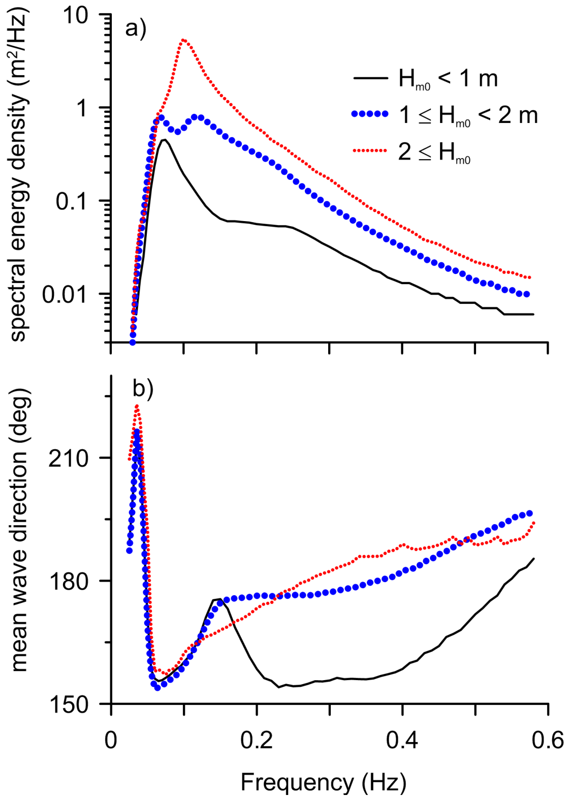
Figure 17. Plot of a) average spectral energy density and b) average mean wave direction of waves under different H_s with frequency in 2015
