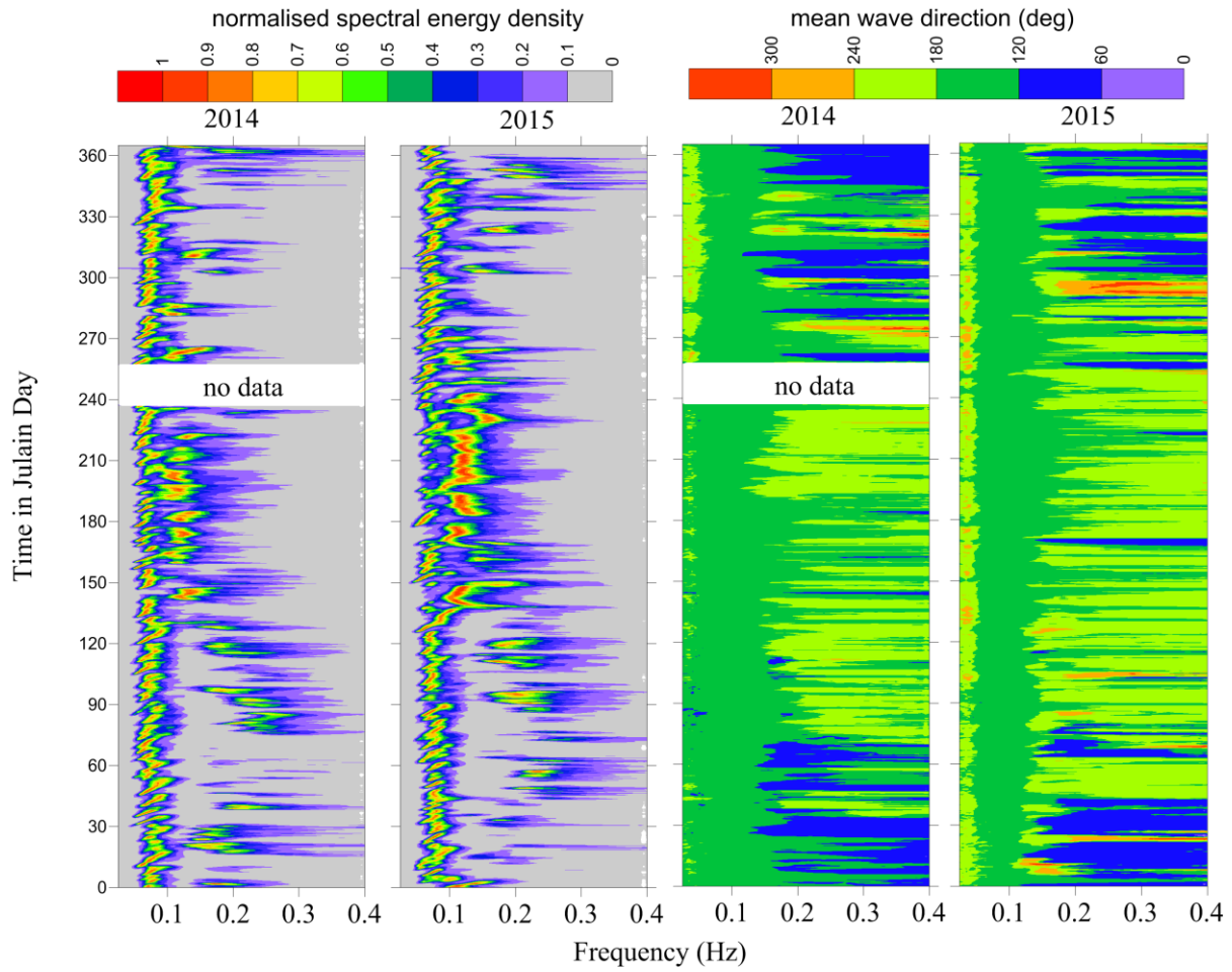
Figure 8. Left two panels shows the time series plot of the normalised spectral energy density with frequency in 2014 and 2015. Two panels in the right indicates the time series plot of wave direction with frequency
