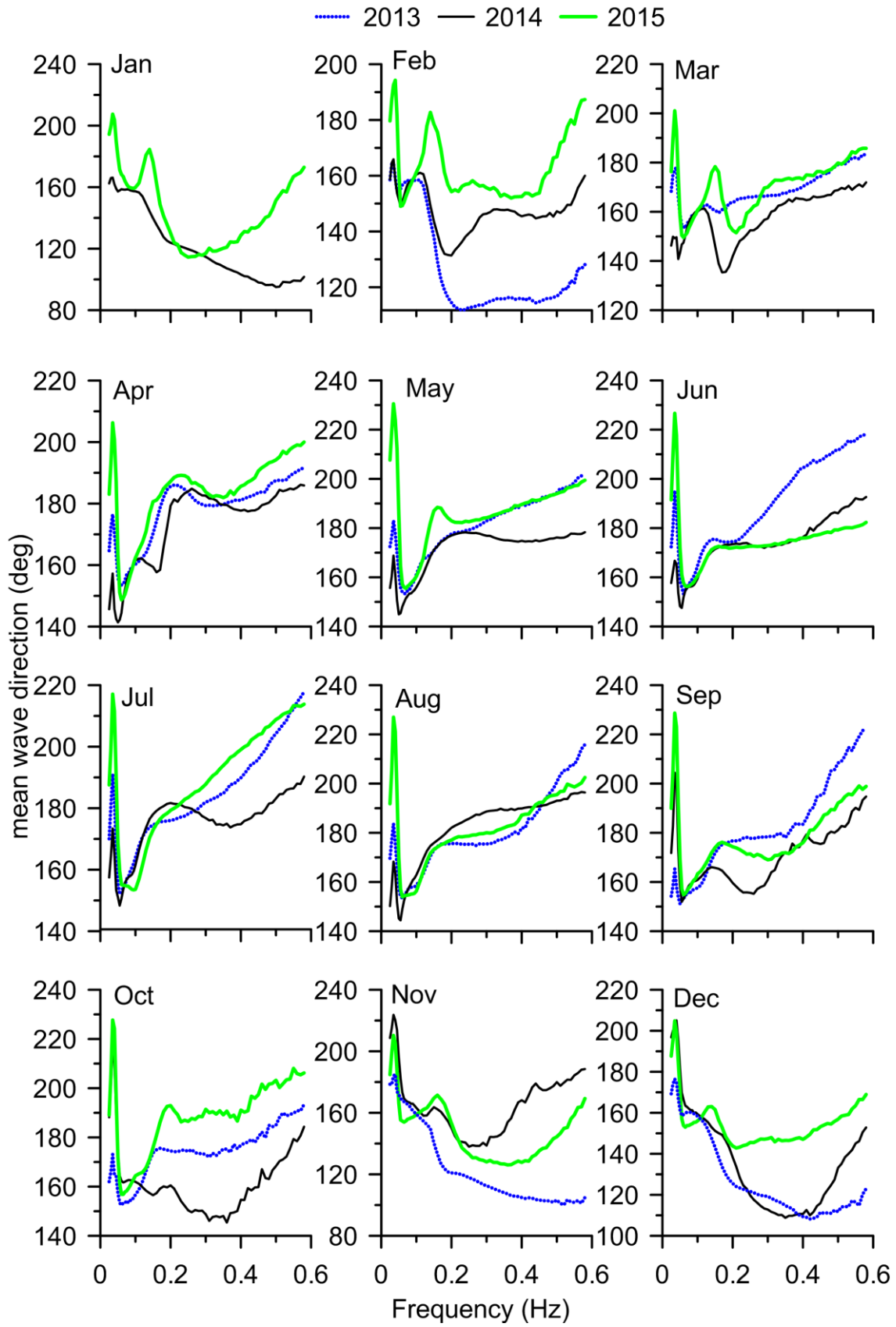
Figure 13. Monthly average wave direction during January to December in 2013, 2014 and 2015
