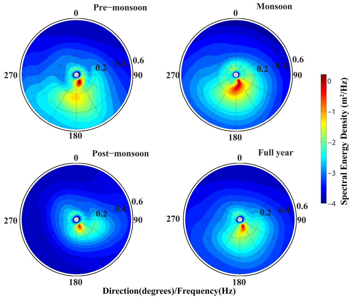
Figure 11. Seasonal average and annual average wave directional spectrum during the year 2015 based on measured data
