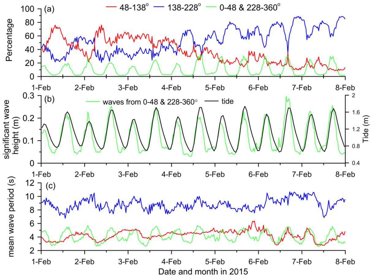
Figure 19. a) Percentage of surface height variance from different directions (0-48° & 228-360°, 48-138° and 138-228°), b) corresponding significant wave height and tide, c) the mean wave period during 1 to 8 February 2015
