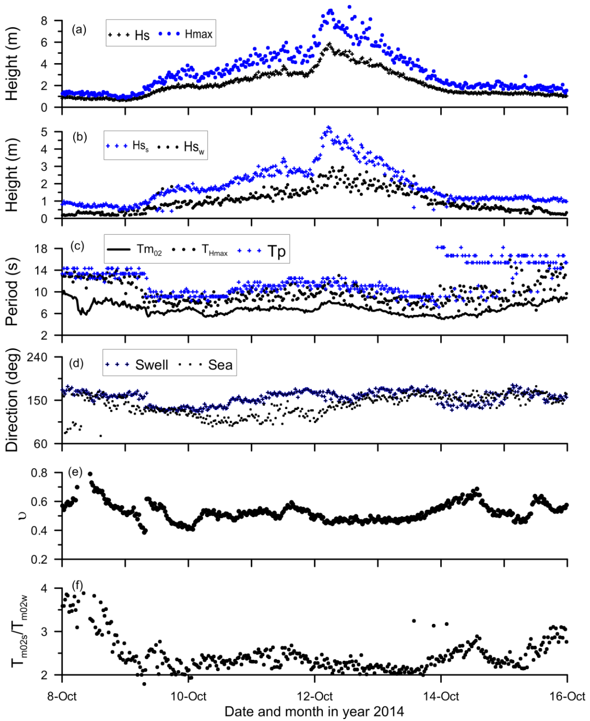
Figure 6. Plot of wave parameters during tropical cyclone Hudhud
