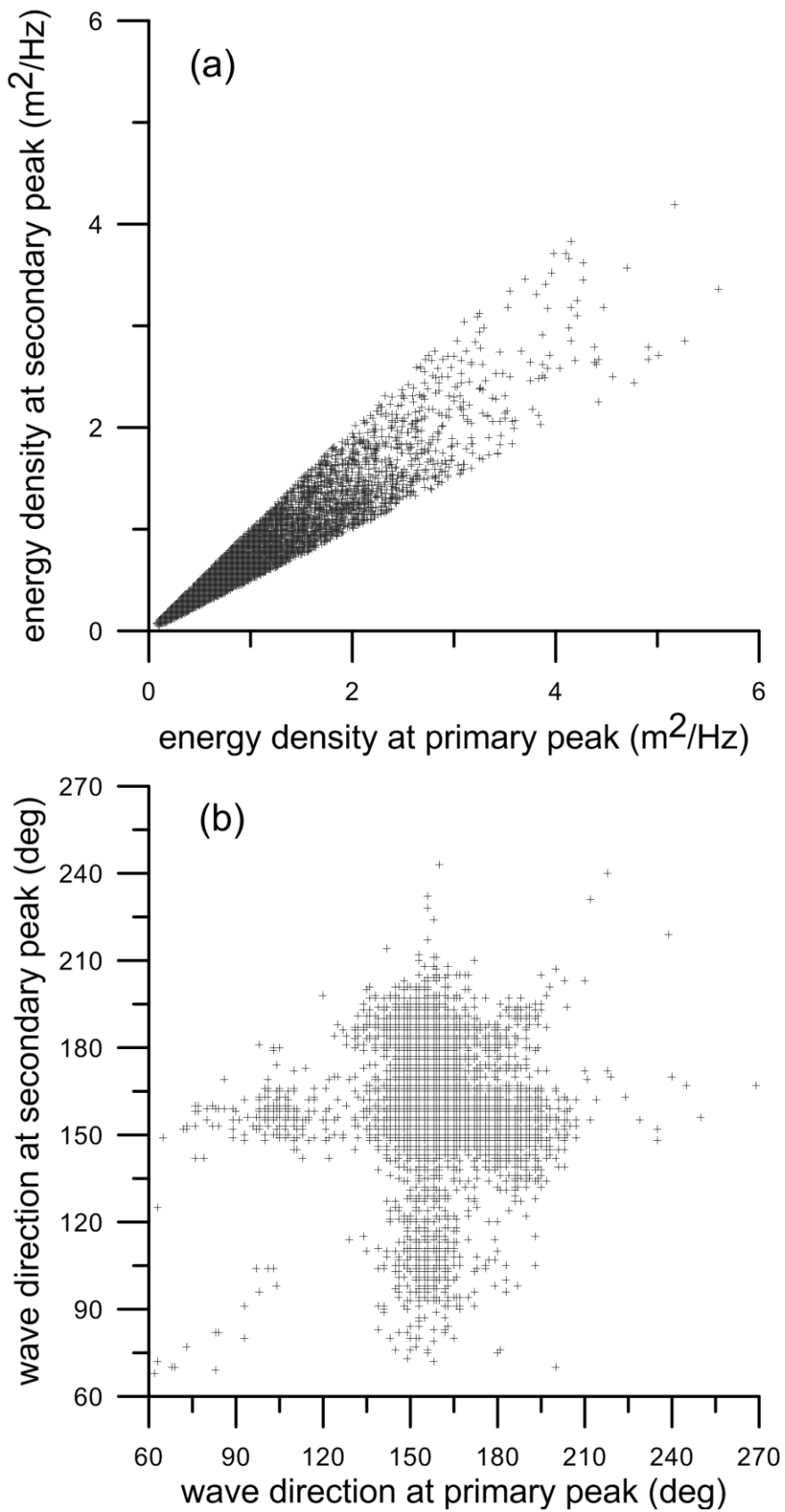
Figure 14. a) Scatter plot of spectral energy density at primary peak and at secondary peak, b) wave direction at primary peak and wave direction at secondary peak
