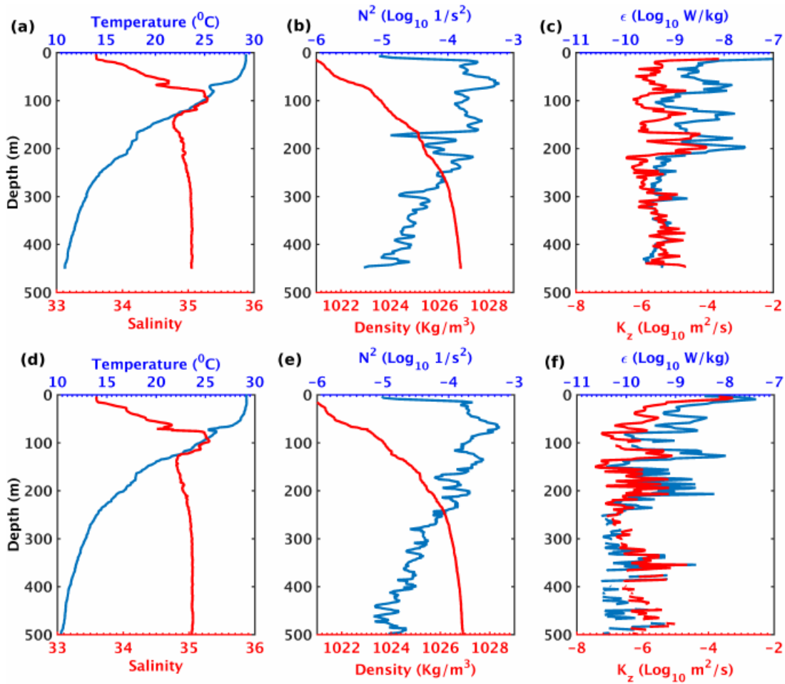
FIG . 13. Data from VMP-250 at 7° 54'N and 89°06'E on 15 July 2016 : (a) Temperature (blue) and salinity (red). (b) Squared Brunt Vaisala Frequency ( N^2 , blue) and density (red). (c) log 10 of turbulent kinetic energy dissipation rate ( \epsilon , blue) and log 10 of eddy diffusivity coefficient ( K_z , red). Near-simultaneous data from glider SG613: (d) Temperature (blue) and salinity (red). (e) N^2 (blue) and density (red). (f) log 10 of \epsilon (blue) and log 10 of K_z (red). The noise threshold of \epsilon = 10\text{--}10.5 \text{ W kg}^{-1} . The measured microstructure shear was used to infer \epsilon and K_z in the water column by assuming isotropic turbulence (Moum et al. 1995) and a mixing efficiency of 0.2 (Osborn 1980). The upper 10 m of the VMP-250 data has been removed to avoid contamination by the ship's wake.
