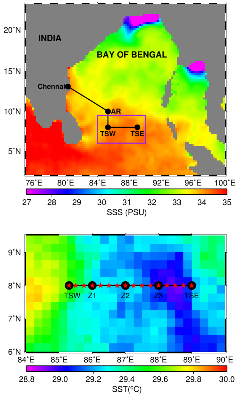
FIG. 3. Upper panel: a map of the BoB and the cruise track of the BoBBLE field program. Shading is SSS from SMAP. Lower panel: The section along which observations were made during BoBBLE. The black circles (TSW, Z1, Z2, Z3 and TSE) represent glider deployment locations (see Table 1 for details). Argo float deployments (see Table 2 for details), IOP, radiometer and VMP profiling as well as water sampling were also carried out at these locations. Stars indicate locations where additional CTD profiles were measured during the return leg of the cruise. At TSE, additionally, CTD profiles were measured from 4 to 15 July 2016. Shading indicates SST from AMSR-E.
