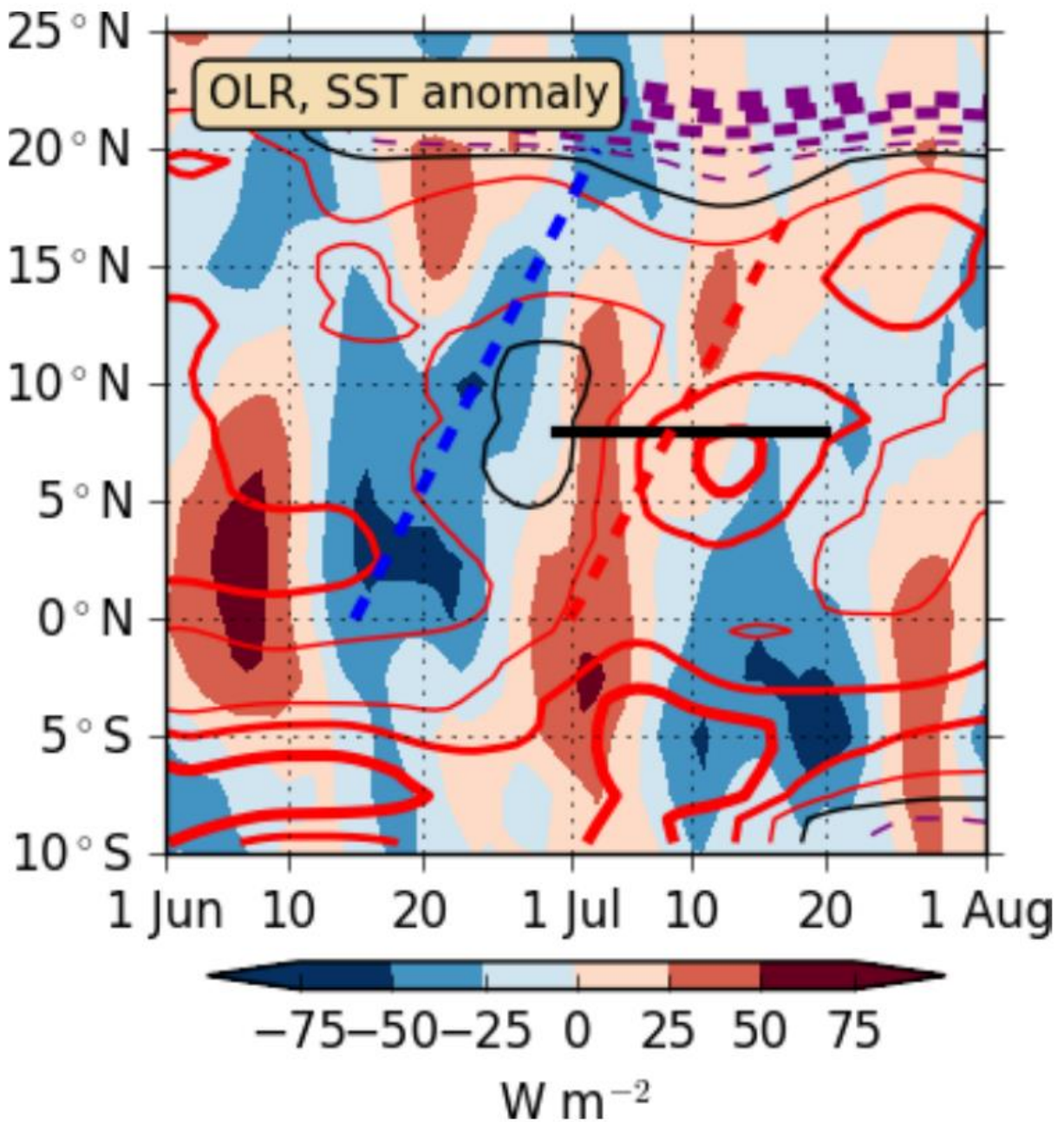
FIG. 4. Hovmöller diagram (averaged from 80°-95°E) for anomalous 5-day running mean OLR (shading interval 25 \text{ W m}^{-2} ), SST (line contour interval 0.2^\circ\text{C} ; negative contours dashed purple, zero contour solid black, positive contours solid red). The solid black line at 8^\circ \text{ N} shows the timing of the BoBBLE ship and glider and Argo float deployments. Negative (positive) OLR anomalies indicate convectively active (suppressed) phase of BSISO. The dashed blue (red) lines are shown to subjectively indicate the main axis of northward propagation of the active (suppressed) phases of the BSISO during June-July 2016.
