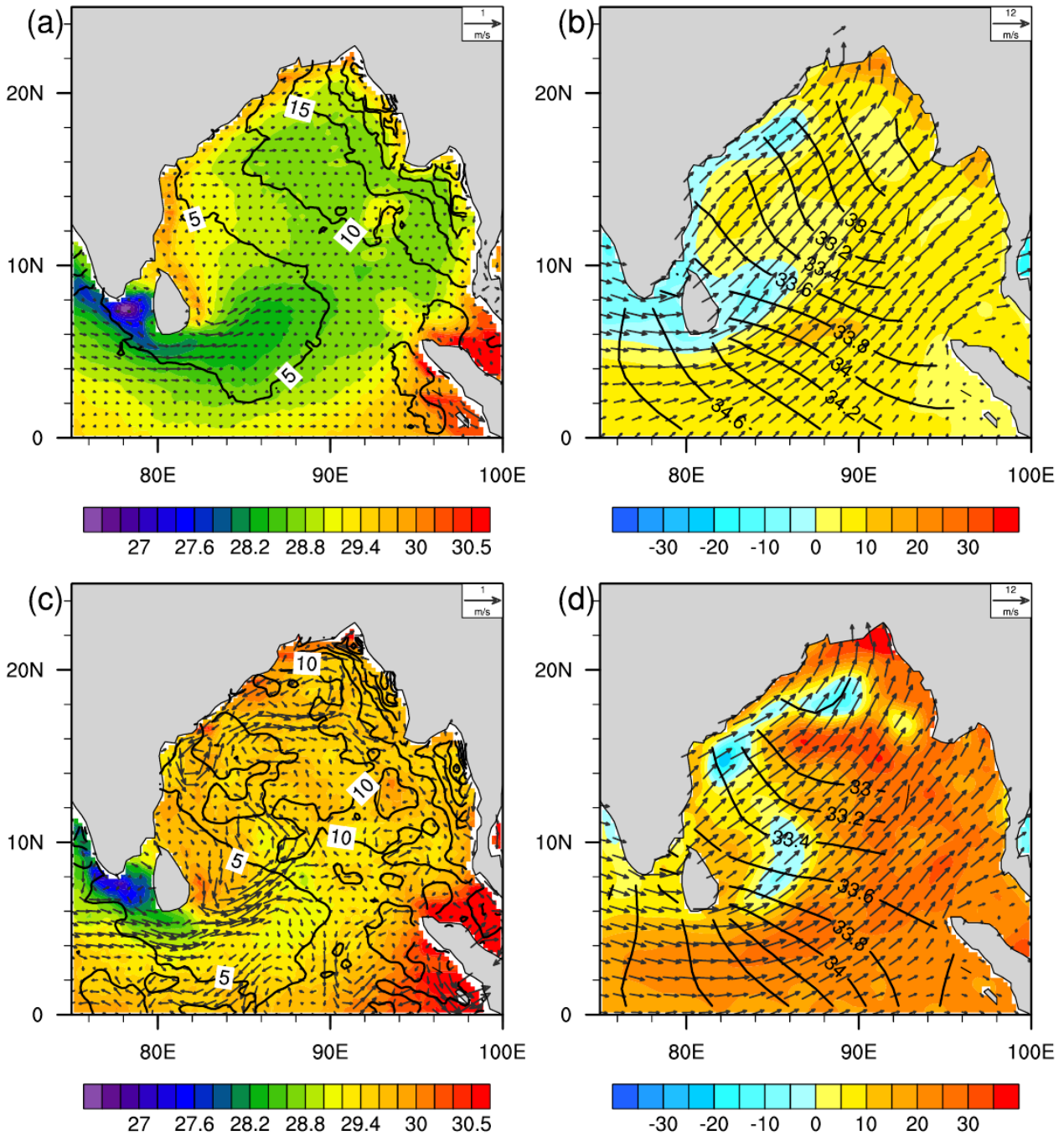
FIG . 1. Climatology for the period 23 June – 24 July. (a)TMI SST (1998–2014, shading in C), TRMM rainfall (1998–2015, contours) OSCAR (1993–2015, vector arrows); (b) AVISO MSLA (1993–2015, shading in cm), salinity from Argo (2005–2015, contours) ASCAT surface winds (2008–2015, vector arrows). Fields in panels (c) and (d) are the same as in panels (a) and (b), respectively, except that they are for the period 23 June - 24 July, 2016
