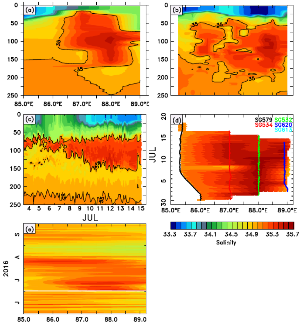
FIG. 10. High Salinity Core. (a) Vertical section of CTD salinity along 8^{\circ} N, measured during 30 June- 4 July 2016, at stations located one degree apart between 85.3^{\circ} E and 89^{\circ} E. (b) Same section as in (a) profiled during 15-20 July 2016 at stations located a quarter degree longitudes apart. (c) Time-depth section of salinity measured at TSE during 4–15 July 2016. High Salinity ( >35 ) core is highlighted using contours in (a), (b) and (c). (d) Time–longitude section of salinity averaged between 90–130 m using glider data. (e) Time–longitude section of salinity averaged between 90–130 m using Argo data.
