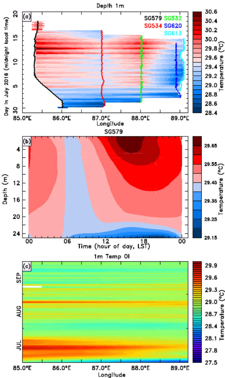
FIG . 6. (a) Longitude–time section of OI glider temperature at 1 m depth. The longitudes of the five gliders are shown by the coloured lines. (b) Average diurnal cycle of temperature for glider SG579 at the western end of the 8° N section. Time of day is in local solar time (LST). (c) Longitude–time section of temperature at 1 m depth for the July–September months of 2016, based on OI Argo data. A three day moving mean has been applied to the Argo data.
