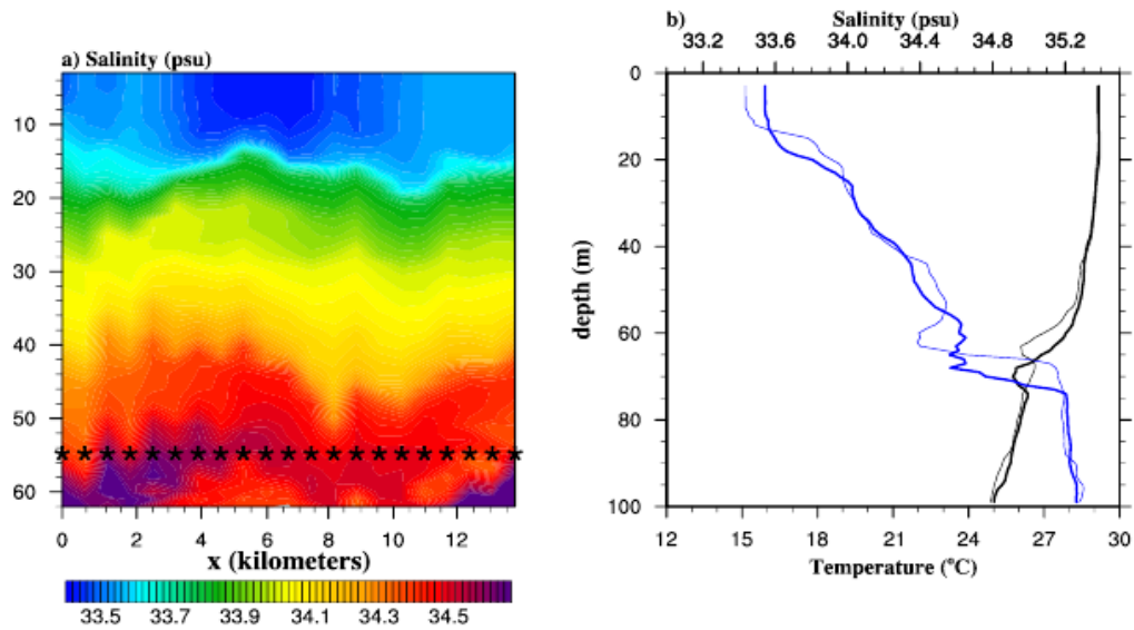
FIG . 12. uCTD observations of a rain-formed low salinity pool. (a) Salinity along a 14 km section over which 21 vertical profiles were measured just after a spell of rain. Locations of uCTD profiles are indicated using asterisks marked at a depth of 55 m. Along the depth axis, the raw data is averaged into 1 m bins before plotting.(b) Vertical profiles of temperature (black) and salinity (blue) measured outside the low salinity pool (at x = 2 km, thick lines) and inside (at x = 6 km, thin lines).
