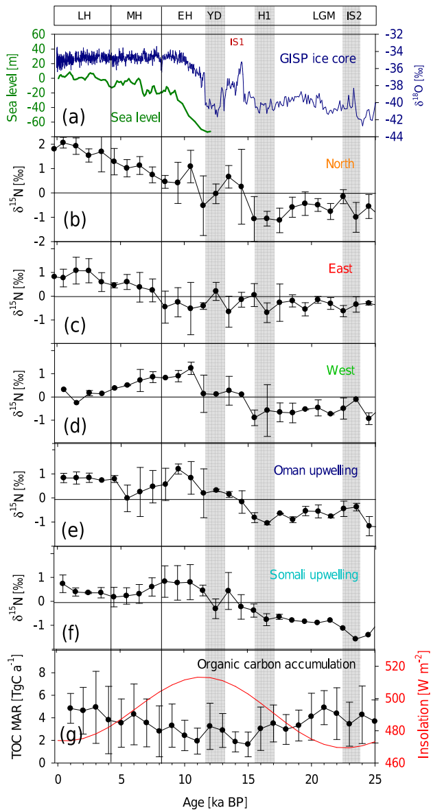
Figure 6. The \delta^{18}\text{O} values in ‰ from the GISP2 ice core (Groottes and Stuiver, 1997) and sea level (m above NN) reconstruction from the Red Sea (Siddall et al., 2003) (a) compared with millennial regional averages of normalized and averaged \delta^{15}\text{N} (‰) values from the northern (b), eastern (c), and western (d) Arabian Sea, the Oman (e), and Somali (f) upwelling area. Total organic carbon mass accumulation in the Arabian Sea (TOC MAR in \text{Tg C year}^{-1} ; data from Cartapanis et al., 2016, and Tim Rixen, unpublished) and insolation at 30^\circ\text{N} in \text{W m}^{-2} (Berger and Loutre, 1991) (g) during the last 25 kyr. Error bars denote \pm 1\sigma . Grey bars and abbreviations as in Fig. 3; interstadial 1 (IS1).
