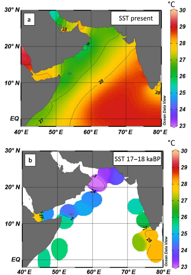
Figure 4. Annual SST distribution in ^{\circ}\text{C} from the World Ocean Atlas (Locarnini et al., 2013) (a); alkenone- and Mg/Ca-derived SST reconstruction for the time slice from 17–18 ka BP (b) from cores shown in Fig. 1.
