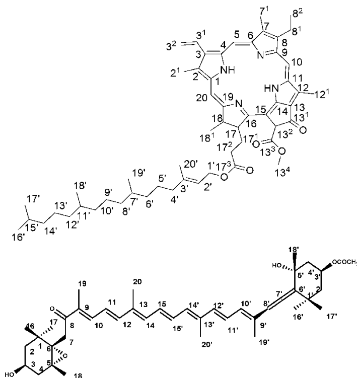
Figure 1. Chemical Structures of pheophytin- a ( 1 ) and fucoxanthin ( 2 ) isolated from S. cinereum .
