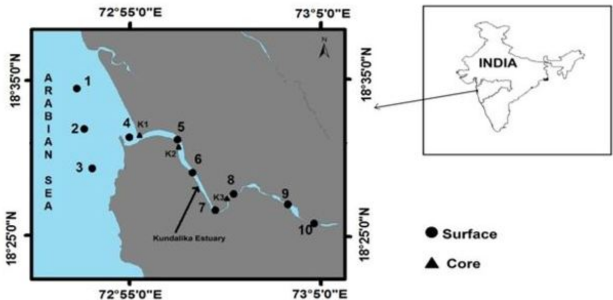
Fig. 1 — Map showing study area and sampling locations.
