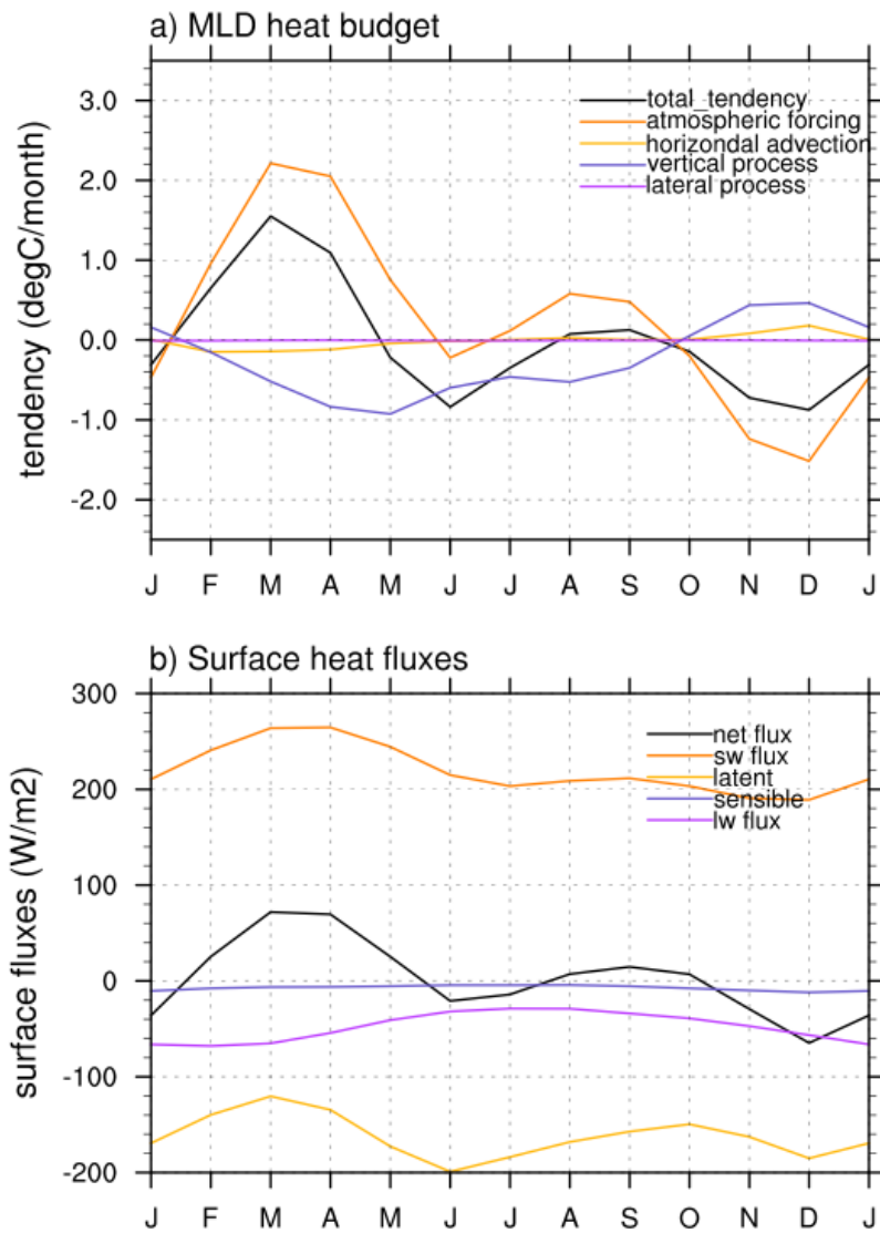
Figure 4. Averaged BoB climatological seasonal cycle of FCTL (a) mixed layer heat budget terms ( ^{\circ}\text{C}\cdot\text{month}^{-1} , see section 2.3 for details) and (b) surface net heat fluxes and its four components ( \text{W}\cdot\text{m}^{-2} ).
