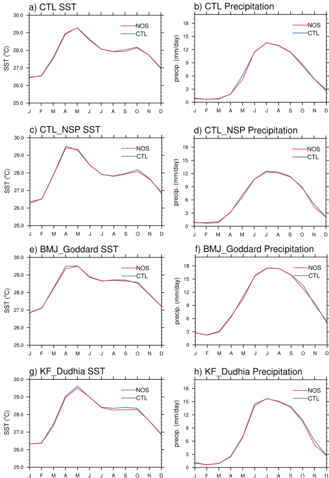
Fig. 8: Averaged BoB CTL and NOS mean seasonal cycle of (a) SST and (b) precipitation (i.e. same as 8ef but without flux corrections). (c)-(d) Same as (a)-(b), but for CTL-NSP and NOS-NSP (i.e. with the penetration of solar radiation into the ocean de-activated). (e)-(f) Same as (a)-(b), but for CTL-G and NOS-G (Goddard shortwave radiation parameterization). (g)-(h) Same as (a)-(b), but for CTL-KF and NOS-KF (Kain-Fritsch convective parameterization).
