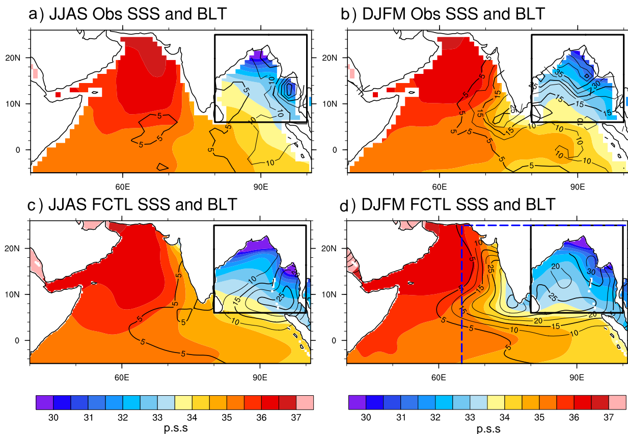
Fig. 3 Summer (June to September: JJAS) ( left ) and Winter (December to March; DJFM) ( right ) climatologies of observation ( top ) and FCTL ( bottom ) Sea Surface Salinity (SSS, shading, pss) and Barrier Layer Thickness (BLT, contours, meters). For the model data, a horizontal smoothing has been applied, with a similar spatial scale than that used for the observationally-derived climatologies i.e. with a smoothing radius of 175 km for BLT as for de Boyer Montegut et al. (2004) and 4° (444 km) for SSS as for the NIOA climatology. The dashed blue frame on panel d indicates the region over which the influence of salinity on vertical mixing is neglected in the series of “NOS” experiments (see table 1).
