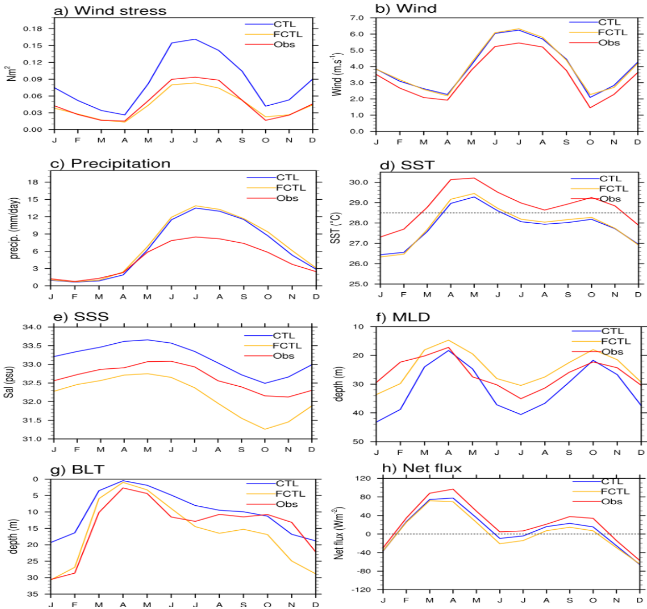
Fig. 2 Averaged BoB ( 6^{\circ}N-25^{\circ}N , 80^{\circ}E-100^{\circ}E , see region on Fig. 3) climatological seasonal cycle for CTL (Blue) & FCTL (flux correction applied on wind stress: see text for details, yellow) experiments and observations (red) for (a) wind stress ( N.m^{-2} ), (b) wind speed ( m.s^{-1} ) (c) precipitation ( mm.day^{-1} ) ( W.m^{-2} ), (d) Sea Surface Temperature (SST, ^{\circ}C ), (e) Sea Surface Salinity (SSS, psu), (f) mixed layer depth (MLD, m) (g) Barrier Layer Thickness (BLT, m) and (h) net heat flux. Observed climatologies are obtained from the TropFlux 1990-2007 average for wind stress and net heat flux, ERA-interim 1990-2007 average for wind speed, TMI 1998-2006 average for SST, TRMM 1998-2011 average for rainfall, NIOA climatology for SSS and de Boyer Montegut et al. (2004) climatology for MLD and BLT. The dashed horizontal line on panel d indicates the observed threshold ( 28.5^{\circ}C ) for deep atmospheric convection.
