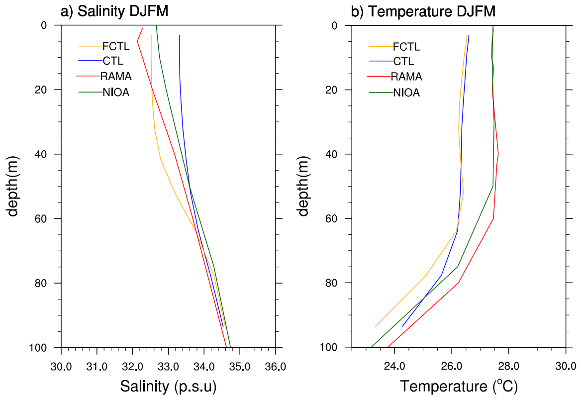
Fig 9. Winter (DJFM) temperature and salinity BoB-averaged climatological profiles for longitude 90°E and latitude 15°N from the RAMA buoy (red), NIOA product (green), CTL (blue) and FCTL (yellow).
