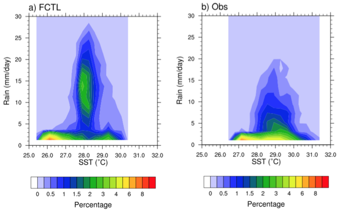
Figure 10: SST-rainfall relation in (a) the FCTL simulation and (b) from TMI and TRMM observations. The probability density function (%) was constructed from daily SST and rainfall over the BoB region, using 2.5 \text{ mm}\cdot\text{day}^{-1} and 0.33^\circ\text{C} wide bins.
