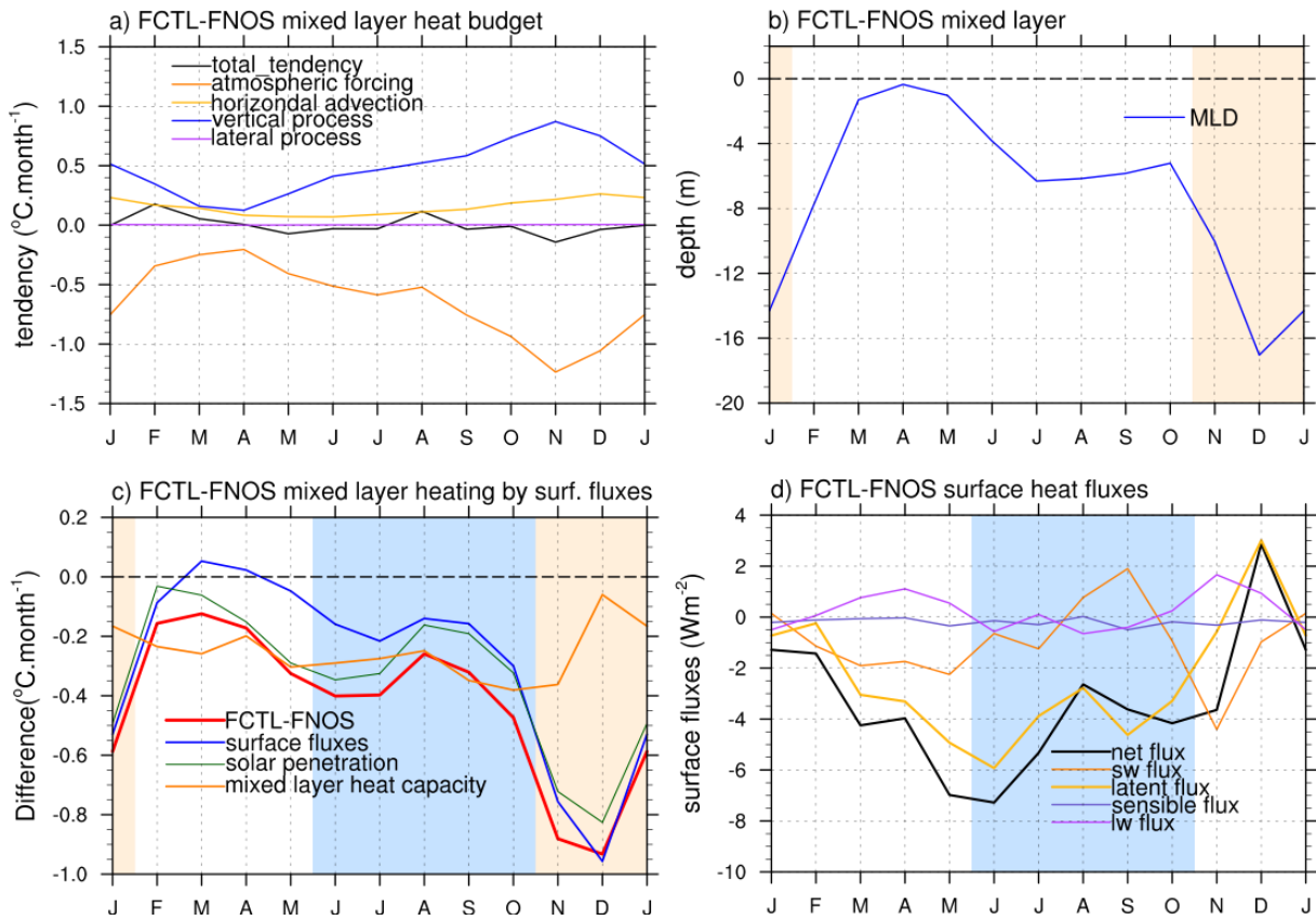
Figure 7. Average BoB climatological seasonal cycle of FCTL minus FNOS ( a ) MLD heat budget ( ^{\circ}\text{C}\cdot\text{month}^{-1} ), ( b ) MLD (m) and ( d ) surface fluxes ( \text{W}\cdot\text{m}^{-2} ). ( c ) shows the FCTL minus FNOS recomputed atmospheric forcing term (thick red curve). The green curve allows to evaluate the effect of solar penetration, the blue curve the effect of the change in surface heat fluxes and the orange one the effect of the changes in mixed layer heat capacity (see text and Annex A for details). The blue shading highlights the July to October period and the salmon shading highlights the November to January period.
