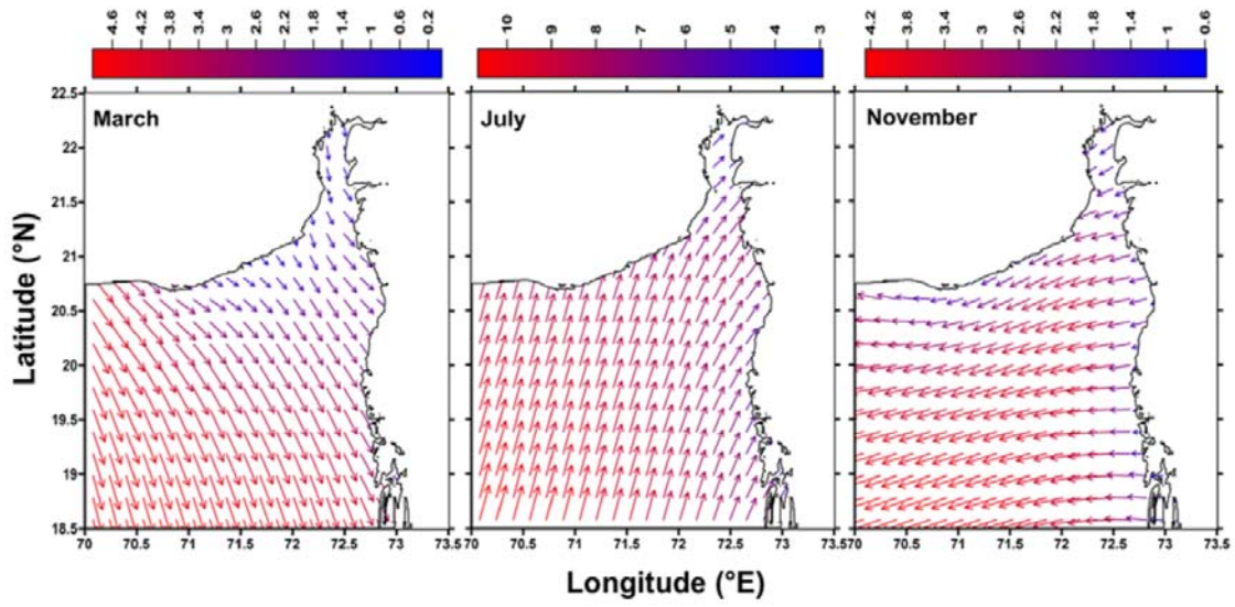
Figure 11: Seasonal wind regime of Gulf of Khambhat in March (representing pre-monsoon), July (representing monsoon) and November (representing post-monsoon). Wind speed is in m/s
