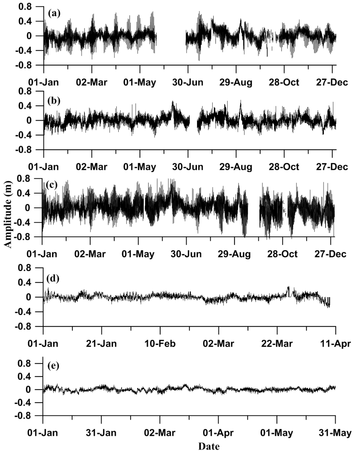
Figure 9. Non-tidal residual of sea-level at selected locations; a) Daman, b) Hazira, c) Bhavnagar, d) Pipapvav and e) Diu
