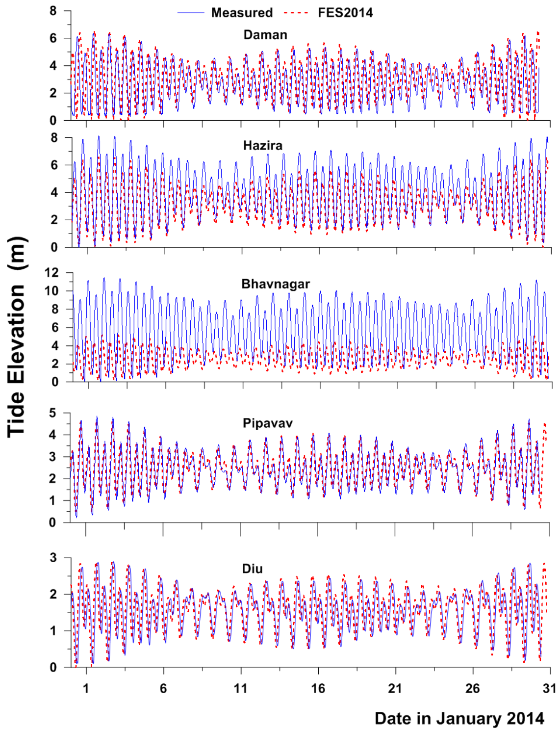
Figure 4. Comparison of FES2014 tide with measured tide at Daman, Hazira, Bhavnagar, Pipavav and Diu
