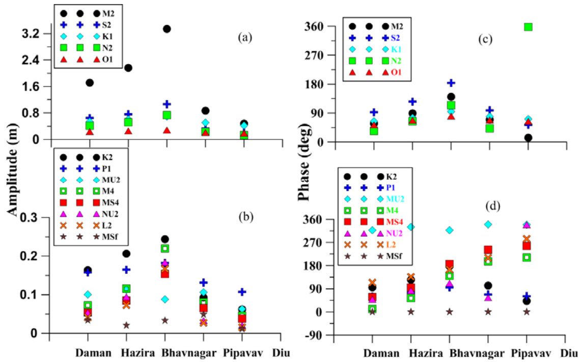
Figure 5. a) and b) Amplitude distribution of major astronomical tidal constituents at 5 locations in the study area based on measured data and the corresponding phase lag distribution is shown in c) and d)
