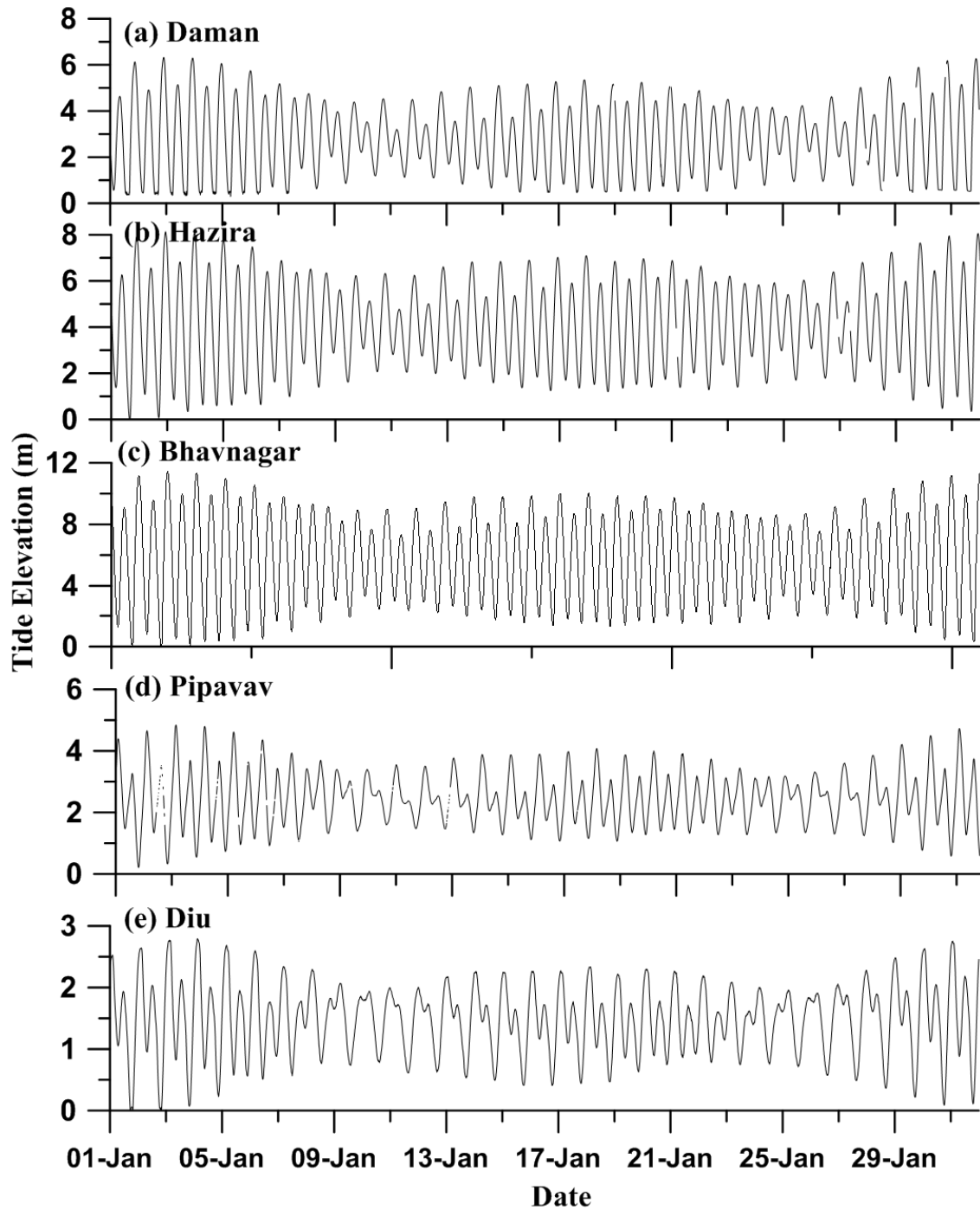
Figure 2. Time series plot of the measured tide data during 1 January to 31 January 2014 at a) Daman, b) Hazira, c) Bhavnagar, d) Pipavav and e) Diu. Tides are presented with respect to Chart Datum
