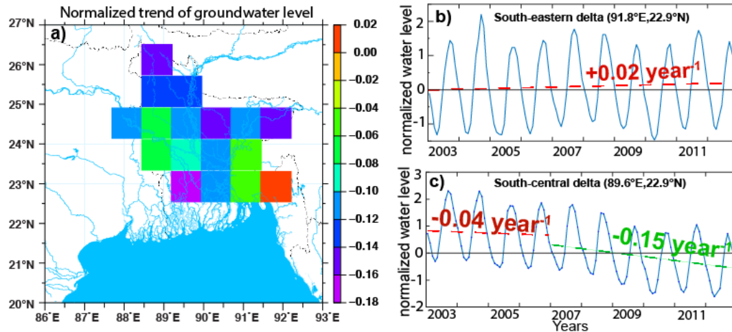
Fig 8. (a) Normalized long-term trend of groundwater level in the hindcast of Khaki et al. (2018). Timeseries of normalized groundwater level extracted at the two locations showing orange shade (for b) and purple shade (for c) in panel (a). The linear tendency lines are superimposed, along with the corresponding values of the tendencies. For (c), we computed separately two tendency lines, over 2003-2006 and over 2007-2012.
