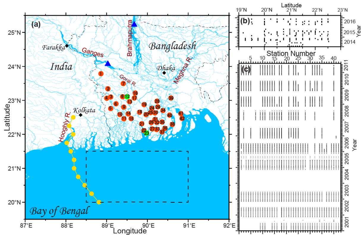
Figure 1. (a) Distribution of the observation stations. Red bullets show the salinity stations, with station numbers. Green bullets show the stations where we also analyzed water level. Blue triangles show the river gauge locations. The ship track with salinity data locations in Hooghly estuary is in yellow. Other locations discussed in the text (e.g. Farakka dam) are displayed. The dashed box in the ocean features the domain considered for analyzing altimetric sea level data. (b) Spatio-temporal coverage of salinity data in Hooghly River. (c) Spatio-temporal coverage of salinity data for Bangladesh stations.
