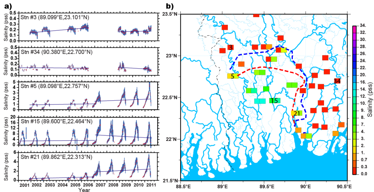
Figure 4. (a) Timeseries of salinity observed at selected stations (red points). The blue vertical bars in all panels feature the year-to-year standard deviation, computed month-wise, separately over the 2001-2006 period and over the 2007-2011 period. For each of these two periods, we superimpose the linear fit in thin solid line. (b) Salinity climatology in April, with the positions of the pre-2006 (red) and post-2007 (blue) 2 units isohaline. The right-shifted squares in certain stations show the April climatological salinity computed over the post-2007 period only.
