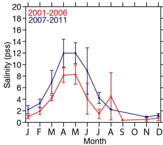
Figure 5. Monthly climatology of salinity observed at station #15 (89.600°E, 22.464°N), distinguishing the pre-2006 (red) and the post-2007 (blue) periods.
