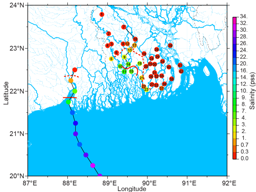
Figure 2. Long-term mean of salinity at all stations. The red dashed/solid line indicates the climatological position of the 2 units isohaline in April/August, respectively. The thin black lines feature the central and western sections displayed in Fig3a and 3b, respectively
