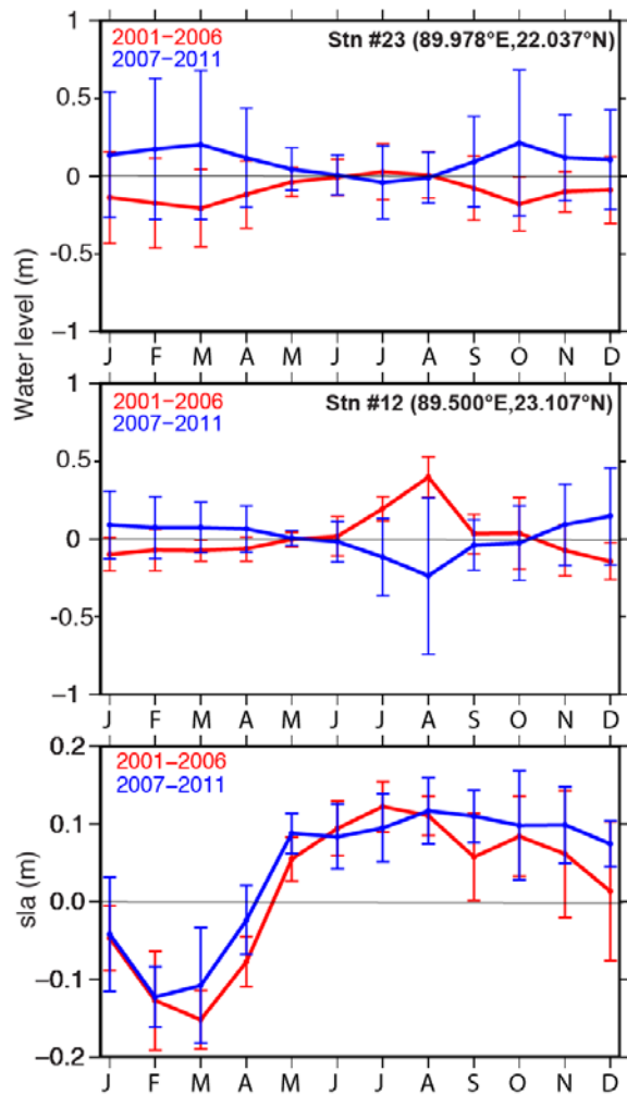
Fig 7. (top) Monthly climatology of river water level observed at station #23, for the pre-2006 (red) and the post-2007 (blue) periods. The monthly climatology of river water level has been removed, for clarity. (middle) Same, for station #12. (bottom) monthly climatology of altimetric sea level averaged over the box displayed on Fig. 1, for the pre-2006 (red) and the post-2007 (blue) periods. The vertical bars in all panels feature the year-to-year standard deviation, computed month-wise.
