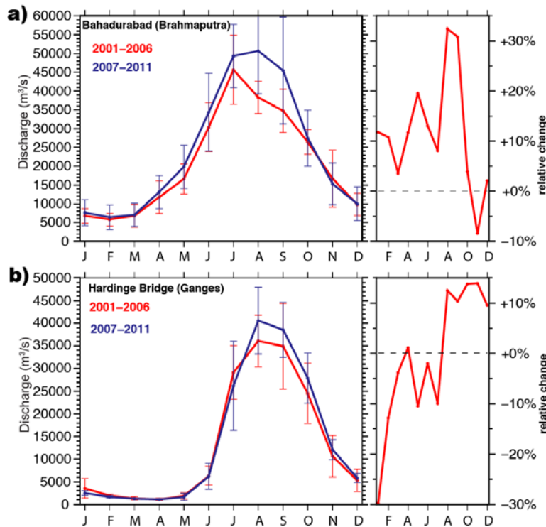
Figure 6. Monthly climatology of river discharge for the Brahmaputra (top left) and for the Ganges (bottom left), distinguishing the pre-2006 (red) and the post-2007 (blue) periods. The right panels show the corresponding relative change between the two periods, expressed in percent of the pre-2006 values.
