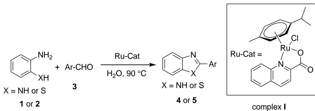
Scheme 1. Reaction pathways for the synthesis of 2-arylbenzimidazole and 2-arylbenzothiazole.
