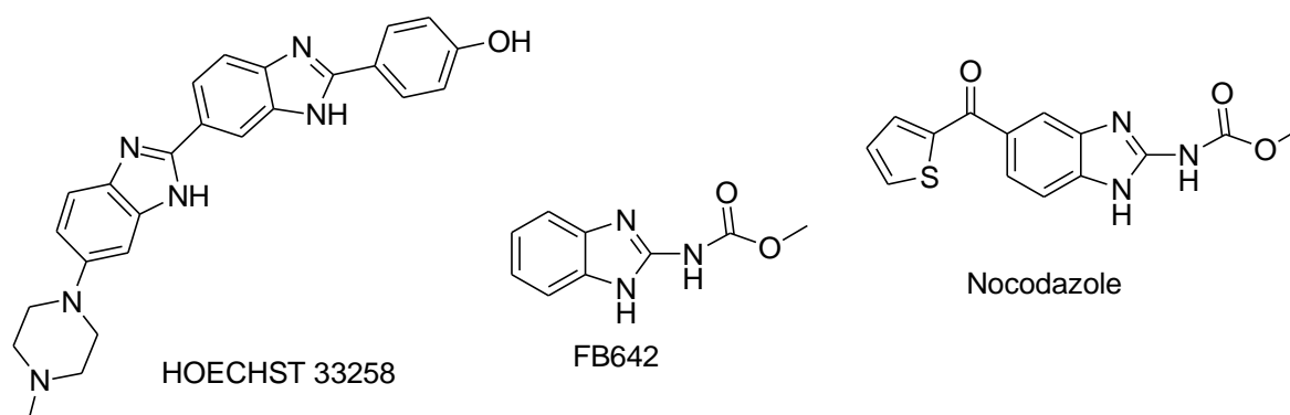
Figure 1. Structures of benzimidazole compounds with anticancer properties.
