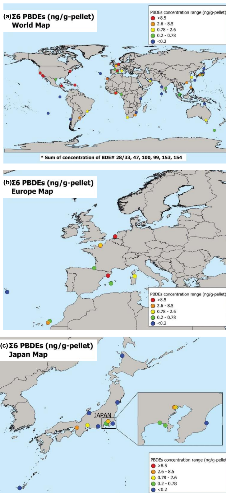
Fig. 4 Concentrations of \Sigma_6 PBDEs in beached plastic resin pellets. \Sigma_6 PBDEs: sum of concentrations of BDE-28 / 33, 47, 99, 100, 153, and 154. (a) Global, (b) Europe, and (c) Japan
