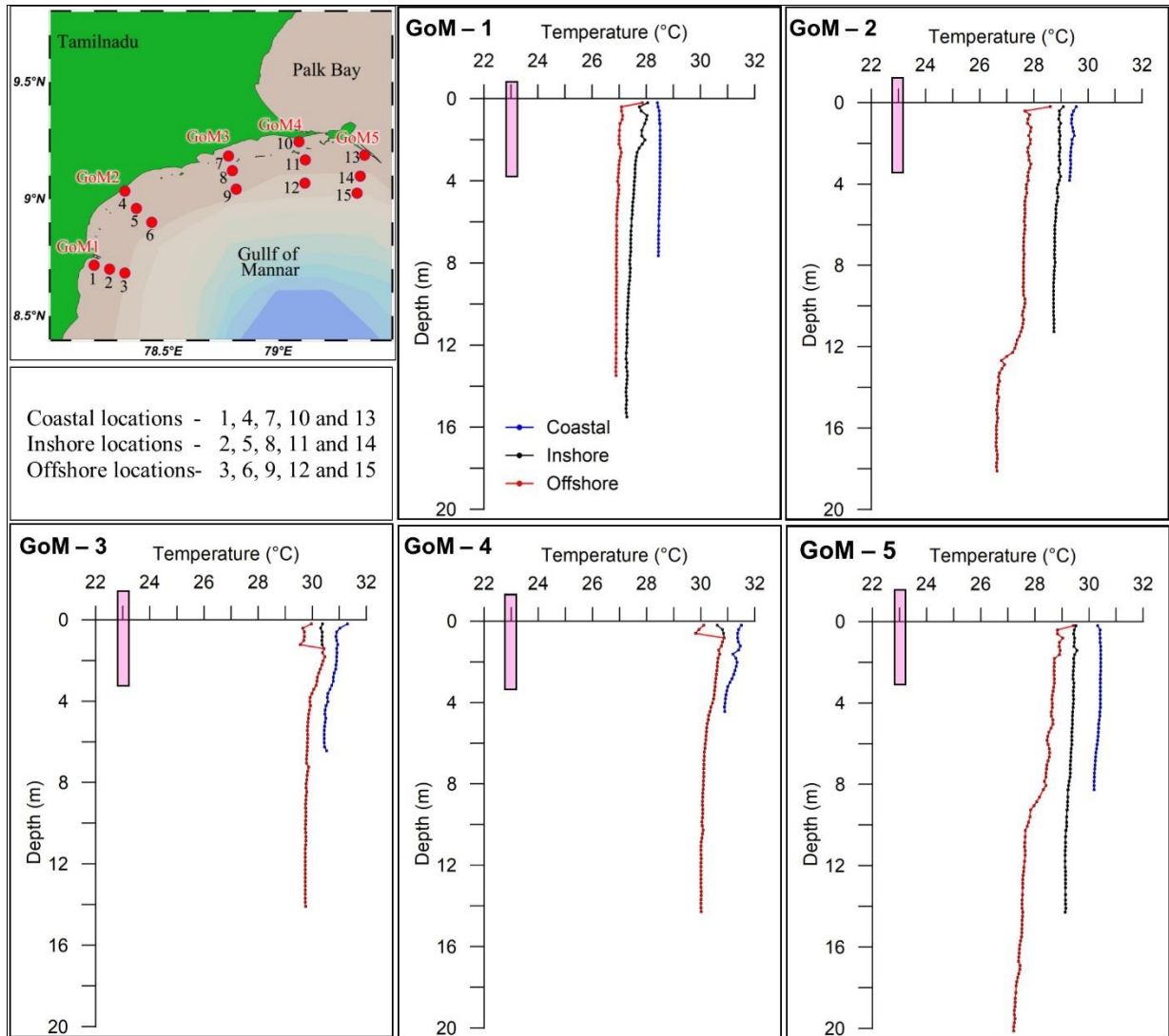
Figure 6 - The vertical distribution of temperature in five cross-shore transects along the Indian shelf in the GoM during the Southwest Monsoon (September 2010). The upwelling temperature ( <23^{\circ}\text{C} ) is indicated on the x-axis as a pink bar to show the significantly warmer water that prevails in the GoM during the Southwest Monsoon
