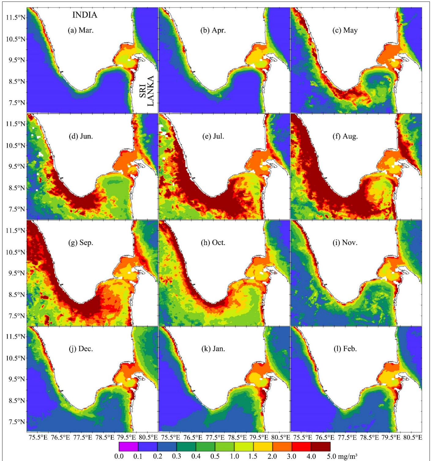
Figure 5 - Chlorophyll- a ( \text{mg m}^{-3} ) distribution in the study domain and its monthly variations associated with the seasonal evolution from the Pre-Monsoon to the Northeast Monsoon period. The presence of moderate to the high concentration of chlorophyll- a occurs in the GoM most of the year.
