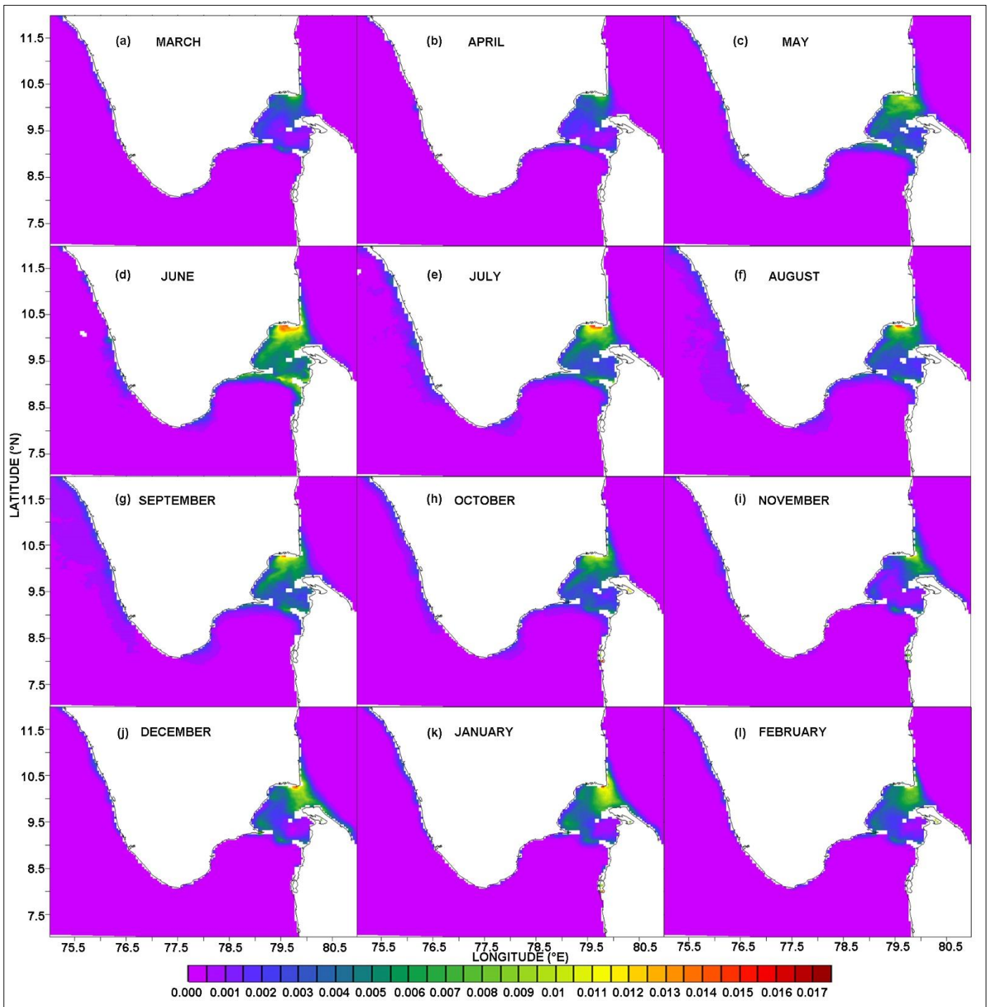
Figure 4 – Monthly satellite reflectance at 645nm (a measure of turbidity) showing high transparency of the water column in the study domain compared to the adjacent regions especially the Palk Bay.
