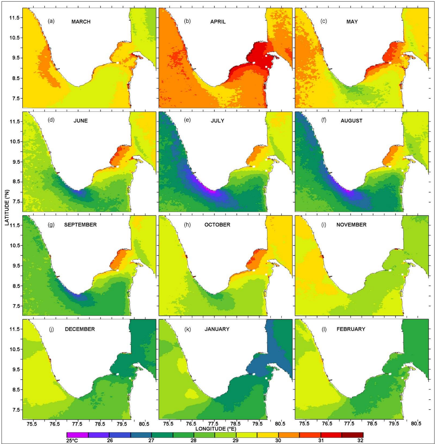
Figure 3 - SST ( ^{\circ}\text{C} ) distribution in the study domain showing its monthly variations associated with the seasonal evolution from the Pre- Monsoon (March-May) to the Northeast Monsoon (November - February) period. Relatively cool SST in the GoM was observed during the SWM due to the advected surface waters from the Indian south-western shelf and during the NEM due to the Bay of Bengal water intrusion.
