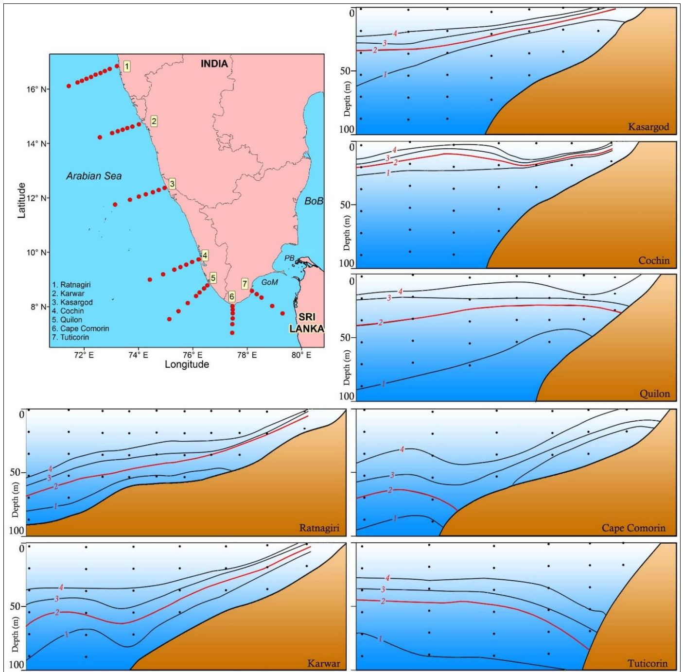
Supplementary Figure 2 - Vertical distribution of dissolved oxygen ( \text{ml L}^{-1} ) along seven cross-shore transects along the central and southwest coast of India during the Southwest Monsoon. Clear signatures of upwelling as up-sloping of isolines of oxygen and stratified water column closer to the coast were evident in all transects except in the Tuticorin transect (Transect 7). It is evident except in the Tuticorin transect that hypoxic subsurface waters from offshore reach the relatively shallower water closer to the coast. In the Tuticorin transect, the surface water column in the nearshore waters was well mixed (deeper mixed layer) followed by a downwelling of isolines of dissolved oxygen in the subsurface waters indicating the absence of upwelling there (adapted from Johansen et al., 1983).
