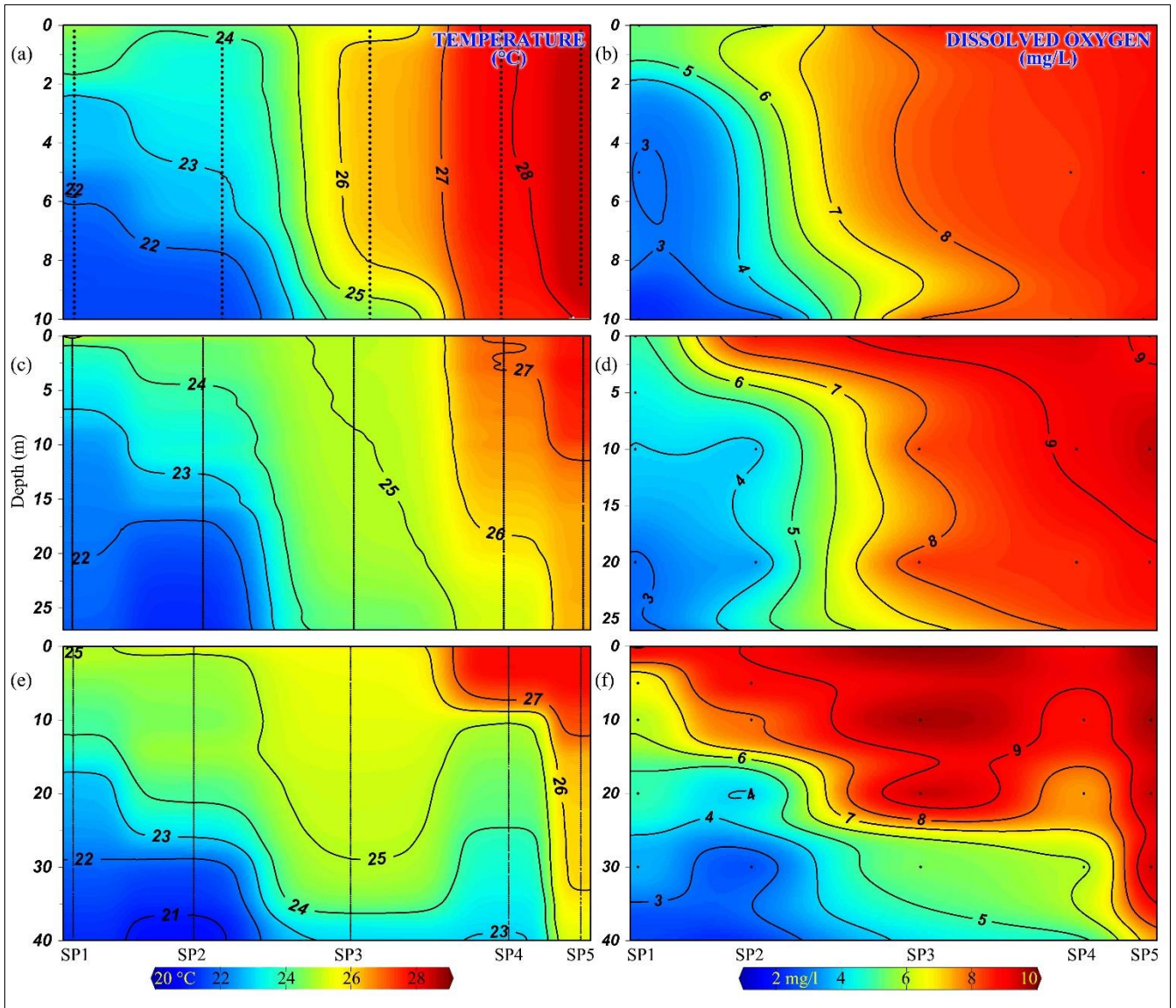
Figure 8 - Vertical distribution of temperature ( ^{\circ}\text{C} ) and dissolved oxygen ( \text{mg L}^{-1} ) in the nearshore waters along the southwest coast of India up to the western boundary of the GoM (Tuticorin). Panels represent (a & b) 10m, (c & d) 25m and (e & f) 40m depth during the Southwest Monsoon (September 2018). SP1 to SP5 are as indicated in Figure 1.
