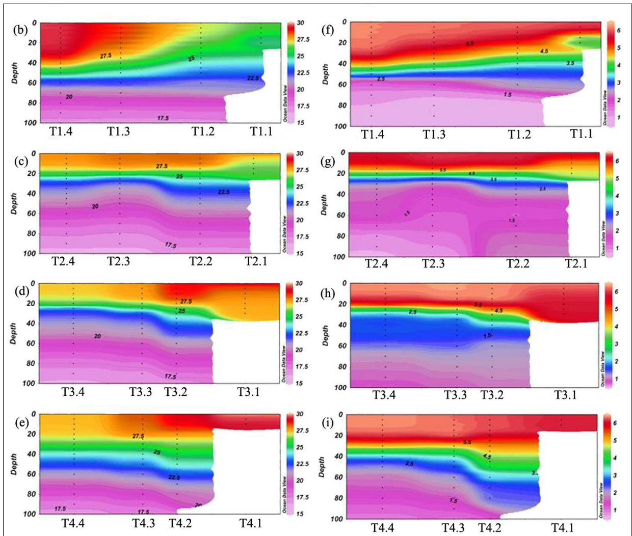
Figure 10 - (a) Four cross-shore transects (T1 - T4) selected in the GoM for ROM projections. The vertical structure of (b-e) temperature ( ^{\circ}\text{C} ) and (f-i) dissolved oxygen ( \text{mg L}^{-1} ) during the SWM (July). It is evident that the model projections closely follow the trend in the in-situ data presented in Figure 4 and supplementary materials 6& 7. Upwelling signatures were apparent in Cape Comorin transect (T1), whereas such features were absent in the rest of the transects (T2-T4) located in the GoM.
