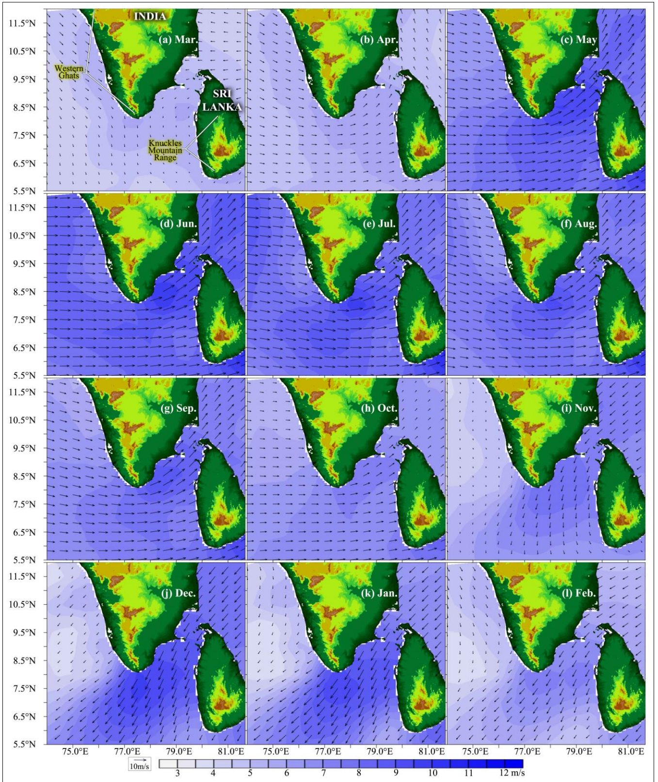
Figure 2 - Wind velocity ( \text{m s}^{-1} ) in the study domain and its variations associated with the seasonal evolution from the Pre-Monsoon (Mar.) to the Northeast Monsoon (Feb.). Strong winds are a characteristic feature of the GoM during the SWM (Jun. - Sep.) and NEM (Nov. - Feb.) periods.
