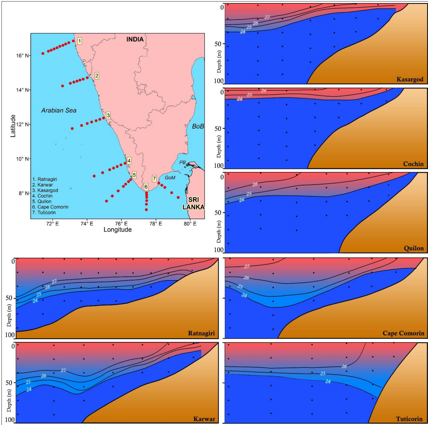
Supplementary Figure 1 - Vertical distribution of temperature along seven cross-shore transects along the central and southwest coast of India during the Southwest Monsoon. Clear signatures of upwelling as up-sloping of isotherms and stratified water column closer to the coast were evident in all transects except in the Tuticorin transect (Transect 7). Shoaling up of cold subsurface waters toward the coast was visible, except in the Tuticorin transect. In the Tuticorin transect, the surface water column in the nearshore waters was well mixed (deeper mixed layer) followed by a downwelling of isotherms in the subsurface waters representing the absence of upwelling process there (adapted from Johannsen et al., 1981)
