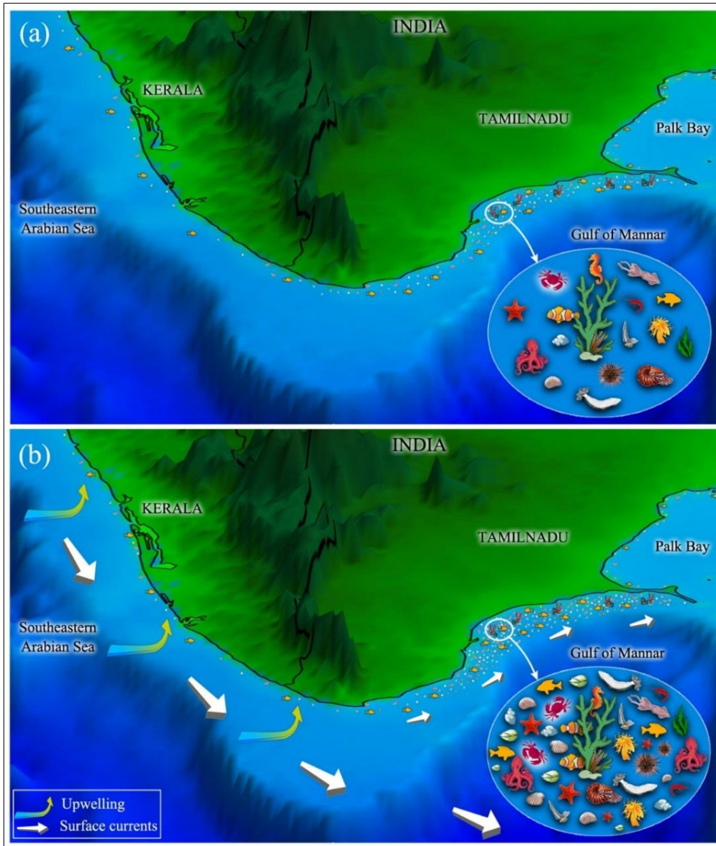
Figure 11 - Schematic of the seasonal scenario of faunal diversity and richness in the GoM during (a) non-upwelling and (b) upwelling periods. The geographically sheltered environment in the GoM provides conducive environmental conditions to support high faunal richness and diversity compared to its adjacent region. The hypoxia avoidance mechanism of fauna from the Indian southwestern shelf during the upwelling period cause their high concentration in the GoM.
