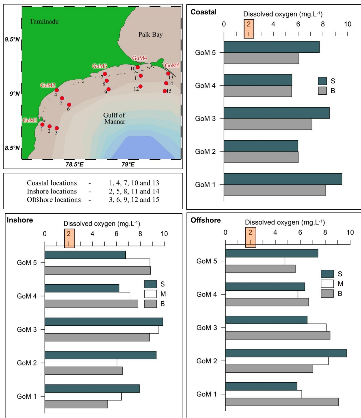
Figure 7 - The vertical distribution of dissolved oxygen in five cross-shore transects along the Indian shelf in the GoM during the Southwest Monsoon (September 2010). The oxygen concentration in the (S) surface, (M) middle, and (B) bottom depths in each sampling location are presented. The hypoxic levels (<2mg L -1 ) is indicated on the x-axis as a pink bar to show the significantly oxygenated water that prevails in the GoM during the Southwest Monsoon
