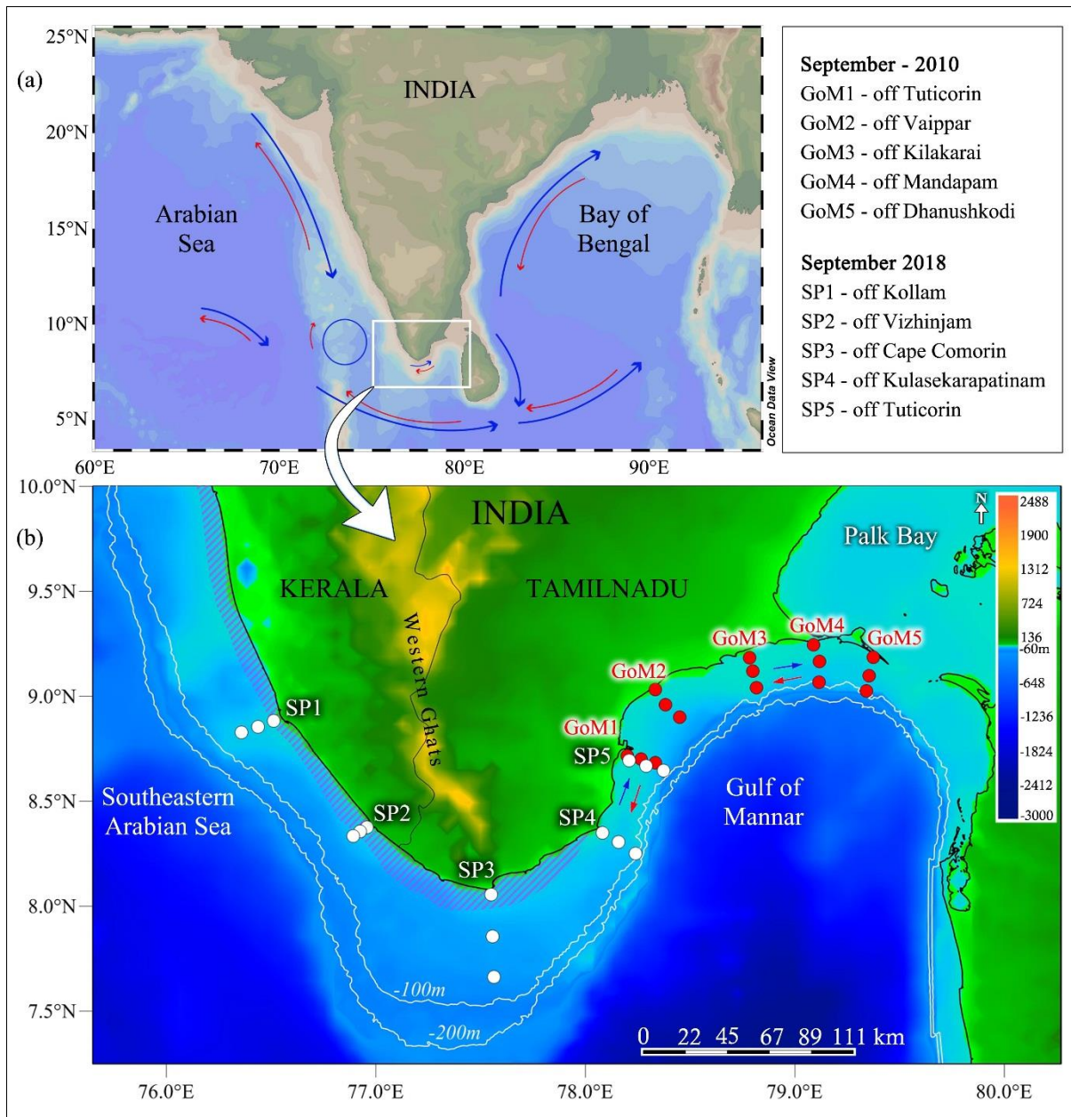
Figure 1 - (a) Study domain showing the GoM and the SEAS. (b) Sampling transects in the study domain. Five cross-shore transects (red filled circles, GoM1 to GoM5) sampled in the GoM during the 2010 - 2011 period and five cross-shore transects (white filled circle, SP1 to SP5) in the Indian shelf waters along the southwest coast of India up to the western boundary of the GoM sampled in 2018. The zone of coastal upwelling along the southwest coast of India is shown as hatched oblique blue lines close to the coastline in panel (b). The seasonally reversing ocean surface currents in the GoM is represented in both panels (a) and (b); blue arrows represent the Southwest Monsoon (June - September) while the red the Northeast Monsoon (November - February).
