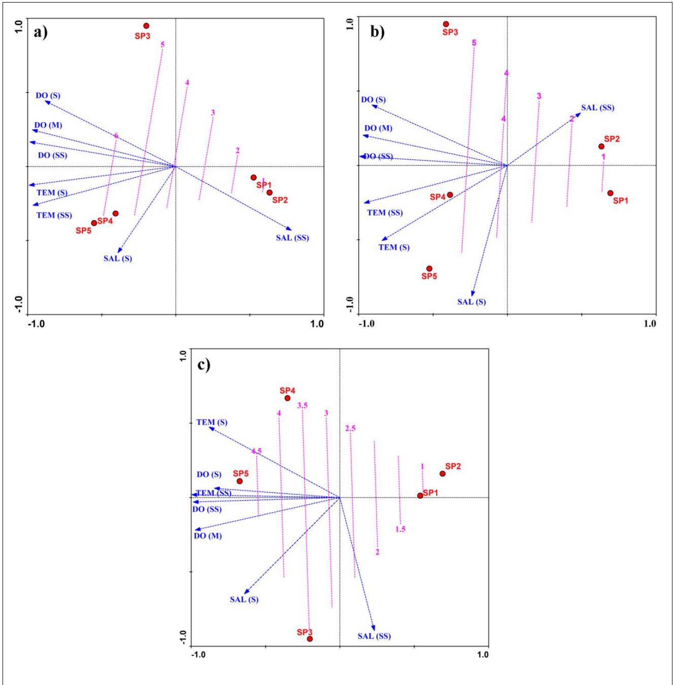
Figure 9 - Principal Component Analysis (first two axes - PC1 and PC2) biplot representing the hydrographical variables (blue dotted lines) and their relatedness in (a) 10m, (b) 25m and (c) 40m depths of SP1 to SP5 transects. The attribution plot (GLM model) of the dissolved oxygen values (pink dotted lines) were overlaid on the PCA 2D plot. The attribution model represents the variations of dissolved oxygen concentration between various transects. PCA plots show that the hydrographical conditions in SP1 and SP2 have a significant difference between SP4 and SP5. The SP4 and SP5 in the vicinity of the GoM had relatively warm and oxygenated waters compared to SP1 and SP2. Abbreviations: SAL - Salinity; TEM - Temperature; DO - Dissolved Oxygen. S - Surface; SS - Subsurface; M -Middle (5m in 10m location; 10m in 25m location; 20m in 40m location).
