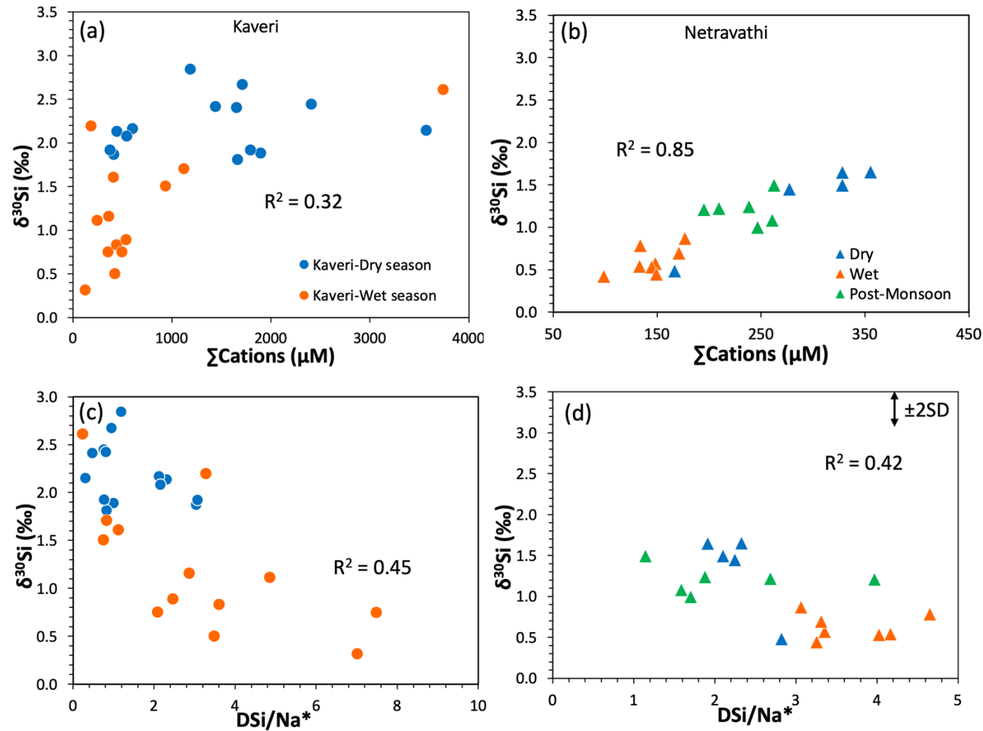
Figure S1. Linear relationship between \delta^{30}\text{Si}_{\text{DSi}} and total cations ( \Sigma\text{C}^{+*} , atmospheric input corrected) (a, b) and \text{DSi}/\text{Na}^* (c, d) for both Kaveri and Netravathi. (blue indicate dry and orange indicate wet and the green in Netravathi indicate post monsoon).
