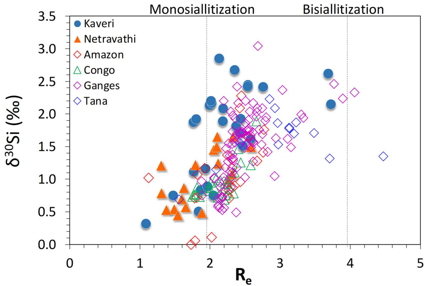
Fig. 6. \delta^{30}\text{Si}_{\text{DSi}} and R_e of the present study compared with the values from other studies global river water (see text for details).
