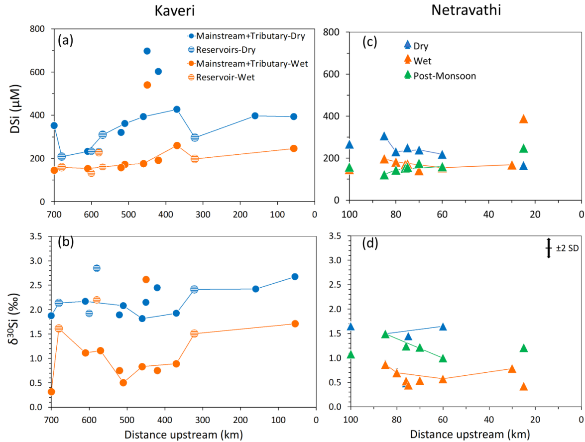
Fig. 2. Spatial and seasonal variability of dissolved Si (DSi) and silicon isotopes of DSi ( \delta^{30}\text{Si}_{\text{DSi}} ) in the Kaveri (2a, 2b) and Netravathi (2c, 2d) river basins during dry (blue) and wet (orange) periods. Post-monsoon data is available also for Netravathi (green). Water flow is from left to right. The filled circles in Kaveri represent the mainstream and tributaries, and the circle with patterns represent the dams/reservoir (Table 1 for more details). The samples along the mainstream are connected.
