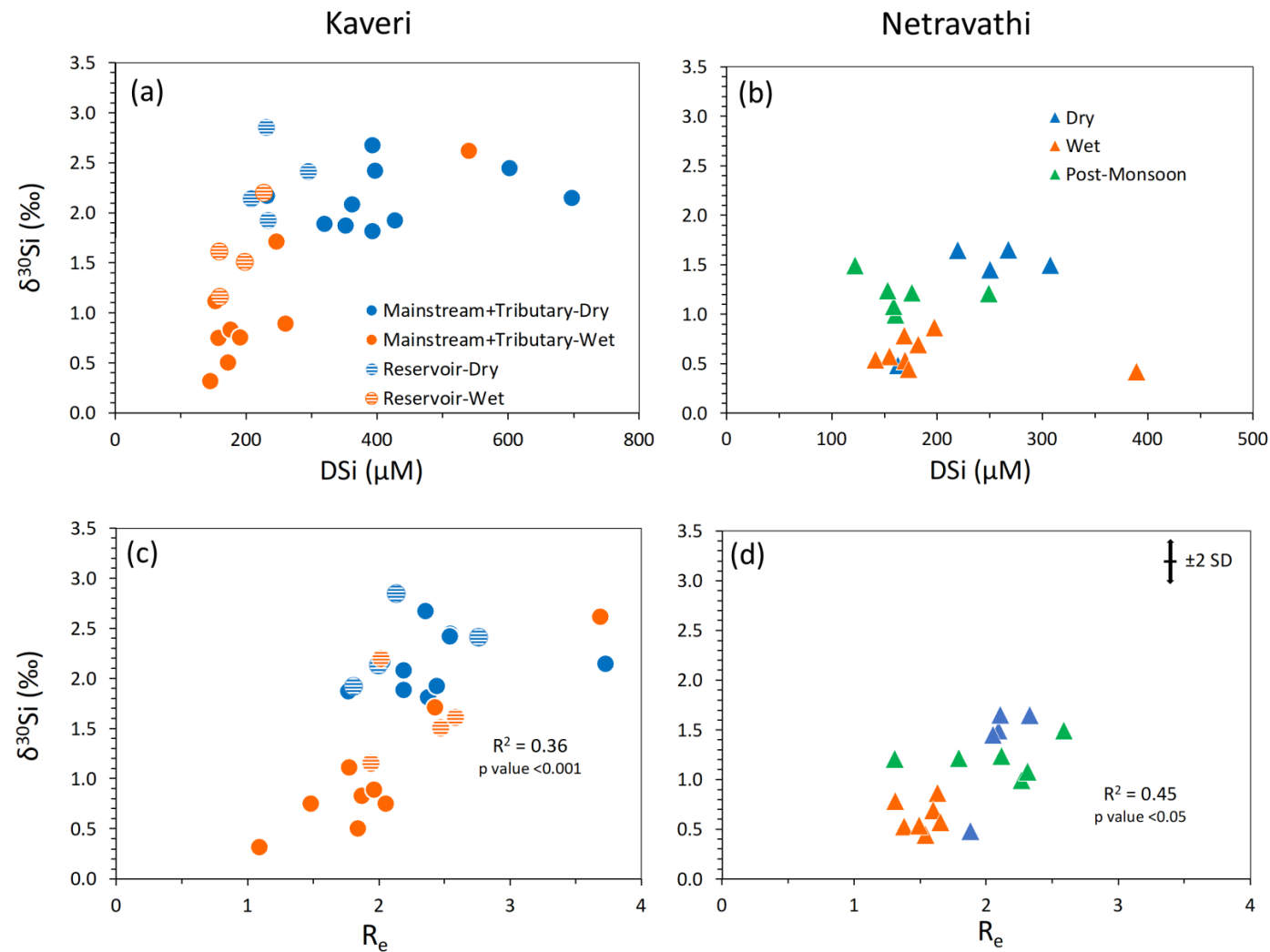
Fig. 3. Evolution of the isotopic signature ( \delta^{30}\text{Si}_{\text{DSi}} ) in the river Kaveri and Netravathi during different seasons, with dissolved Si concentration (3a, 3b) and R_e (3c, 3d).
