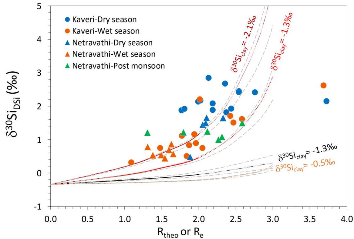
Figure 5. The evolution of R_{\text{theo}} and \delta^{30}\text{Si}_{\text{DSi}} as rock weathers and transforms into secondary products plotted along with measured R_e of river water samples from Kaveri and Netravathi. Trendline for three different silicon isotopic composition for the clay is plotted for the gneiss weathering corrected for quartz and sericite contribution (maroon, red and orange for \delta^{30}\text{Si}_{\text{product}} values of -2.1\text{‰} , -1.3\text{‰} and -0.5\text{‰} respectively). The scenario for whole gneiss weathering and \delta^{30}\text{Si}_{\text{product}} of -1.3\text{‰} is shown in black. The grey dashes lines represent the sensitivity depending on the deviation in the chemical composition in the initial rock composition (Braun et al., 2009)
