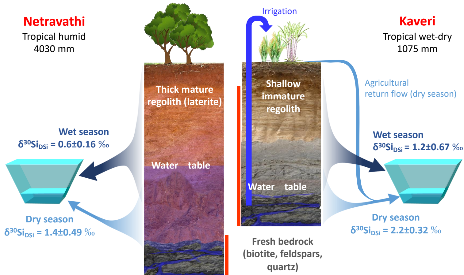
Fig. 4. A schematic of the results from the current study comparing the silicon cycling from two contrasting watersheds in South India. Red bars refer to the section of weathering profile where cation bearing ( \text{Na}^+ , \text{K}^+ , etc.) primary minerals are still present and are leached. Please note that the weathering profile given is just a representative for middle/lower reaches of Kaveri, the humid high elevation profile in Western Ghats is similar to Netravathi (Deepthy and Balakrishnan 2005, Braun et al., 2009, Gurumurthy et al., 2012, Meunier et al., 2015).
