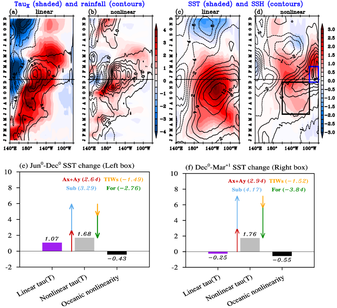
Figure 5. Composite life-cycle of anomalies attributable to the linear and nonlinear wind stress response to SST anomalies during extreme El Niño events. Longitude-time section of equatorial (5°N-5°S) average (a) linear and (b) nonlinear zonal wind stress (shaded, 10^{-2} \text{ Nm}^{-2} ) and rainfall (contours, mm/day) response to SST anomalies; and SST (shaded, °C) and SSH (contours, cm) anomalous responses to the (c) linear (linear \tau(\text{SST}) experiment) and (d) nonlinear (nonlinear \tau(\text{SST}) experiment) components of the wind stress. The left (black, 100 to 160°W, 5°N to 5°S) and right (blue, 90 to 100°W, 5°N to 5°S) boxes on panel (d) respectively indicate the regions and periods over which the spatially averaged and temporally integrated heat budgets of panels (e) and (f) are performed. Those budgets indicate the total contribution of the linear (purple) and nonlinear (grey) wind stress and the oceanic nonlinearities (black) to the SST change (i.e. SST anomalies at the end minus those at the beginning of the period). The contribution of the nonlinear wind stress to the SST change is further broken into lateral advection (red), subsurface processes (blue), air-sea fluxes (green) and Tropical Instability Waves (yellow). Panel (e) focuses on the central and eastern Pacific warming in the 6 months that precede the El Niño peak (i.e. 1 st June 1997 to 1 st December 1997, see black box on panel d) and panel (f) on the prolonged eastern Pacific warming during the 4 months that follow the El Niño peak (i.e. 1 st December 1997 to 1 st April 1997, see black box on panel d). Panels (a, b) are obtained from the ensemble AGCM experiments and c - f from the OGCM experiments described in the text.
