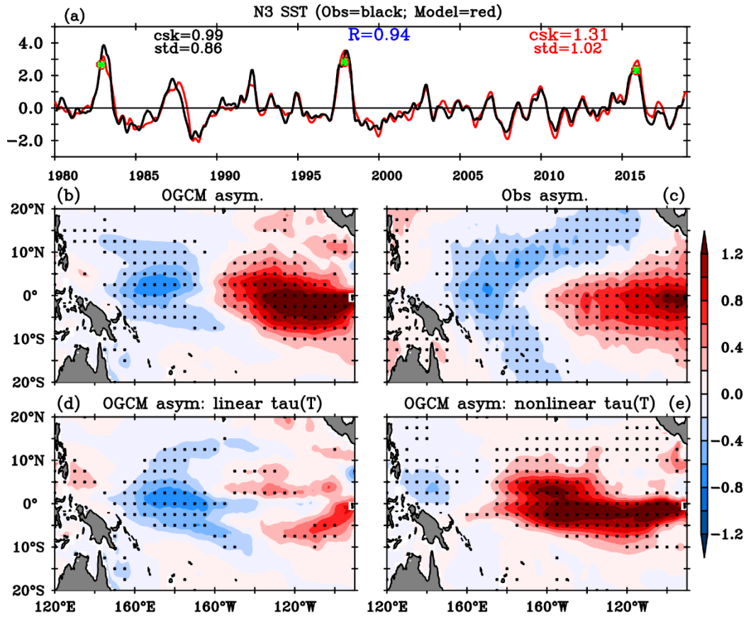
Figure 3. (a) Time series of the average Niño3 (5°N-5°S, 150°W-90°W) SST anomalies for the control OGCM simulation (red curve) and observations (black curve). (b) DJF average ENSO SST asymmetries (shaded, °C, obtained as the half sum of extreme El Niño and strong La Niña composites, see text for details) in the OGCM control simulation, and contributions from the (d) linear and (e) nonlinear wind stress response to SST. See the text for details on the ocean model experiments that yield (d) and (e). Panel (c) is the same as (b) but for observations. The statistical quantities on panel (a) show standard deviation (std), coefficient of skewness (csk) and correlation coefficient (R) values. Stippling on (b) – (e) indicates asymmetry that is different from zero at the 95% confidence level based on a t-test.
