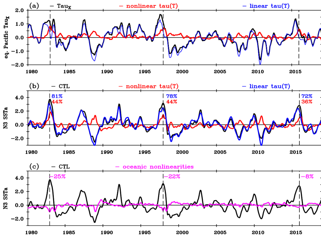
Figure 4. Interannual time series of (a) equatorial Pacific ( 5^{\circ}\text{N} - 5^{\circ}\text{S} , 120^{\circ}\text{E} - 80^{\circ}\text{W} ) averaged zonal wind stress anomalies ( 10^{-2} \text{ Nm}^{-2} ) with contributions from the linear (blue curve) and nonlinear (red curve) components of the response to SST. Niño3 SST anomalies ( ^{\circ}\text{C} ) from (b) the control OGCM simulation (black), and contributions from the linear (blue, linear \tau(\text{SST}) experiment) and nonlinear (red, nonlinear \tau(\text{SST}) experiment) wind stress response to SST, (c) the control OGCM (black) and the contribution from oceanic nonlinearities (magenta curve, obtained as the control minus the sum of the linear and nonlinear \tau(\text{SST}) experiments). The vertical dashed lines mark the peak of the three extreme El Niño events in December 1982, 1997 and 2015. The numbers indicate the percentage of the contributions of the linear (blue), nonlinear (red) wind stress components and of oceanic nonlinearities (magenta) to the total November-January Niño3 SST anomalies during these three events (see supplementary Table S1 for details). The average contribution over the three extreme El Niño events is 77% for linear \tau(\text{SST}) , 41% for nonlinear \tau(\text{SST}) , and -18% for oceanic nonlinearities.
