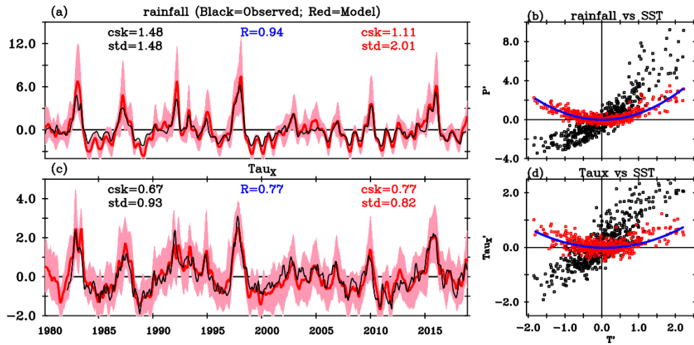
Figure 1. (a) Time series of interannual anomalies of precipitation (mm/day) averaged over the Niño3+4 region (160°E-90°W, 5°N-5°S) for the control AGCM simulation (red curve) and observations (black curve). The red shading represents the ensemble spread of the control AGCM simulation (10 th and 90 th percentiles). (b) Scatter diagram of simulated anomalous rainfall response to SST anomalies over the Niño3+4 region (black dots) with its nonlinear contribution (red dots, see methods for details). The blue curve is a quadratic fit of the atmospheric nonlinear response to SST anomalies. (c, d) Same as (a, b) but for zonal wind-stress anomalies (10 -2 Nm -2 ). The standard deviation (std) and coefficient of skewness (csk) are indicated (AGCM ensemble mean in red, observations in black), as well as the correlation (R) between the AGCM ensemble mean and observed time series.
