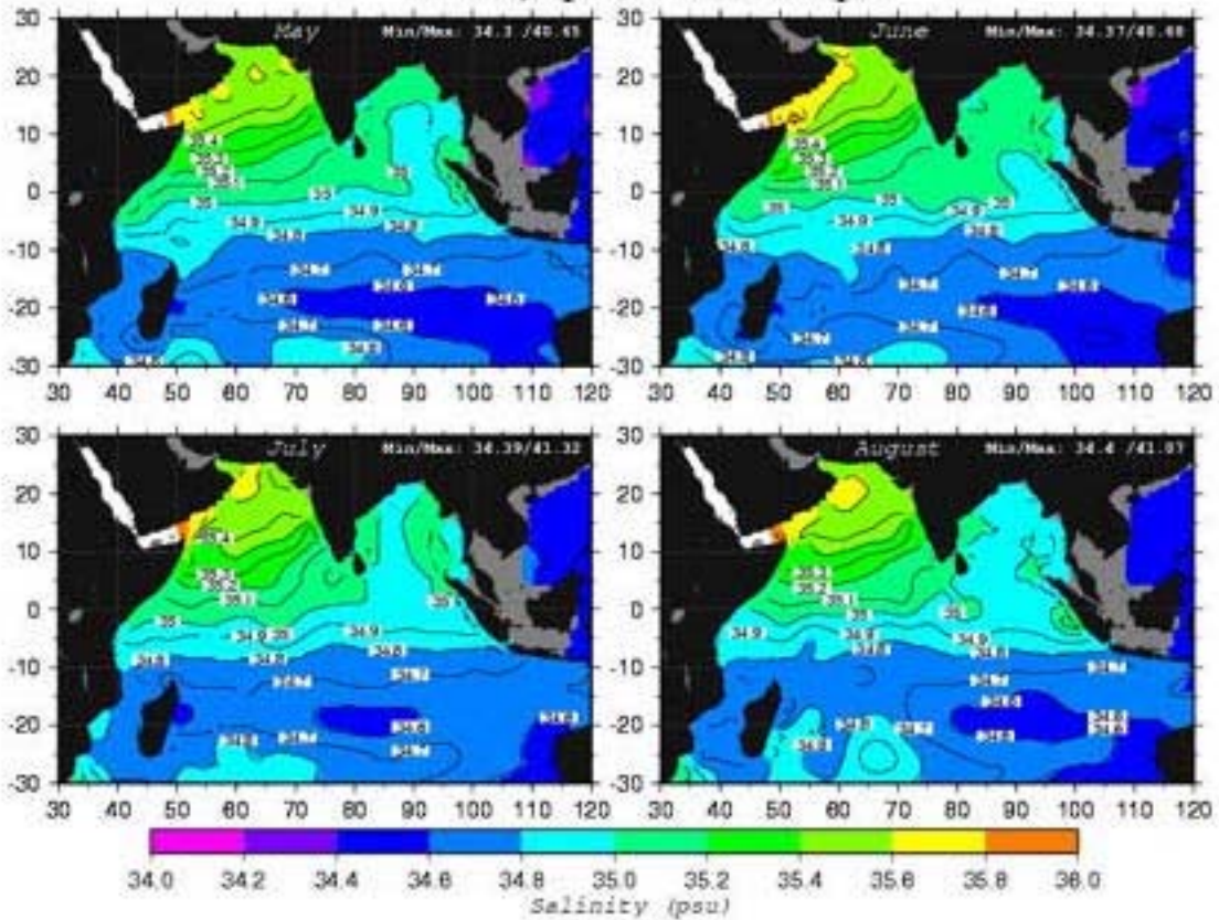
Salinity (psu) at 700 m depth
