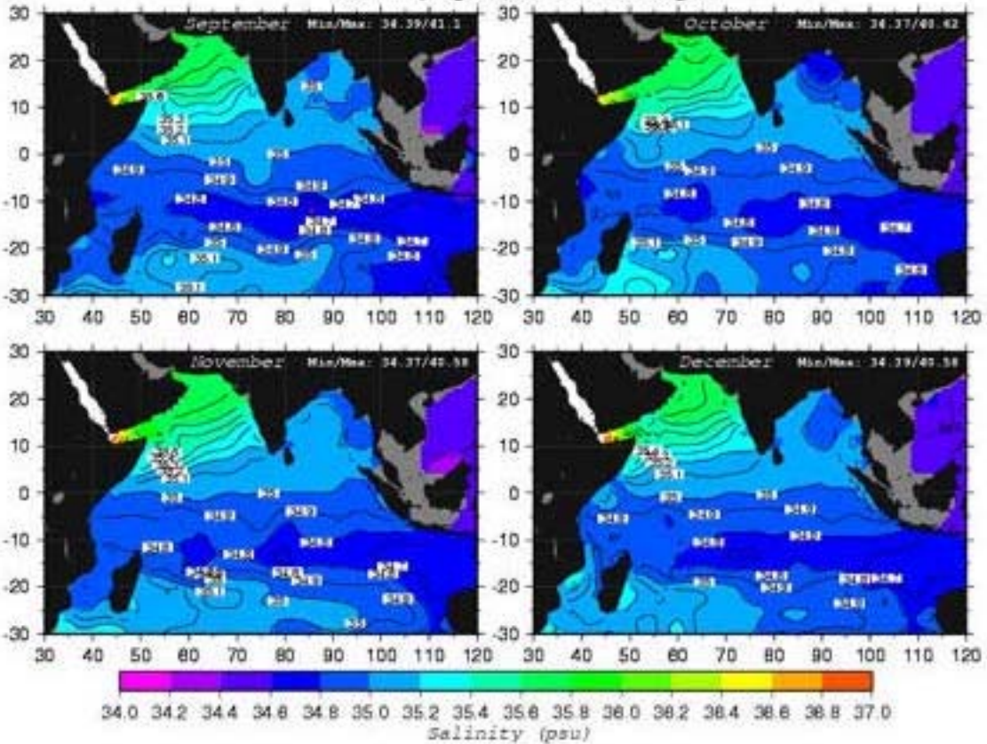
Salinity (psu) at 500 m depth
