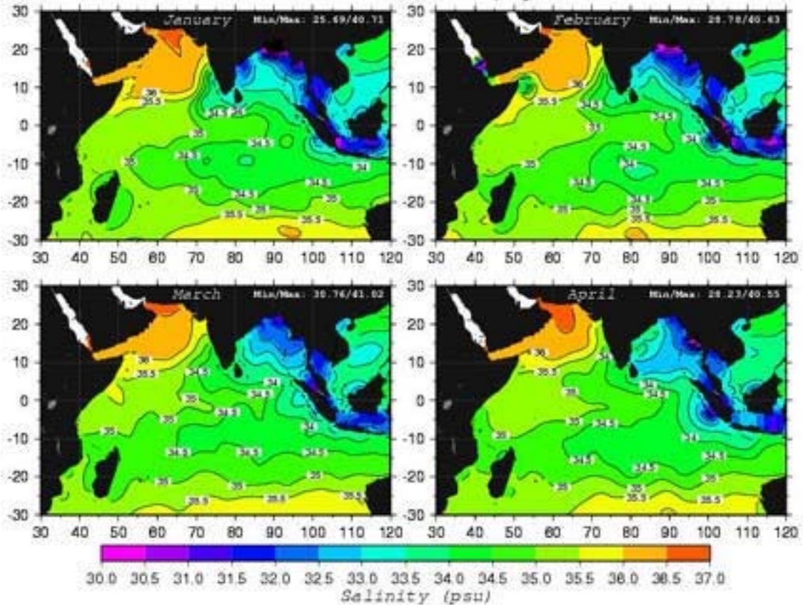
Sea Surface Salinity (psu)
