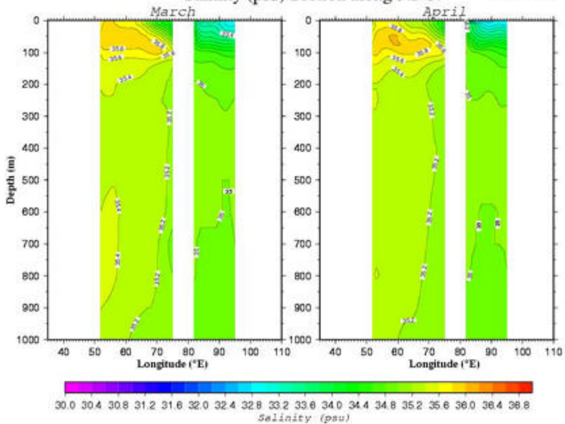
Salinity (psu) Section along 9.5°N
