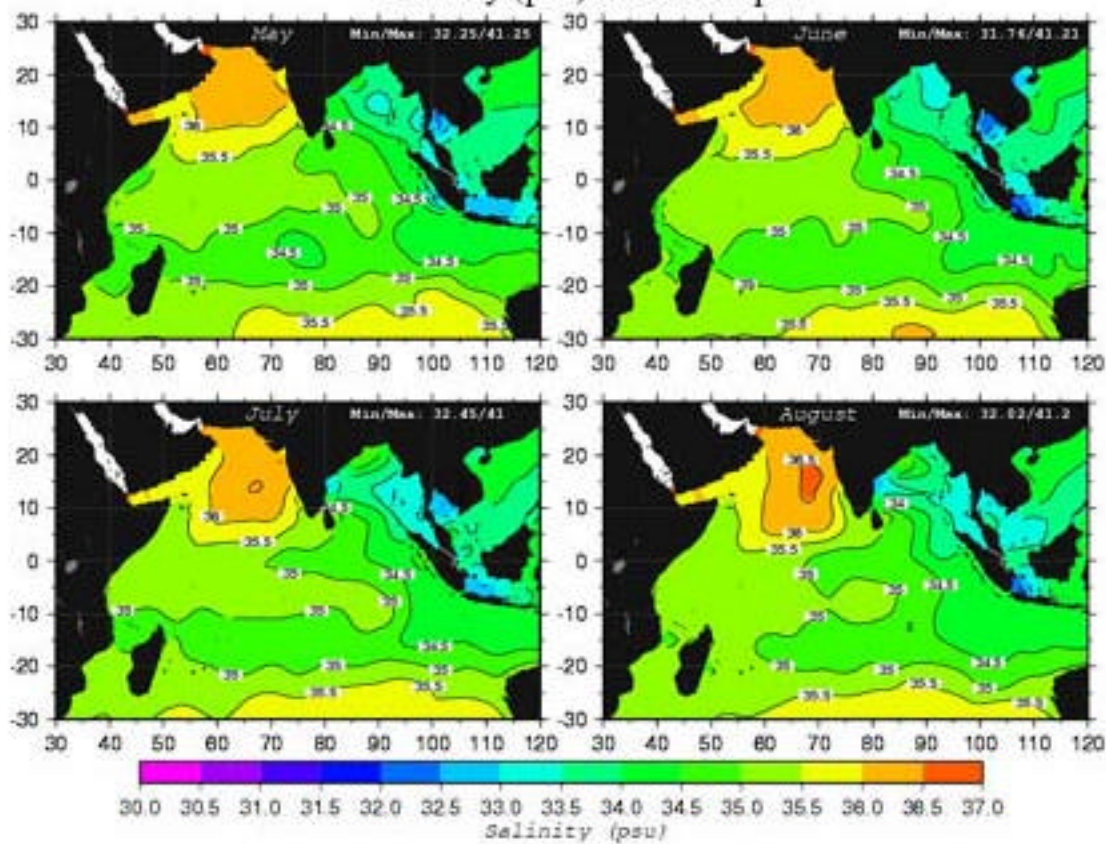
Salinity (psu) at 50 m depth
