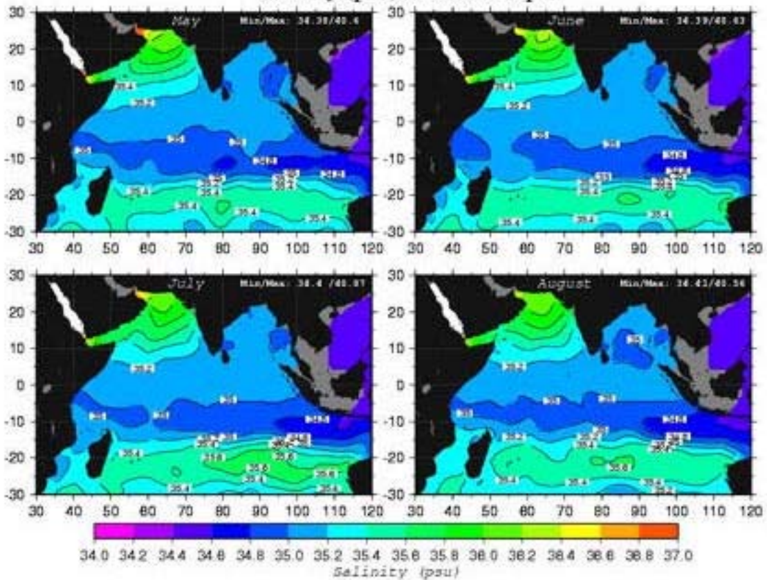
Salinity (psu) at 300 m depth
