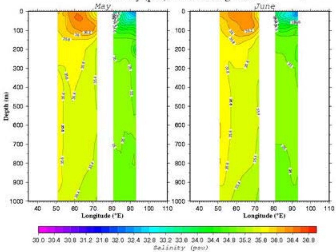
Salinity (psu) Section along 14.5°N
