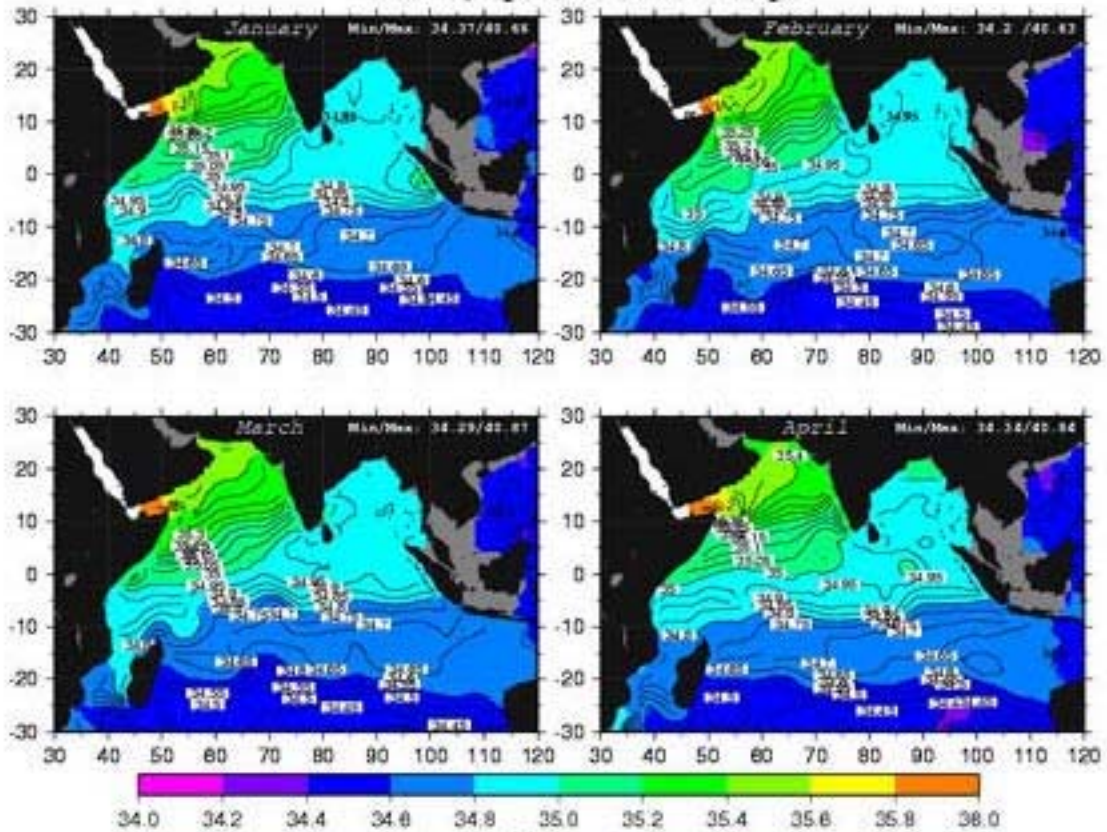
Salinity (psu) at 1000 m depth
