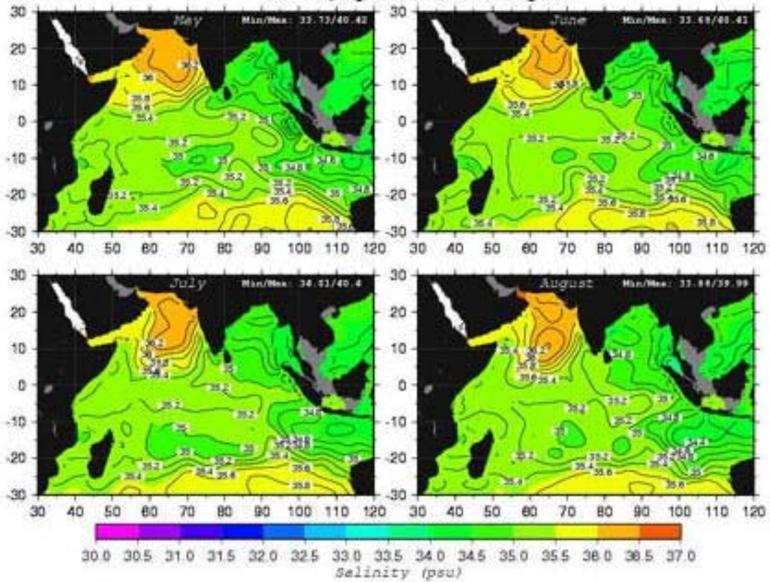
Salinity (psu) at 100 m depth
