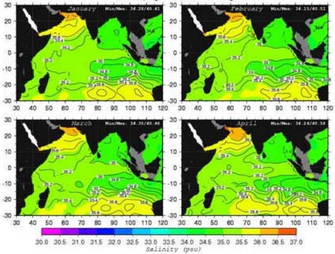
Salinity (psu) at 150 m depth
