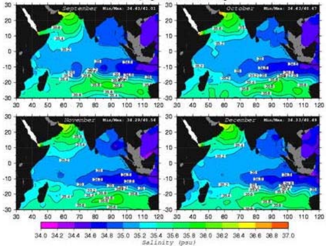
Salinity (psu) at 200 m depth
