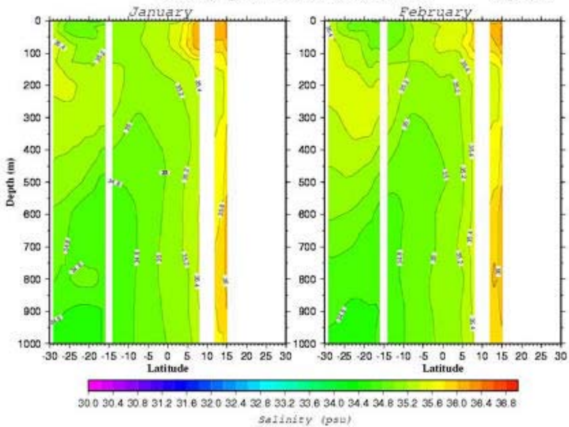
Salinity (psu) Section along 50.5°E
