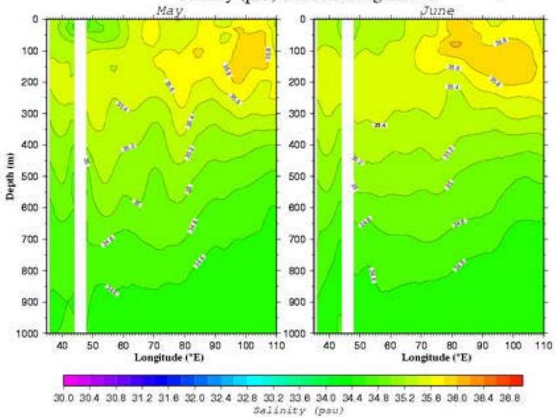
Salinity (psu) Section along 25.5°S
