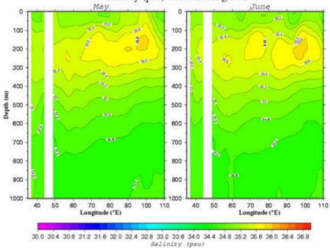
Salinity (psu) Section along 20.5°S
