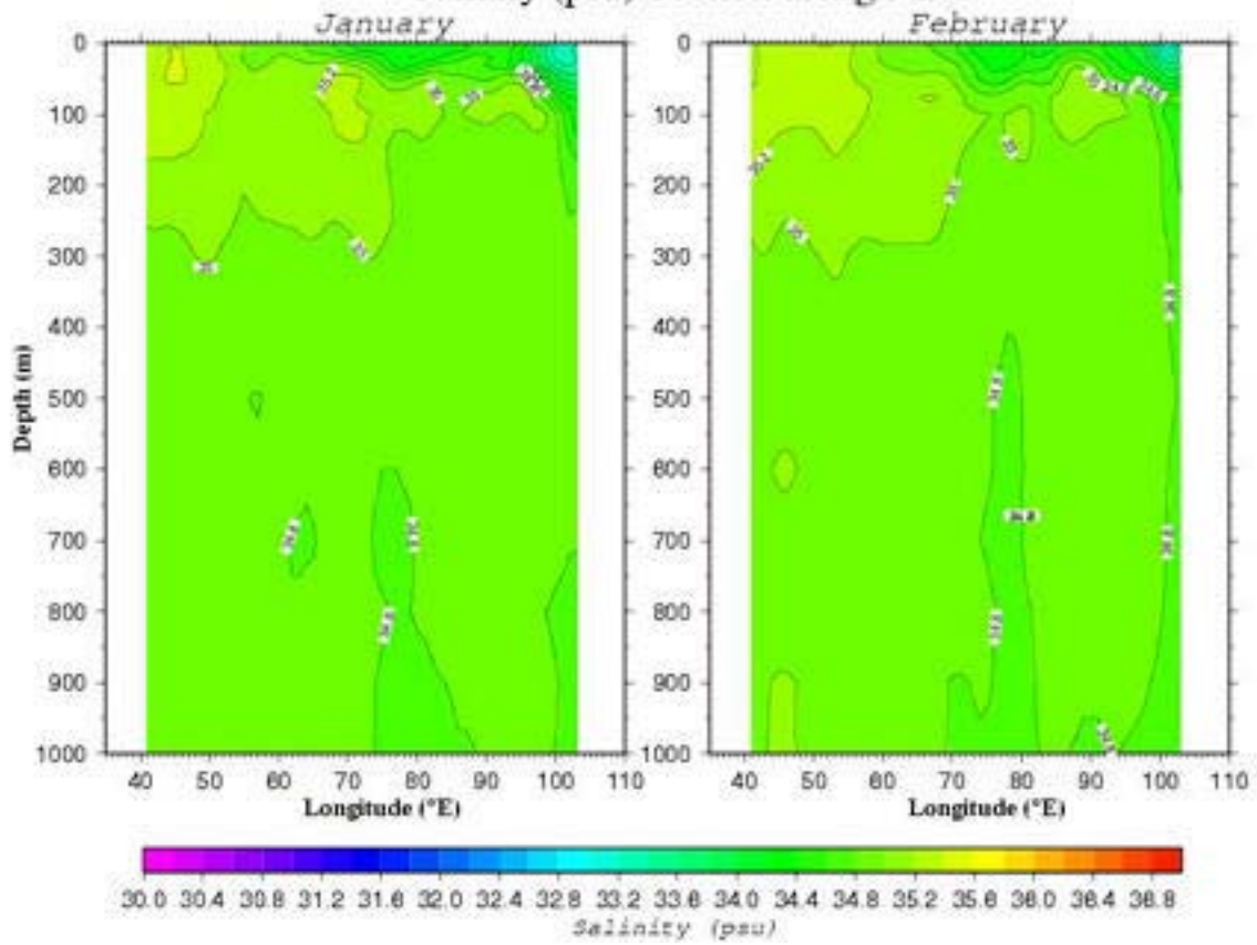
Salinity (psu) Section along 5.5°S
