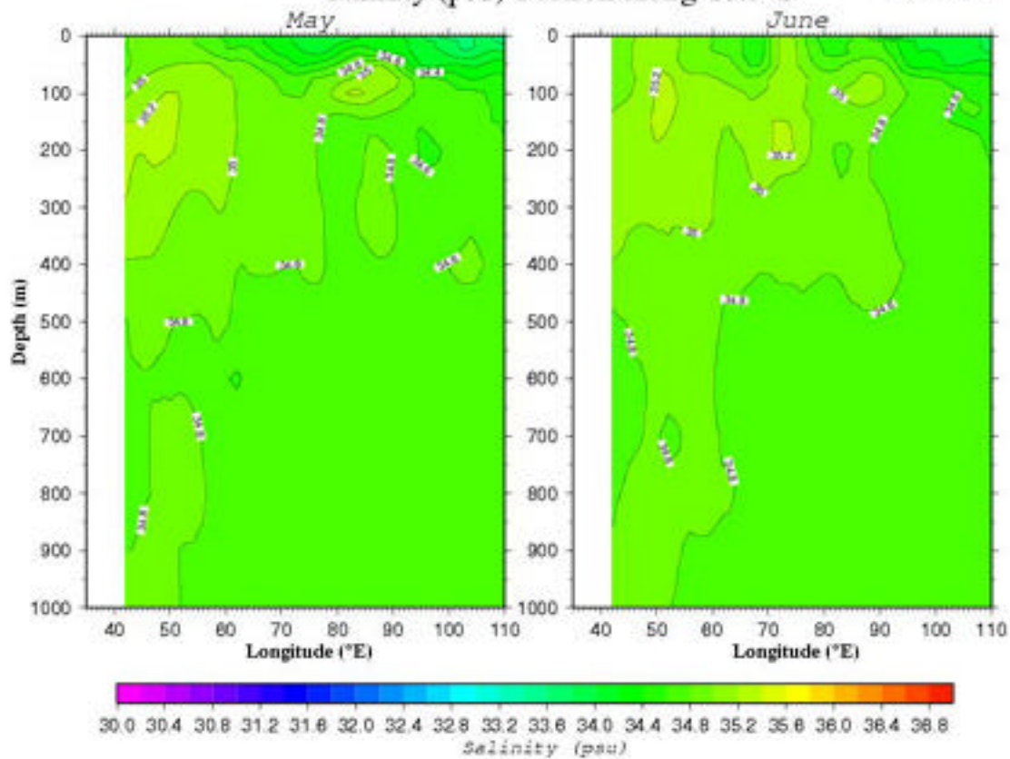
Salinity (psu) Section along 10.5°S
