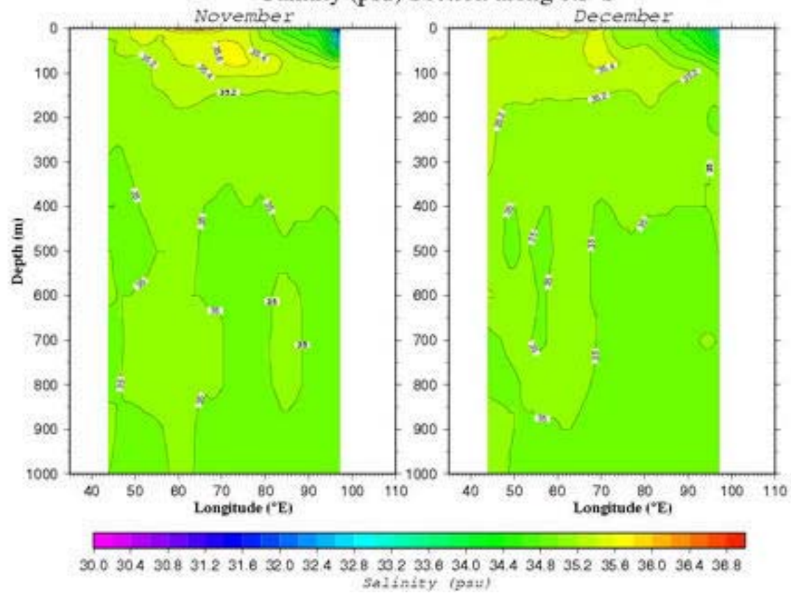
Salinity (psu) Section along 0.5°S
