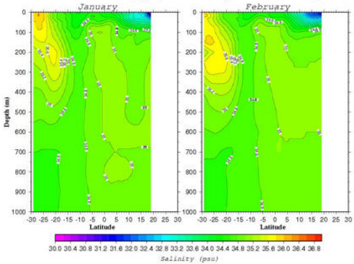
Salinity (psu) Section along 90.5°E
