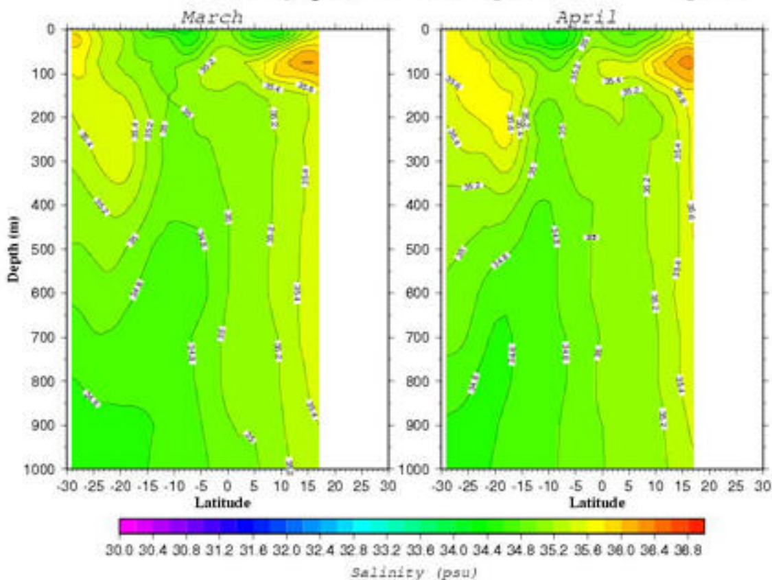
Salinity (psu) Section along 70.5°E
