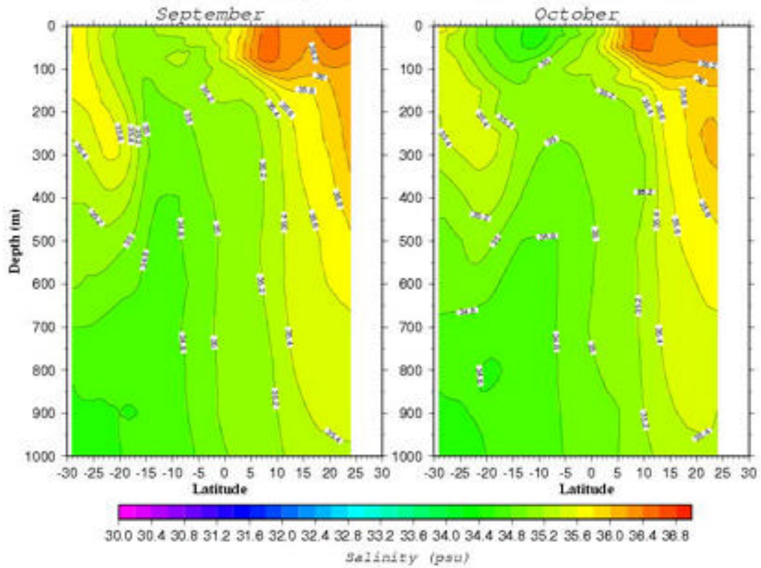
Salinity (psu) Section along 65.5°E
