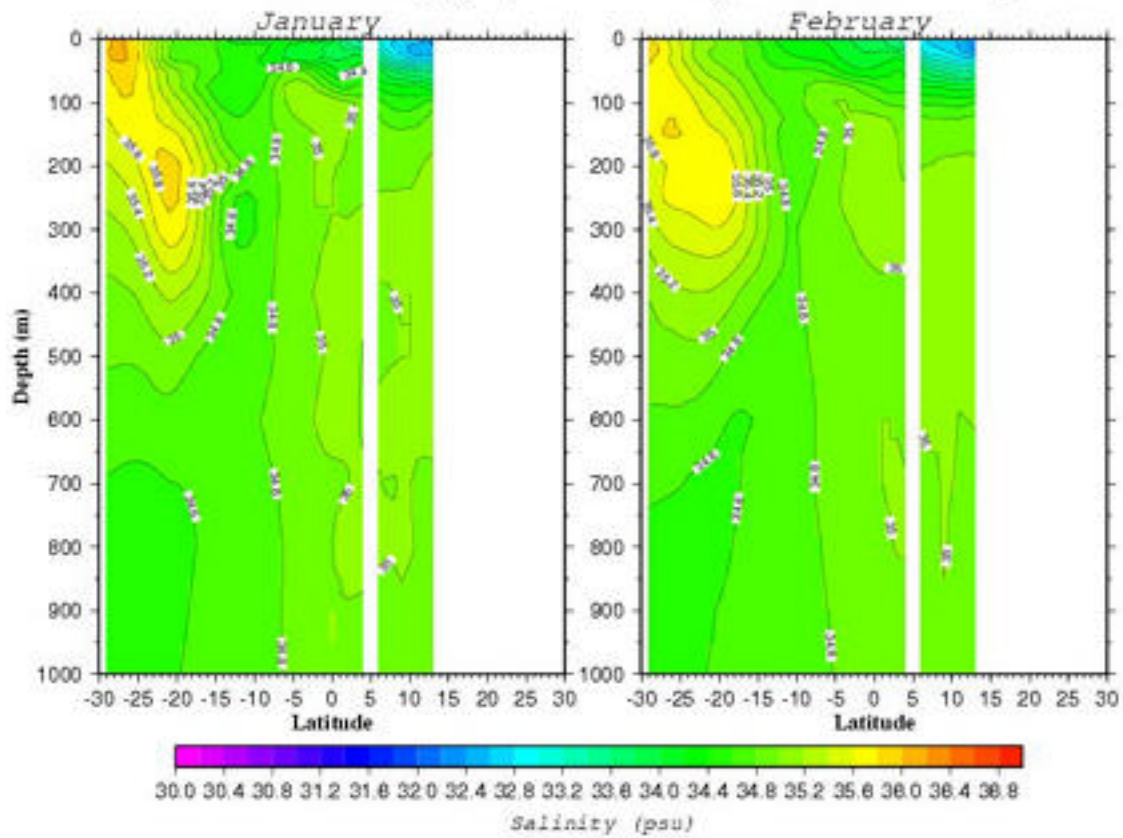
Salinity (psu) Section along 95.5°E
