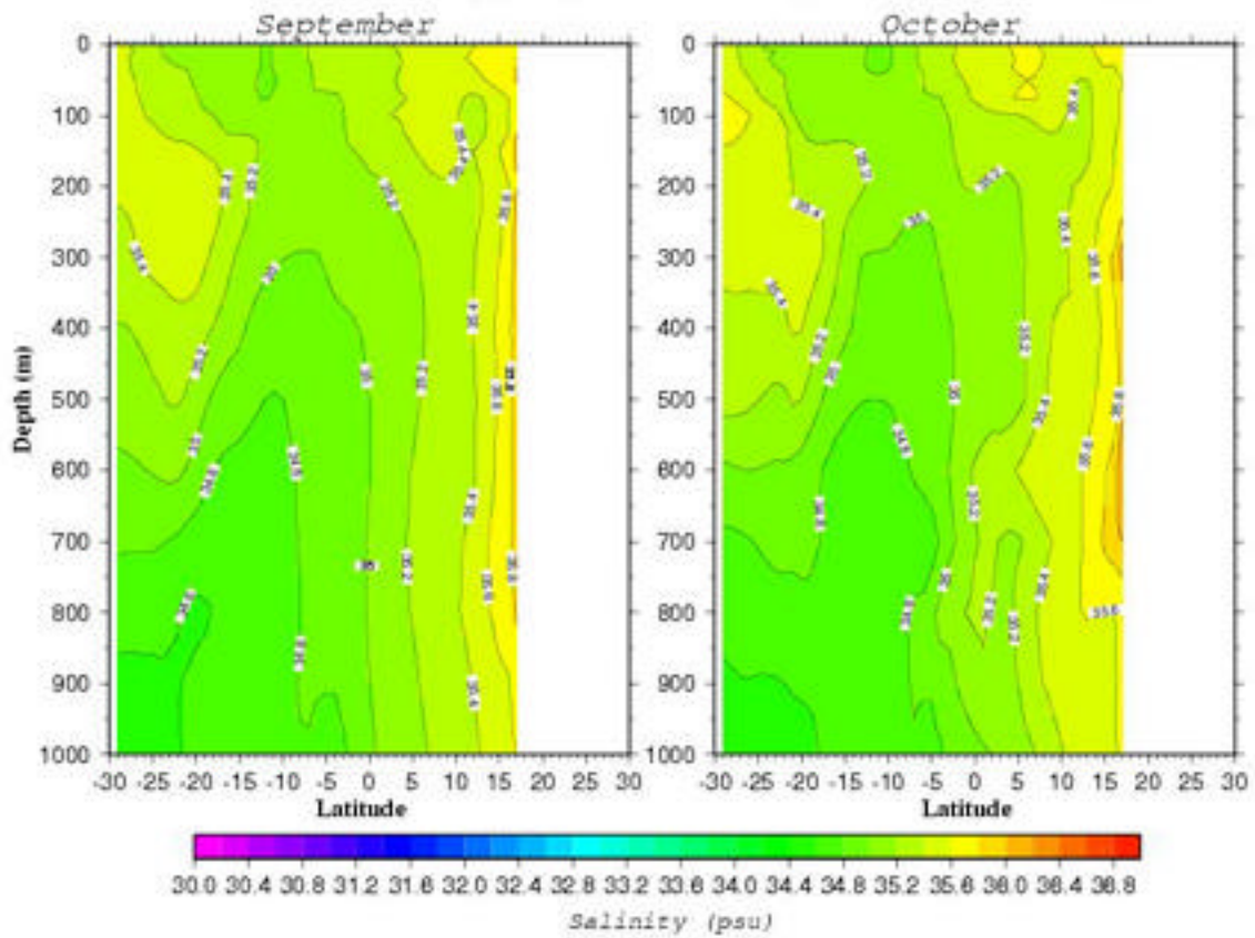
Salinity (psu) Section along 55.5°E
