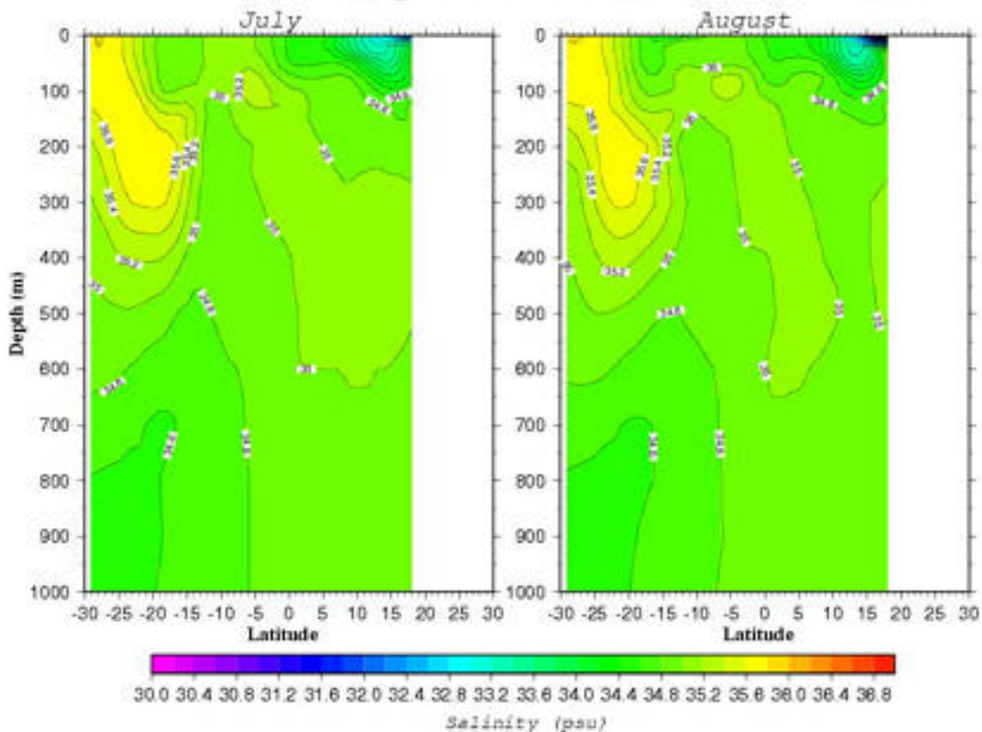
Salinity (psu) Section along 85.5°E
