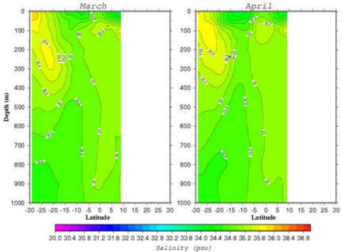
Salinity (psu) Section along 75.5°E
