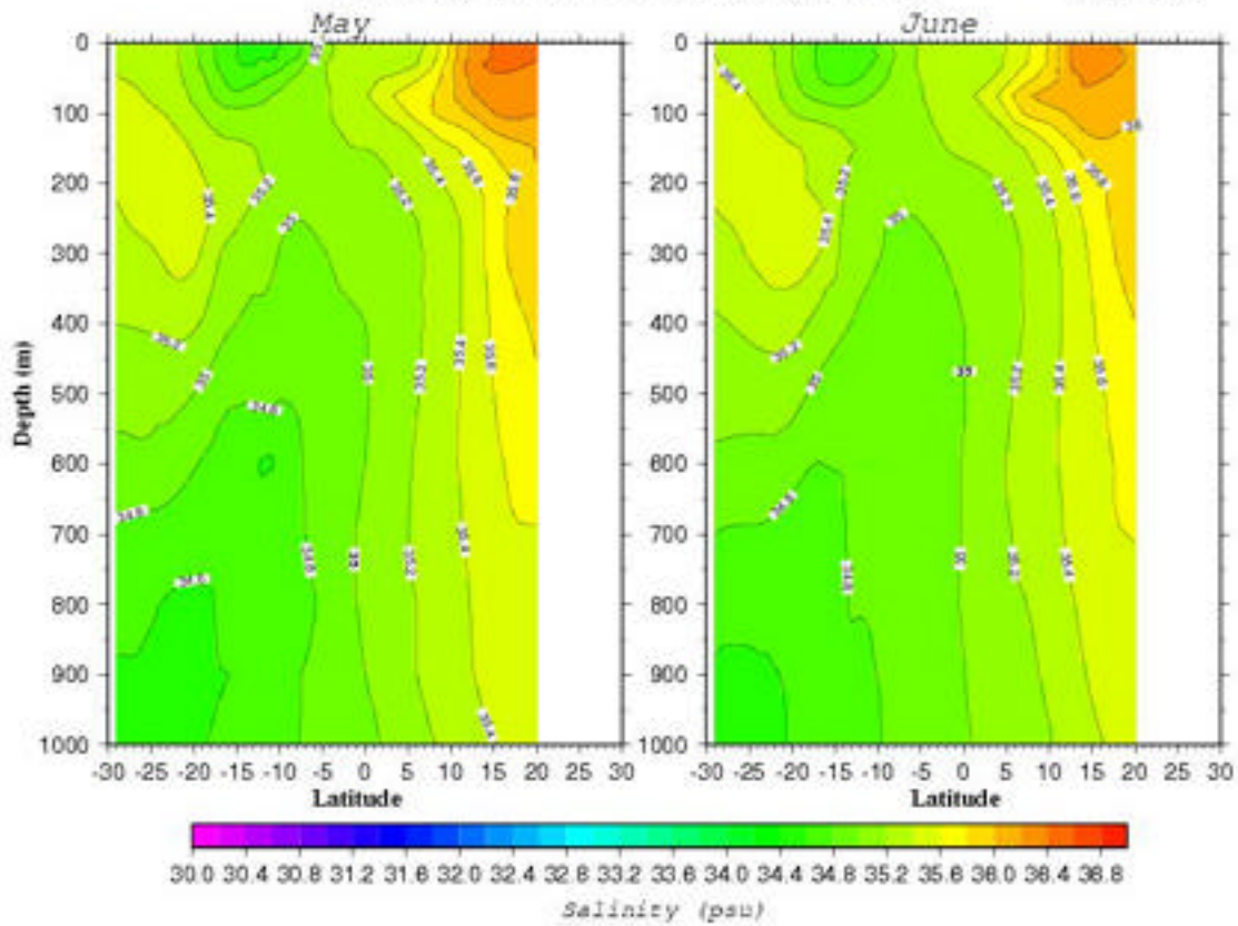
Salinity (psu) Section along 60.5°E
