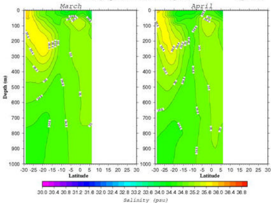
Salinity (psu) Section along 80.5°E
