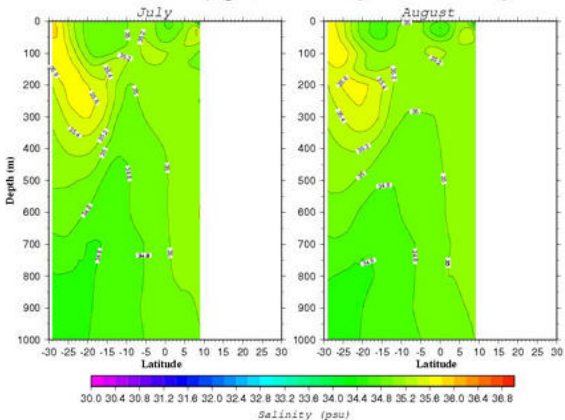
Salinity (psu) Section along 75.5°E
