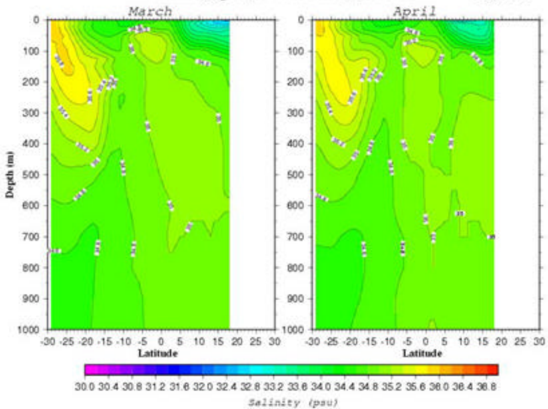
Salinity (psu) Section along 85.5°E
