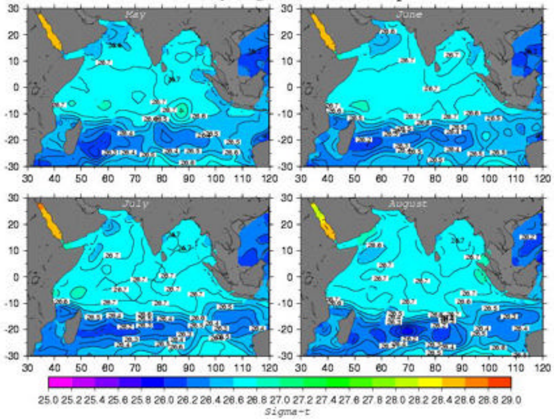
Density (Sigma-t) at 300 m depth
