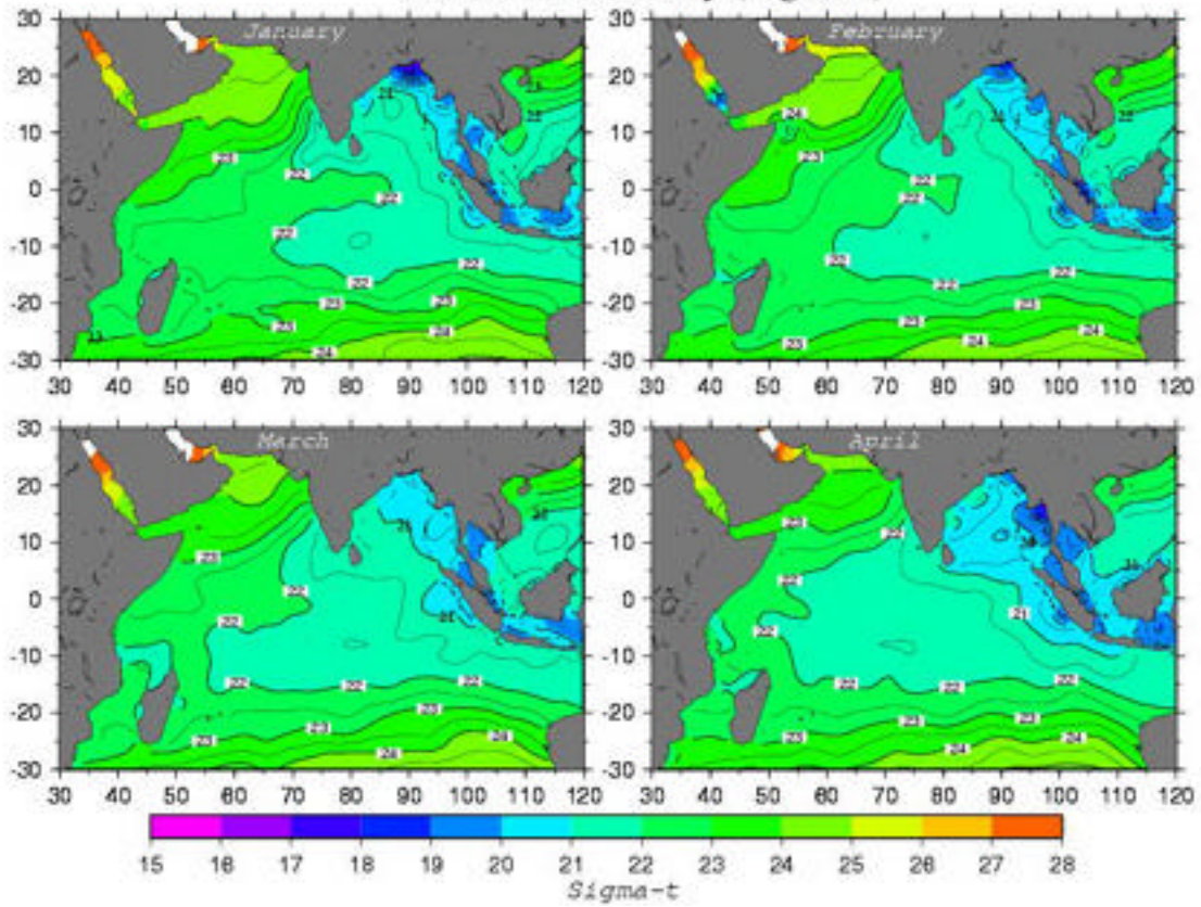
Sea Surface Density (Sigma-t)
