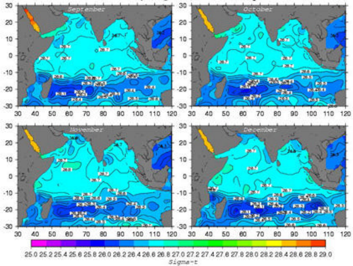
Density (Sigma-t) at 300 m depth
