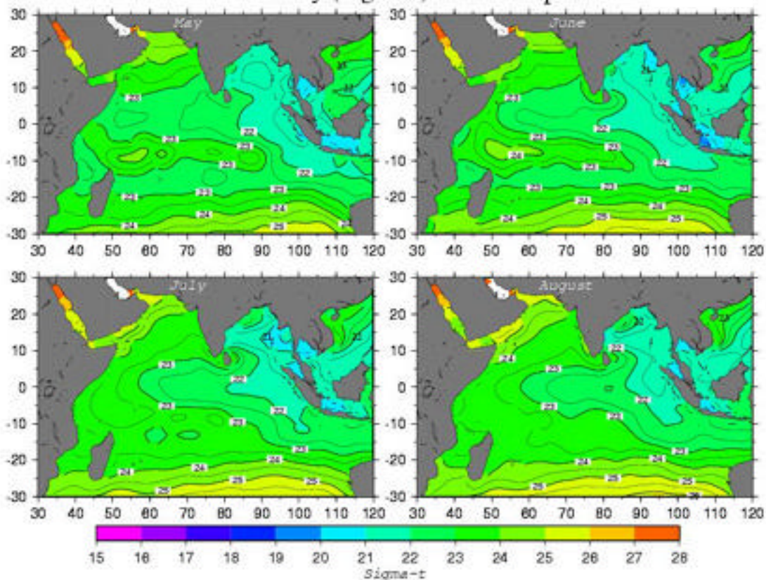
Density (Sigma-t) at 50 m depth
