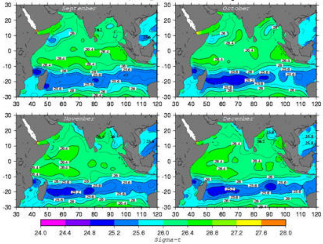
Density (Sigma-t) at 200 m depth
