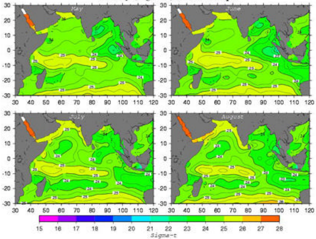
Density (Sigma-t) at 100 m depth
