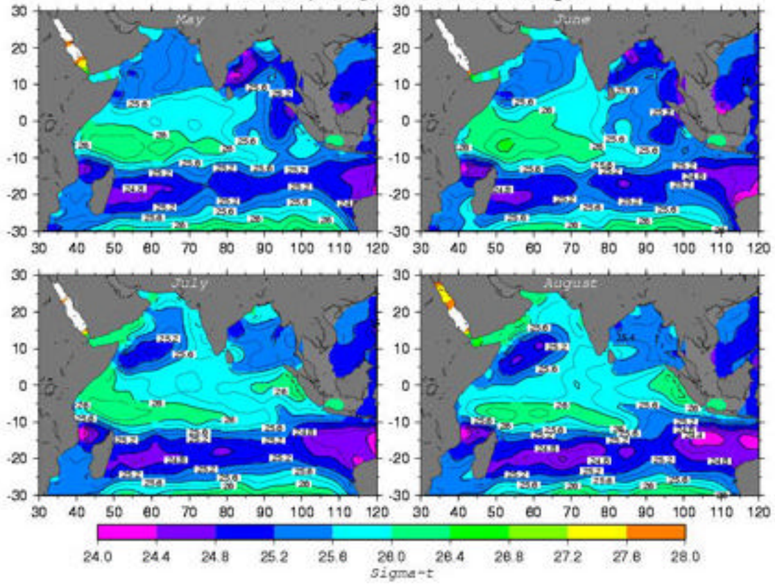
Density (Sigma-t) at 150 m depth
