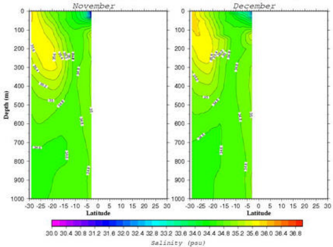
Salinity (psu) Section along 100.5°E
