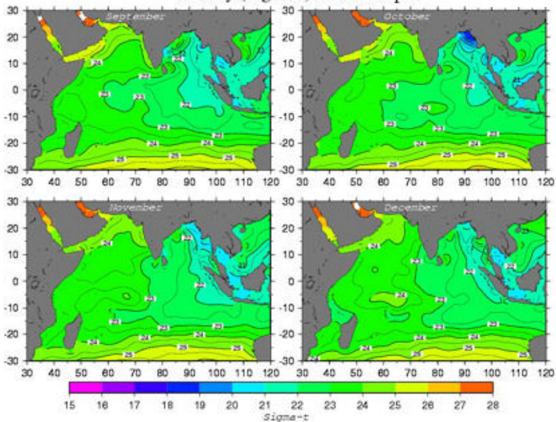
Density (Sigma-t) at 50 m depth
