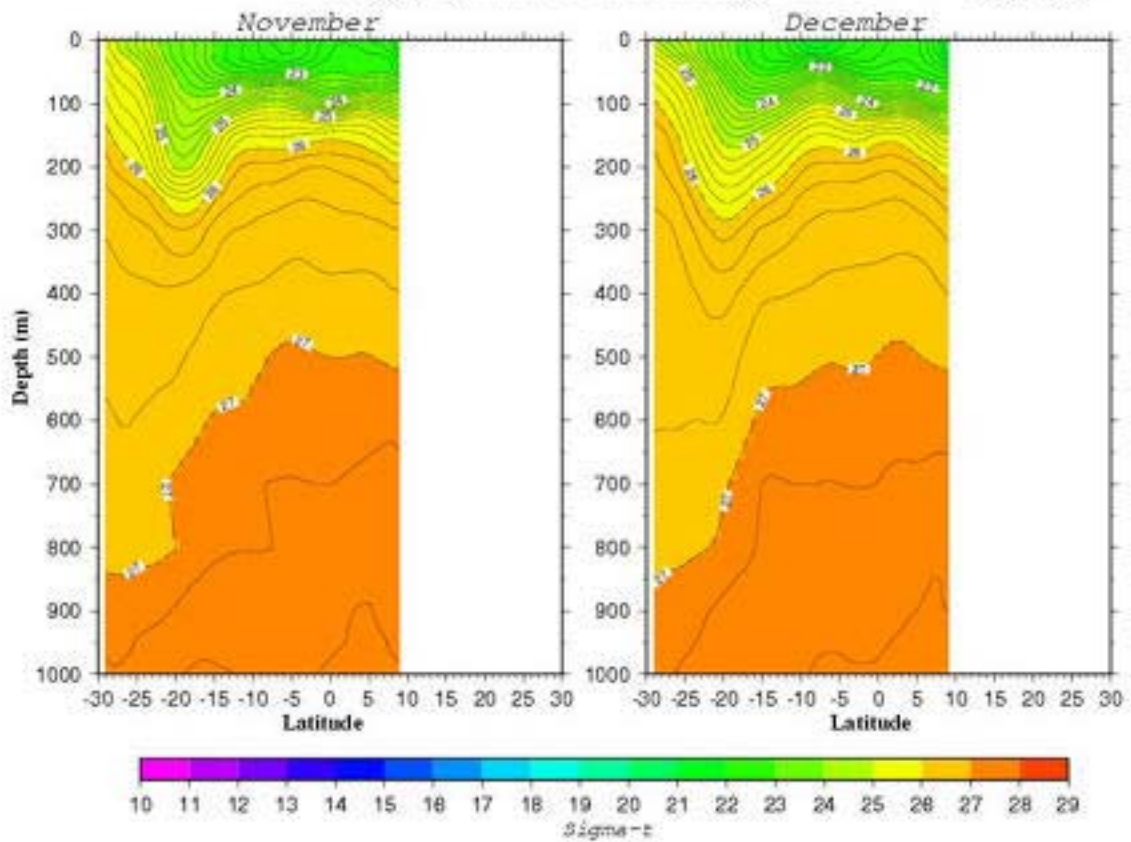
Density ( \sigma_t ) Section along 75.5°E
