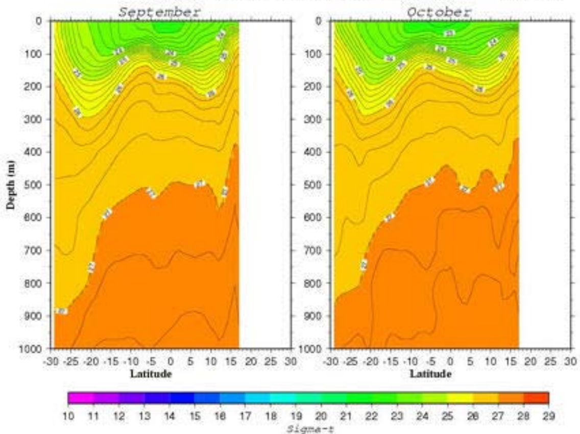
Density ( \sigma_t ) Section along 55.5°E
