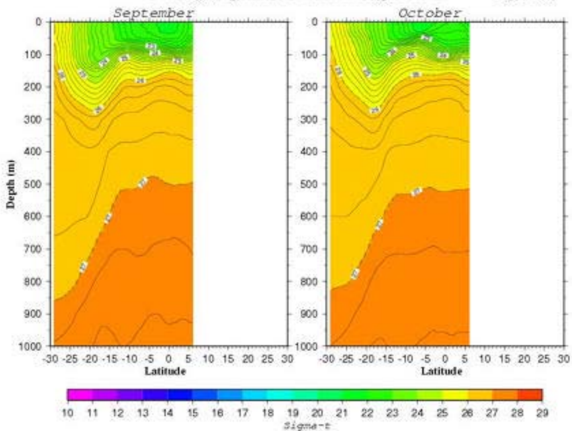
Density ( \sigma_t ) Section along 80.5°E
