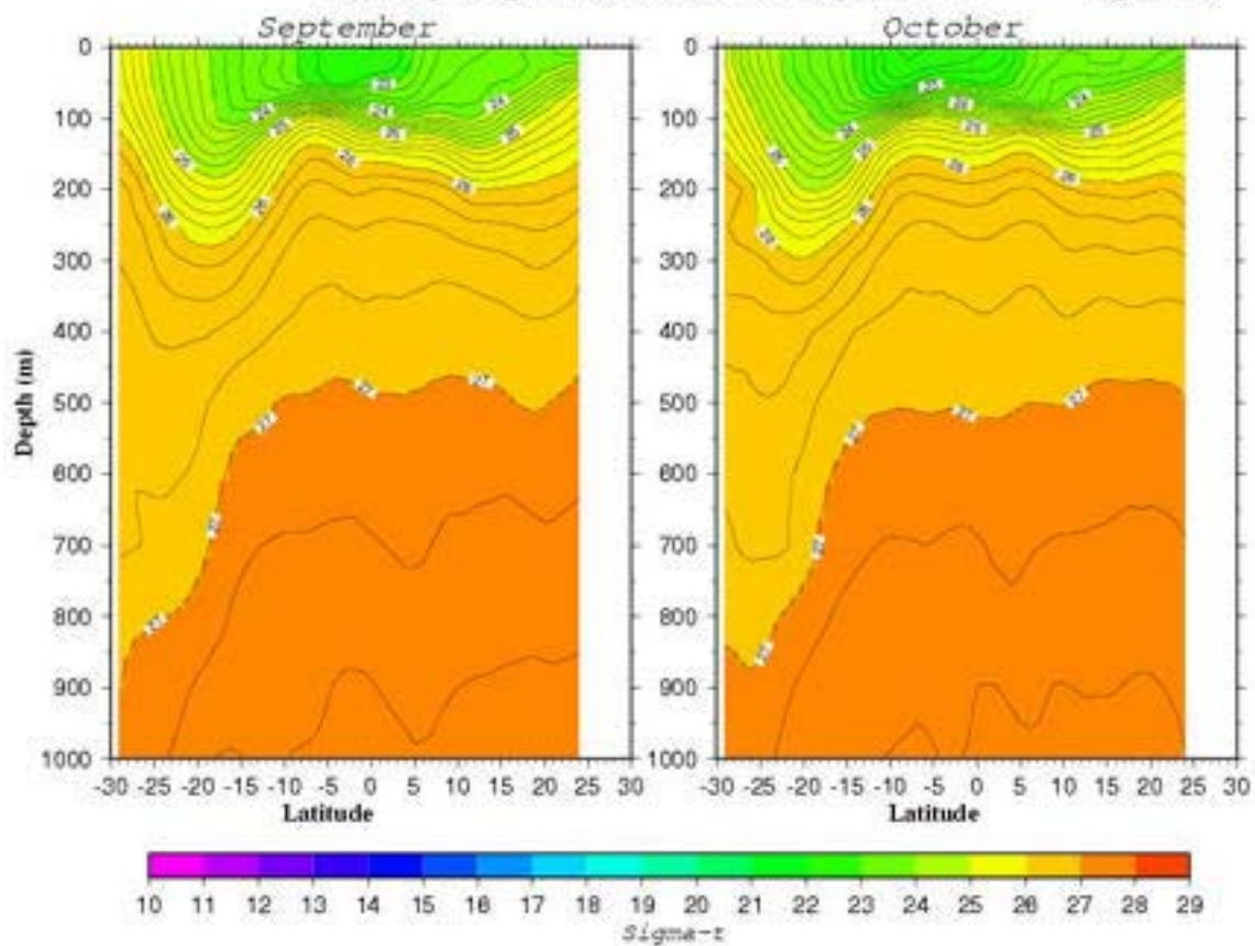
Density ( \sigma_t ) Section along 65.5°E
