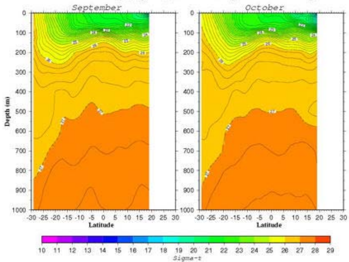
Density ( \sigma_t ) Section along 90.5°E
