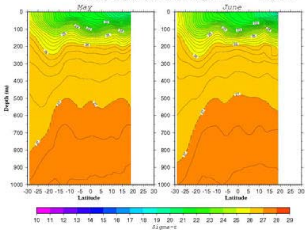
Density ( \sigma_t ) Section along 90.5°E
