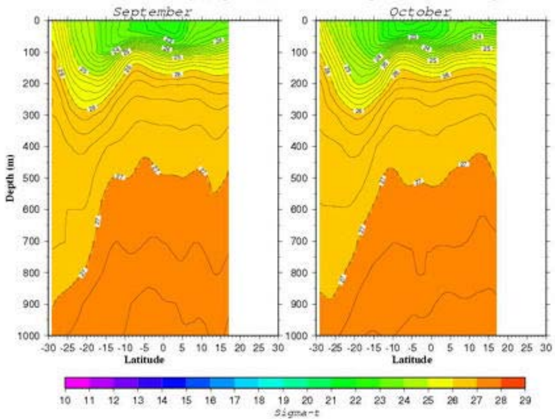
Density ( \sigma_t ) Section along 70.5°E
