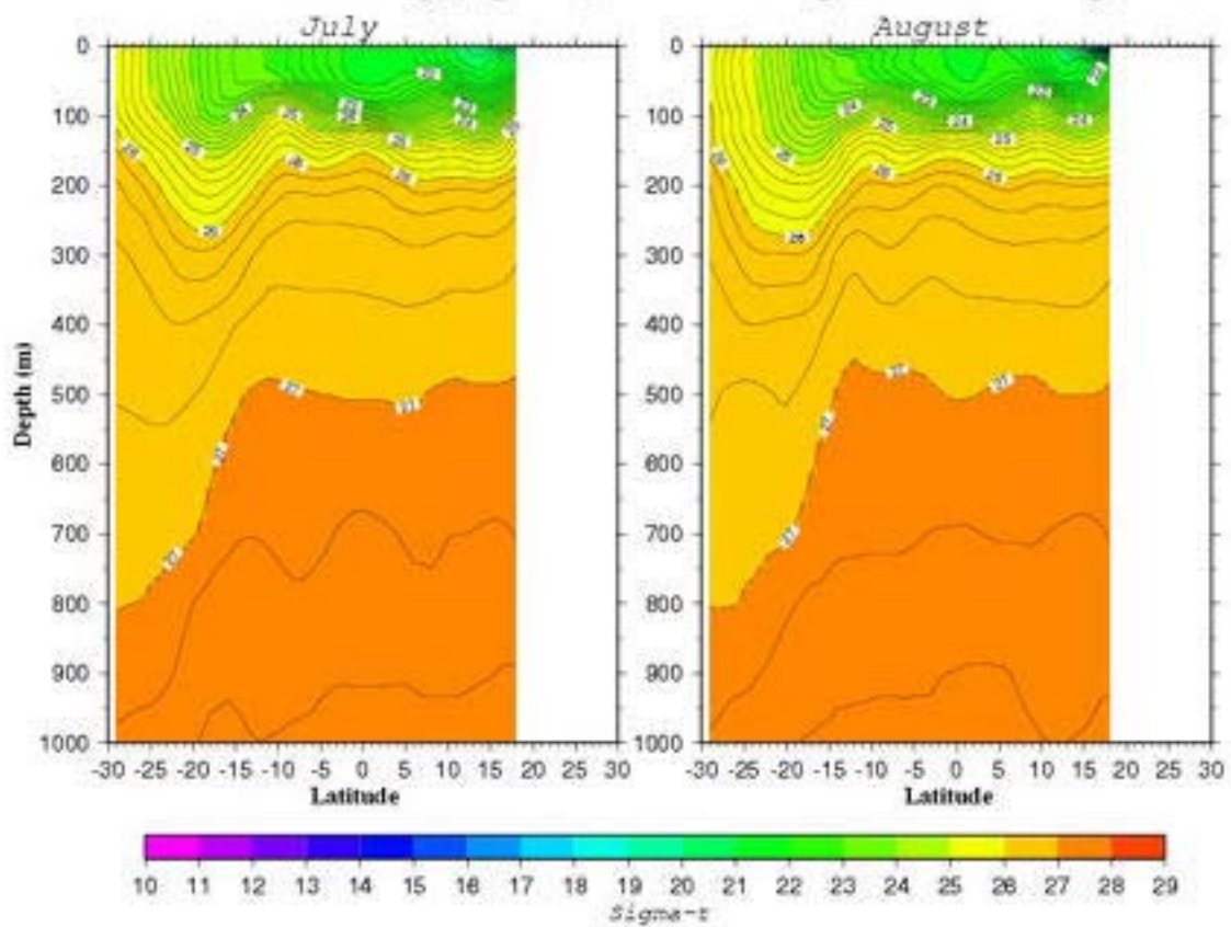
Density ( \sigma_t ) Section along 85.5°E
