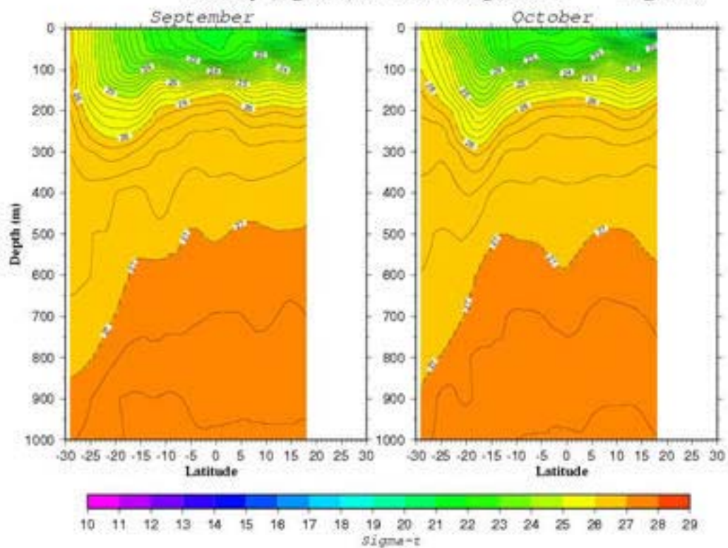
Density ( \sigma_t ) Section along 85.5°E
