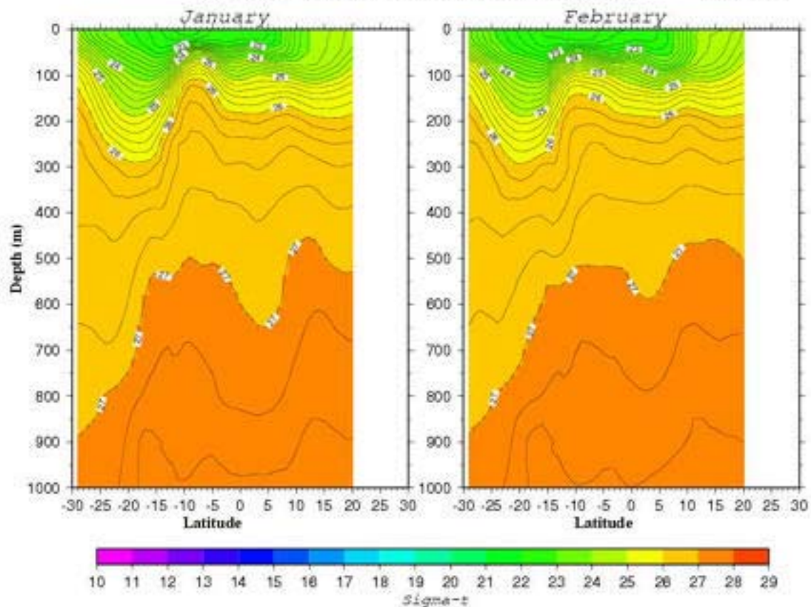
Density ( \sigma_t ) Section along 60.5°E
